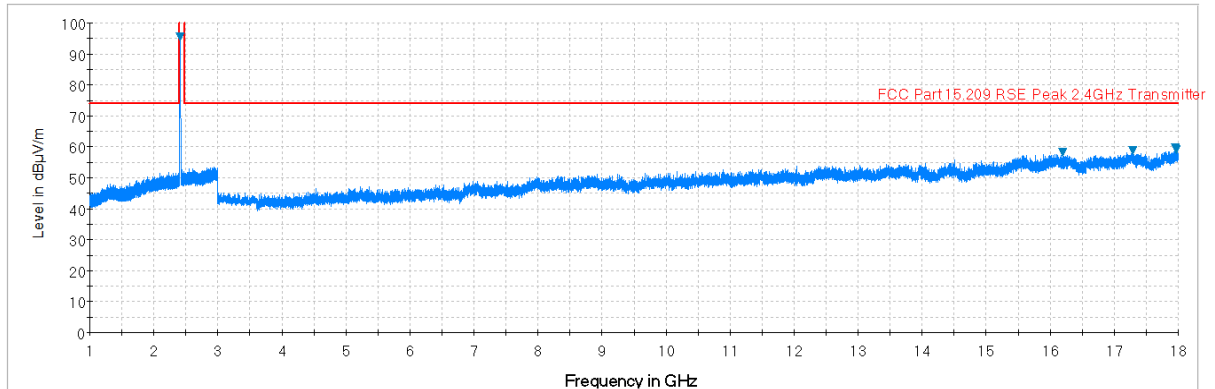
Plot 7-33. Radiated Spurious Plot above 1GHz (802.11b – Ch. 1, Ant. Pol. H)
