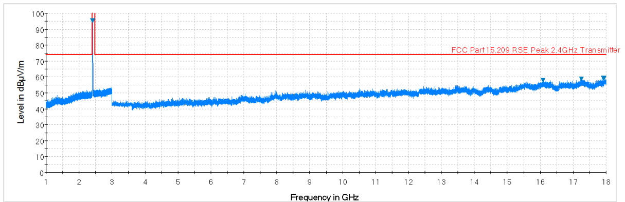
Plot 7-34. Radiated Spurious Plot above 1GHz (802.11b – Ch. 1, Ant. Pol. V)
