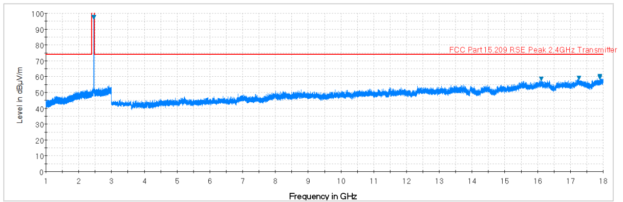
Plot 7-37. Radiated Spurious Plot above 1GHz (802.11b – Ch. 11, Ant. Pol. H)
