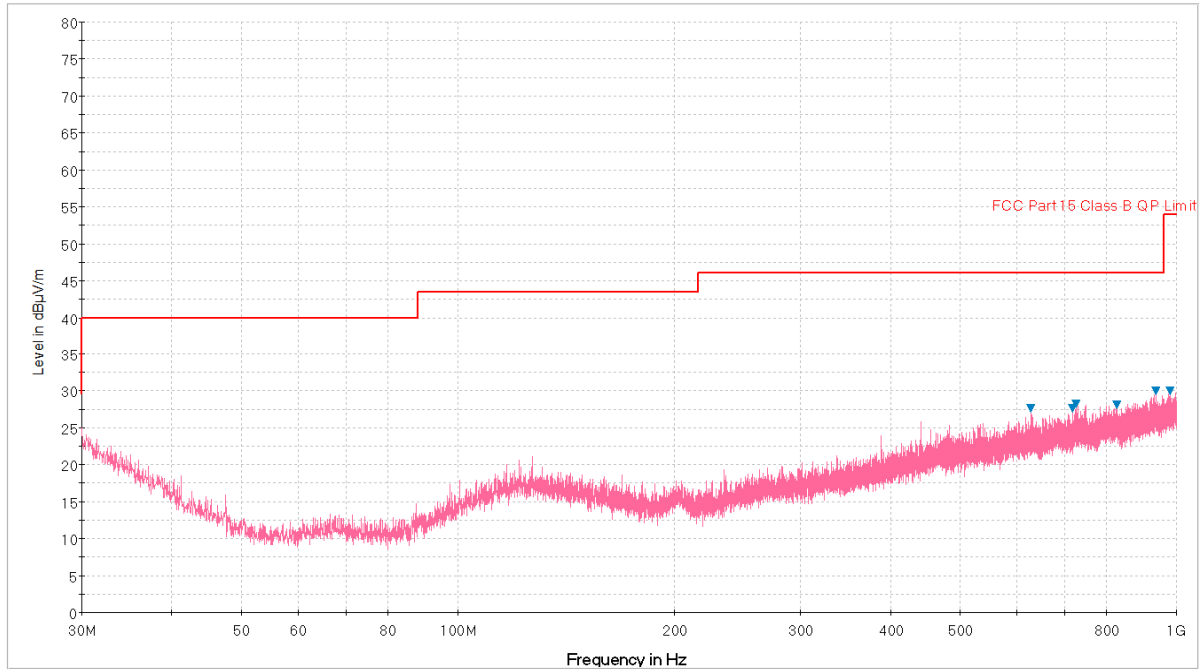
Plot 7-49. Radiated Spurious Plot below 1GHz (Pol. H)
