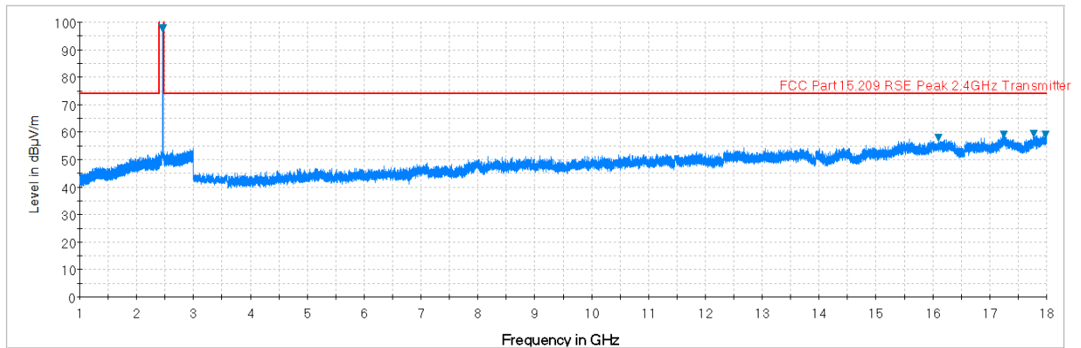
Plot 7-38. Radiated Spurious Plot above 1GHz (802.11b – Ch. 11, Ant. Pol. V)
