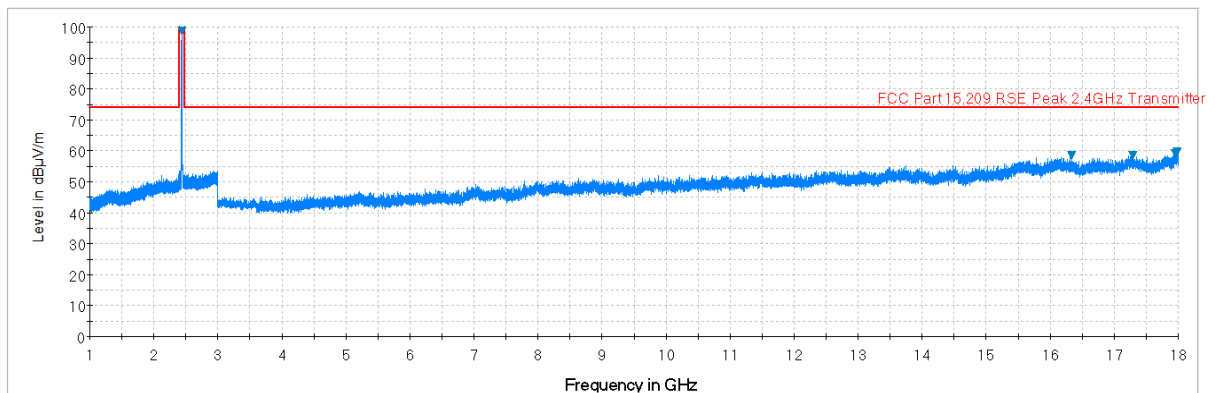
Plot 7-35. Radiated Spurious Plot above 1GHz (802.11b – Ch. 6, Ant. Pol. H)
