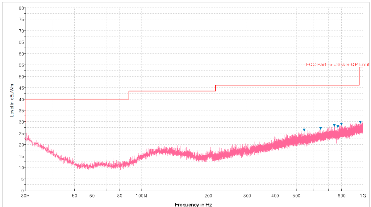
Plot 7-50. Radiated Spurious Plot below 1GHz (Pol. V)
