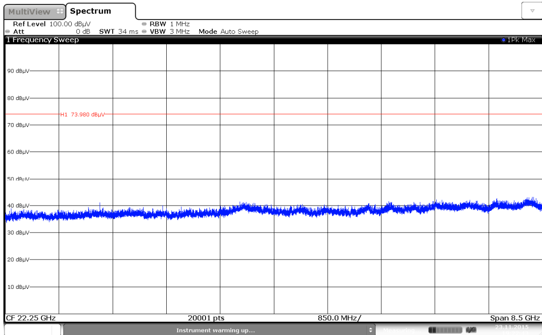
Plot 7-40. Radiated Spurious Plot above 18GHz (Pol. V)
