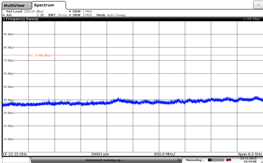
Plot 7-39. Radiated Spurious Plot above 18GHz (Pol. H)
