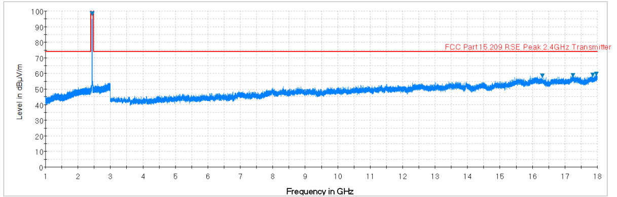
Plot 7-36. Radiated Spurious Plot above 1GHz (802.11b – Ch. 6, Ant. Pol. V)
