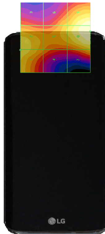
Figure 18-4 E-Field WD Scan overlay
