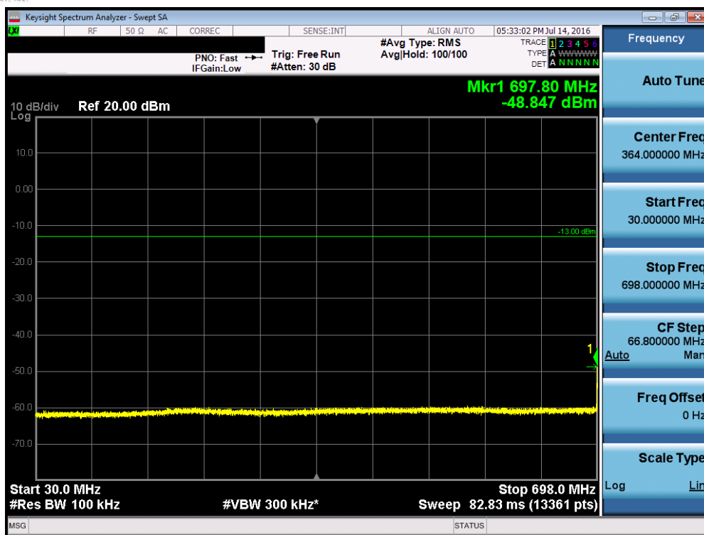
Plot 7-57. Conducted Spurious Plot (Band 12 – 10.0MHz QPSK – RB Size 1, RB Offset 0 – High Channel)
