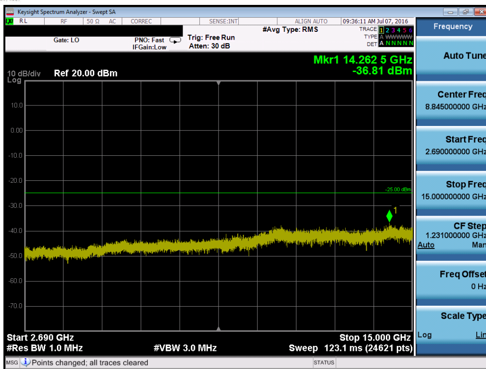
Plot 7-91. Conducted Spurious Plot (Band 41 – 5.0MHz QPSK – RB Size 1, RB Offset 0 – Mid Channel)
