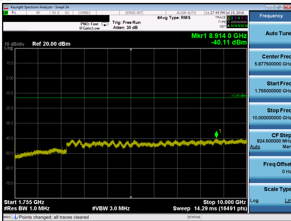
Plot 7-73. Conducted Spurious Plot (Band 4 – 20.0MHz QPSK – RB Size 1, RB Offset 0 – Mid Channel)
