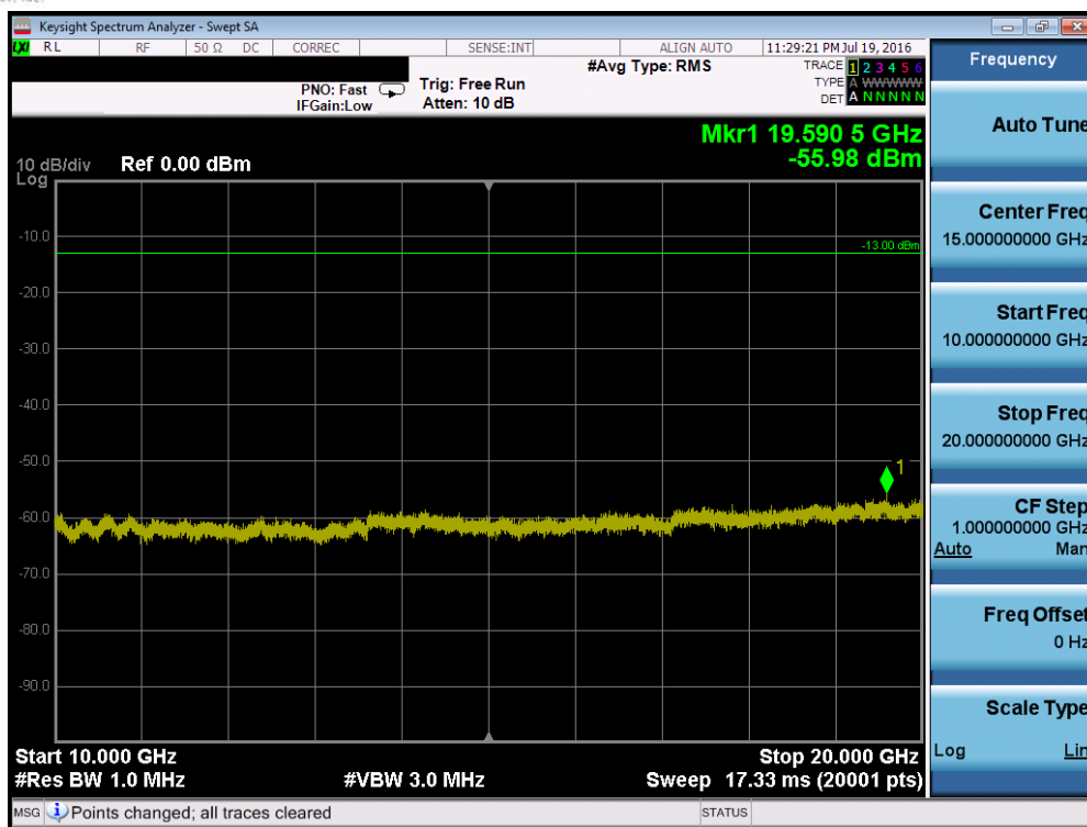
Plot 7-71. Conducted Spurious Plot (Band 4 – 20.0MHz QPSK – RB Size 1, RB Offset 0 – Low Channel)
