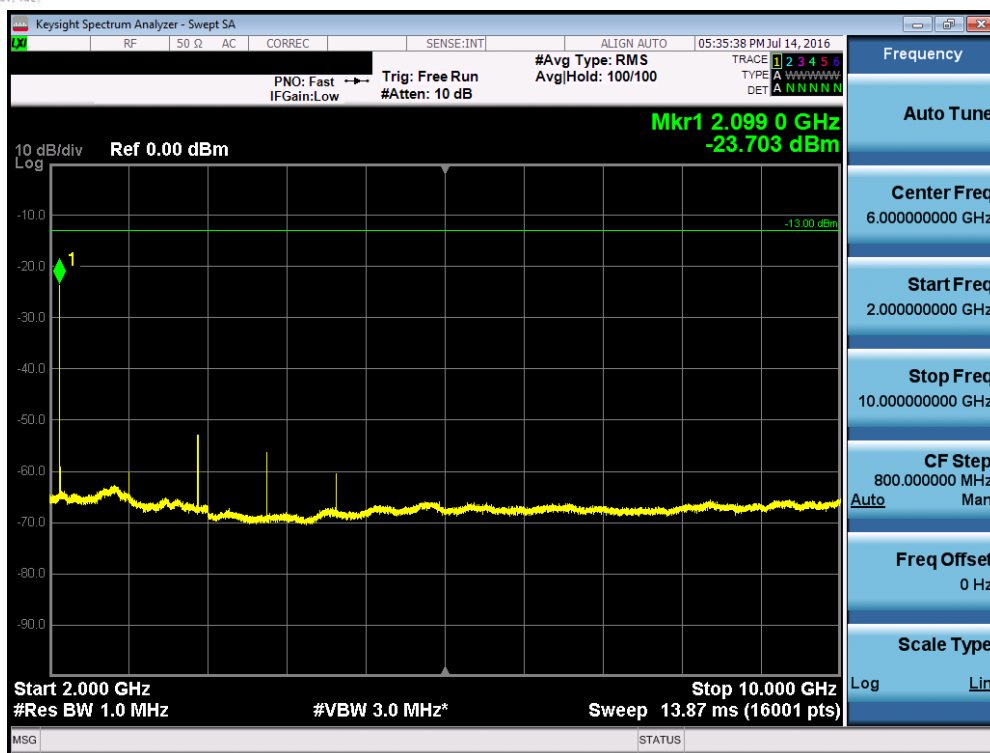
Plot 7-53. Conducted Spurious Plot (Band 12 – 10.0MHz QPSK – RB Size 1, RB Offset 0 – Low Channel)
