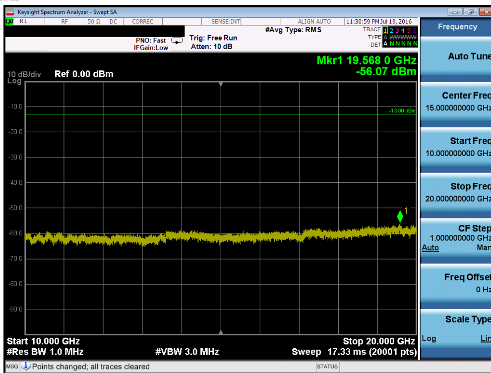
Plot 7-77. Conducted Spurious Plot (Band 4 – 20.0MHz QPSK – RB Size 1, RB Offset 0 – High Channel)
