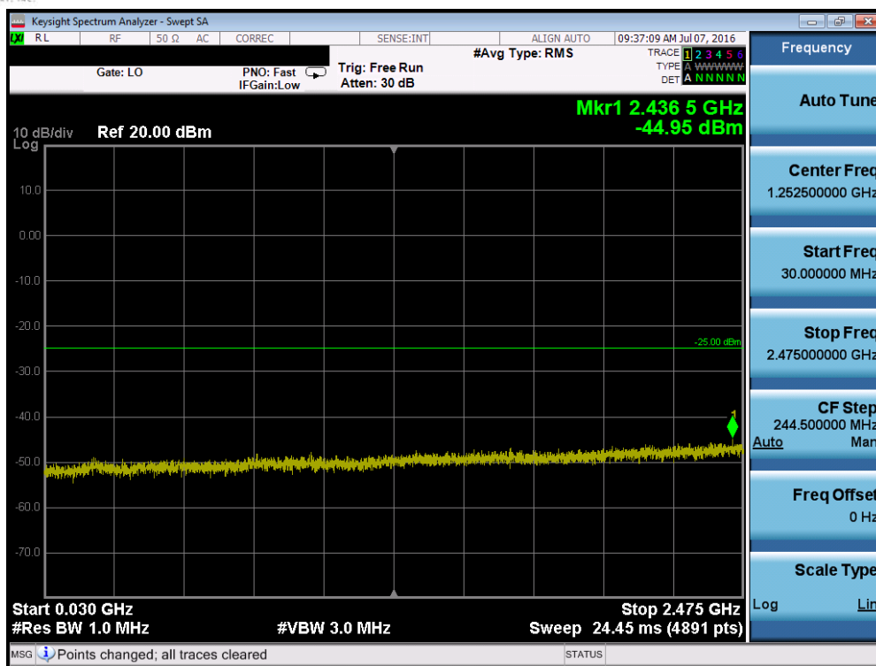
Plot 7-87. Conducted Spurious Plot (Band 41 – 5.0MHz QPSK – RB Size 1, RB Offset 0 – Low Channel)
