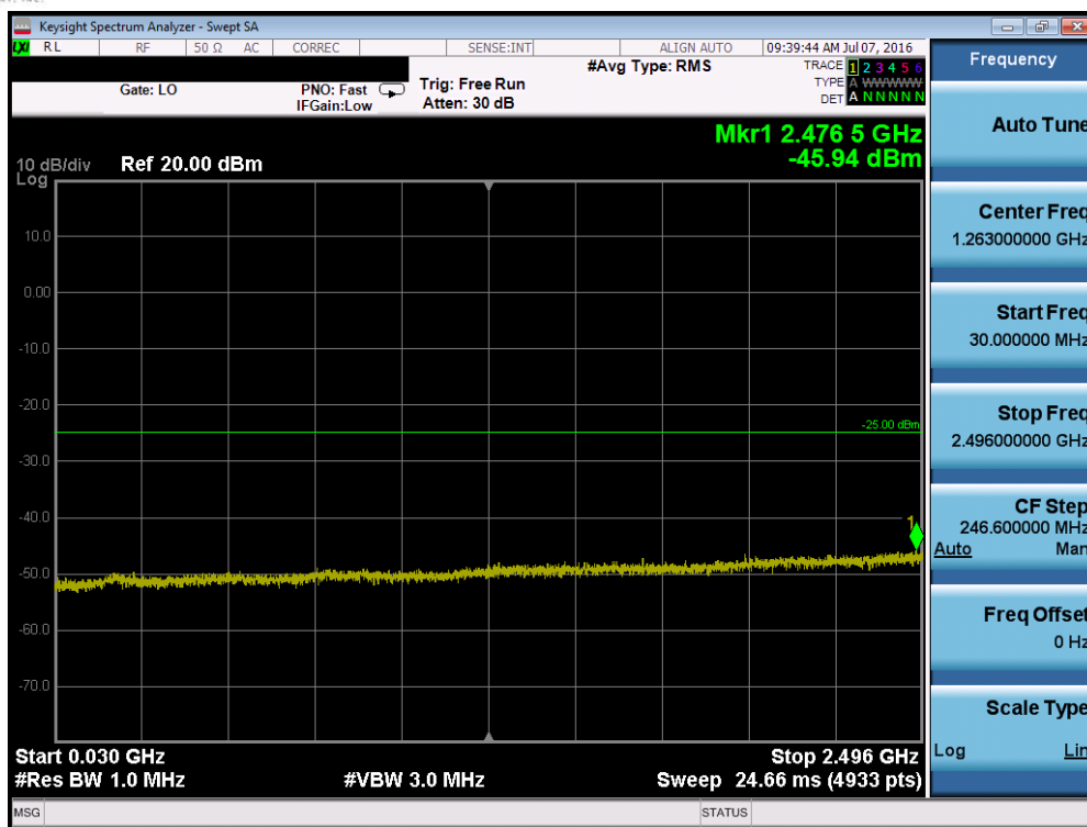
Plot 7-93. Conducted Spurious Plot (Band 41 – 5.0MHz QPSK – RB Size 1, RB Offset 0 – High Channel)
