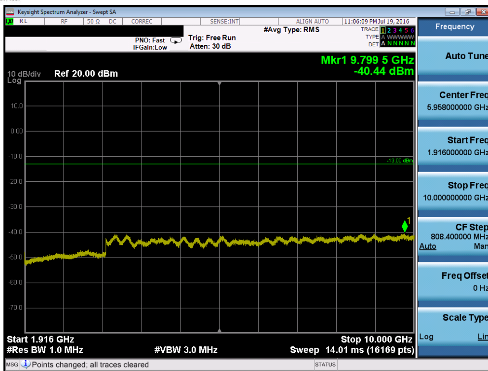
Plot 7-85. Conducted Spurious Plot (Band 2/25 – 20.0MHz QPSK – RB Size 1, RB Offset 0 – High Channel)
