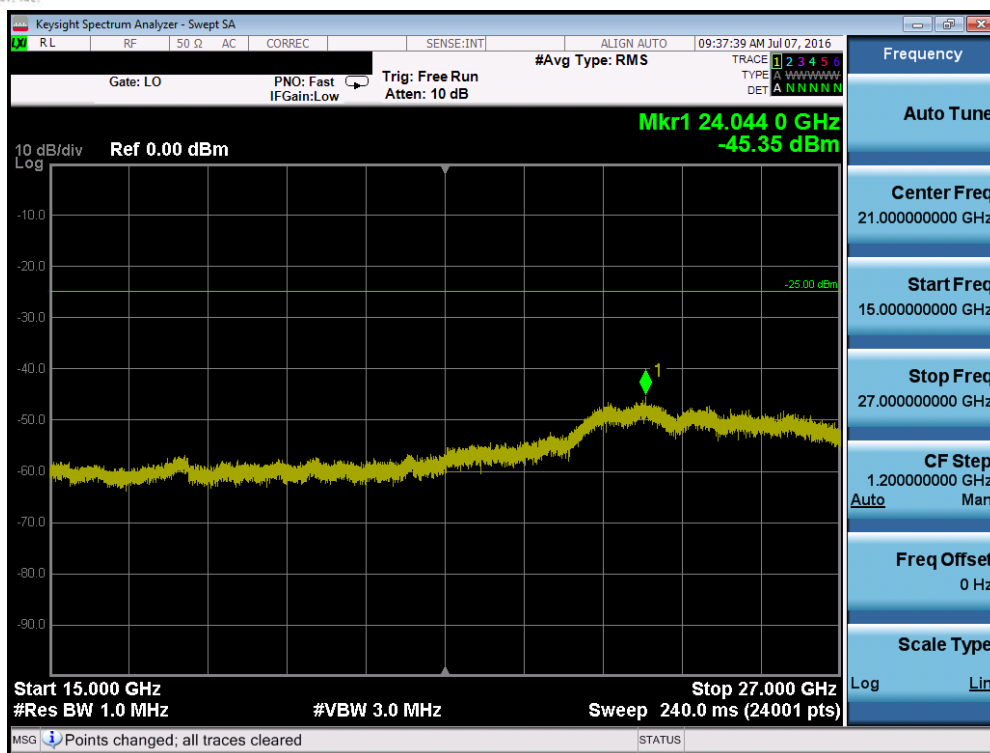
Plot 7-89. Conducted Spurious Plot (Band 41 – 5.0MHz QPSK – RB Size 1, RB Offset 0 – Low Channel)
