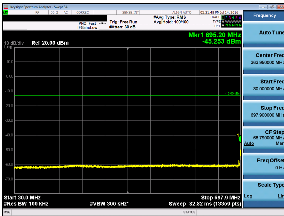
Plot 7-51. Conducted Spurious Plot (Band 12 – 10.0MHz QPSK – RB Size 1, RB Offset 0– Low Channel)
