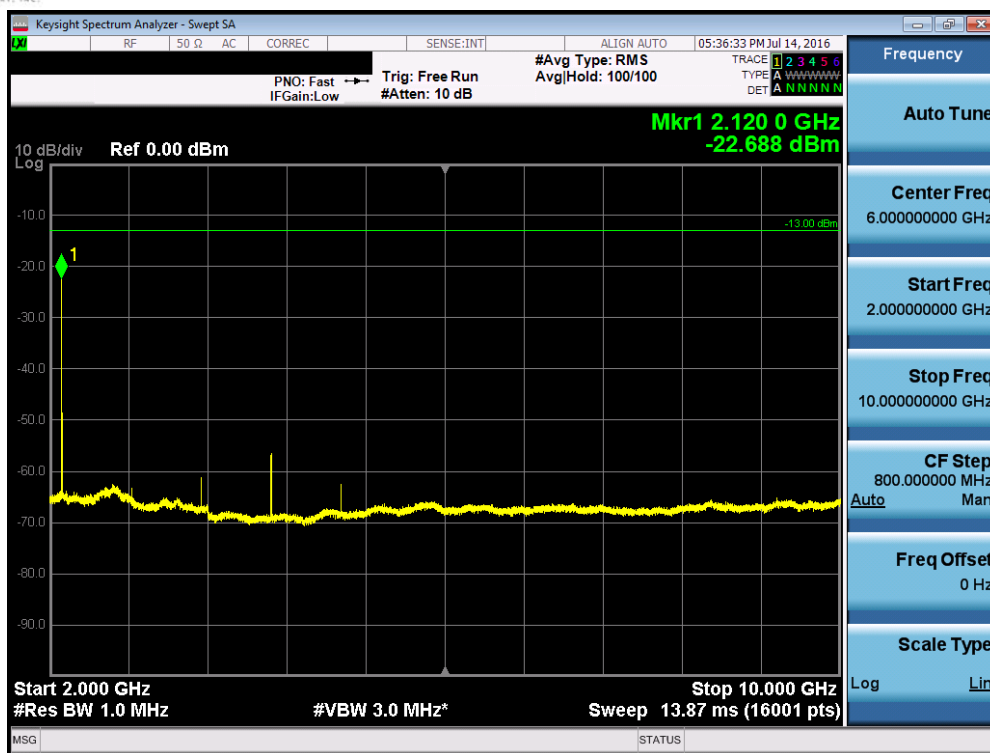
Plot 7-59. Conducted Spurious Plot (Band 12 – 10.0MHz QPSK – RB Size 1, RB Offset 0 – High Channel)
