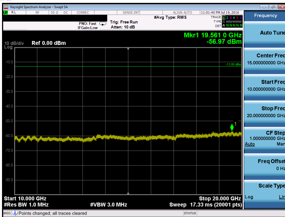
Plot 7-83. Conducted Spurious Plot (Band 2/25 – 20.0MHz QPSK – RB Size 1, RB Offset 0 – Mid Channel)
