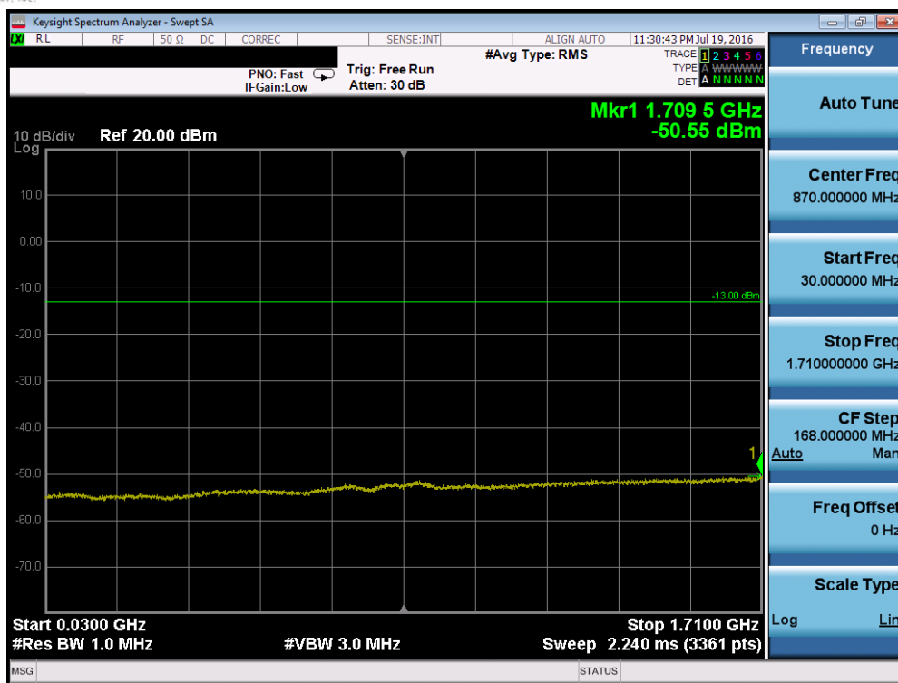
Plot 7-75. Conducted Spurious Plot (Band 4 – 20.0MHz QPSK – RB Size 1, RB Offset 0 – High Channel)
