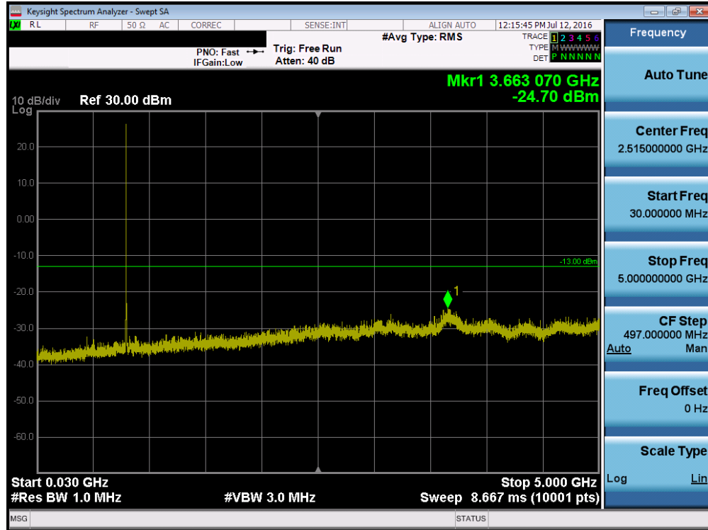
Plot 7-13. Conducted Spurious Plot (CDMA B10, Ch. 476)
