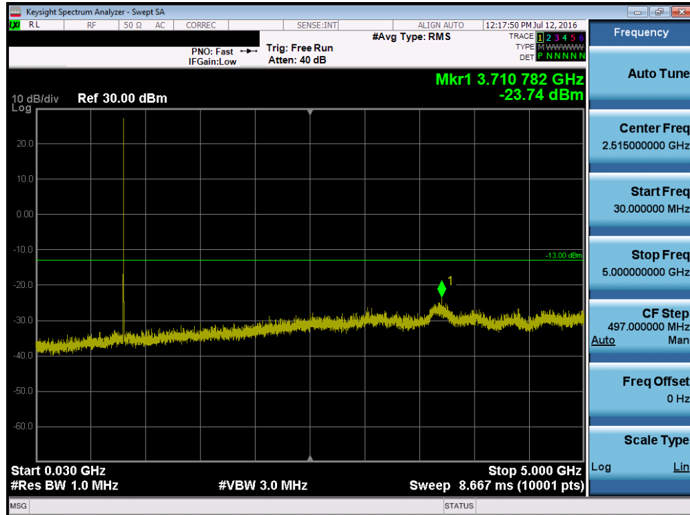
Plot 7-15. Conducted Spurious Plot (CDMA B10, Ch. 684)
