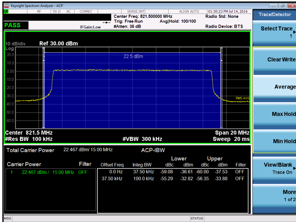
Plot 7-30. Channel Edge Plot (LTE Band 26, 15MHz QPSK – RB Size 75)
