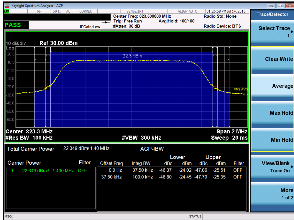
Plot 7-24. Channel Edge Plot (LTE Band 26, 1.4MHz QPSK – RB Size 6 – High Channel)
