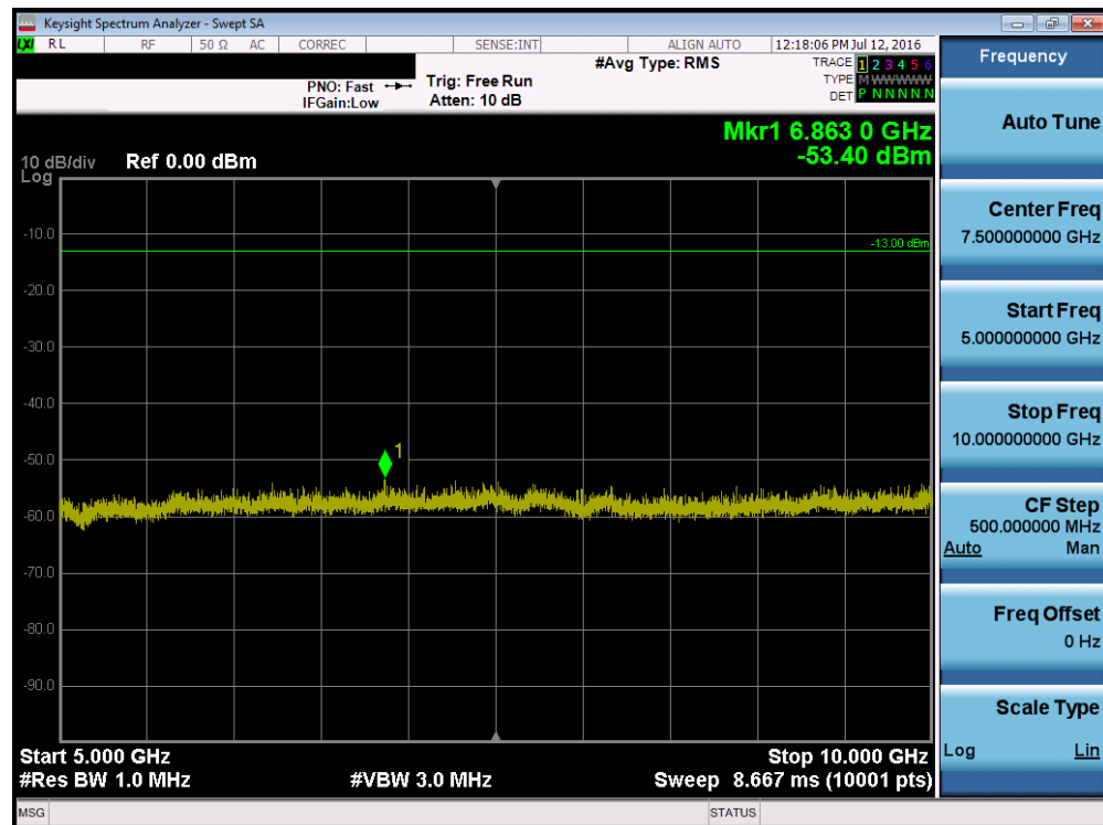
Plot 7-16. Conducted Spurious Plot (CDMA B10, Ch. 684)
