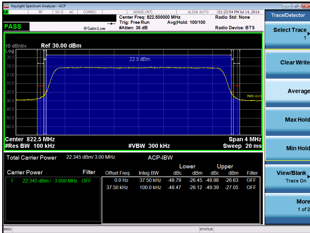
Plot 7-26. Channel Edge Plot (LTE Band 26, 3MHz QPSK – RB Size 15 – High Channel)
