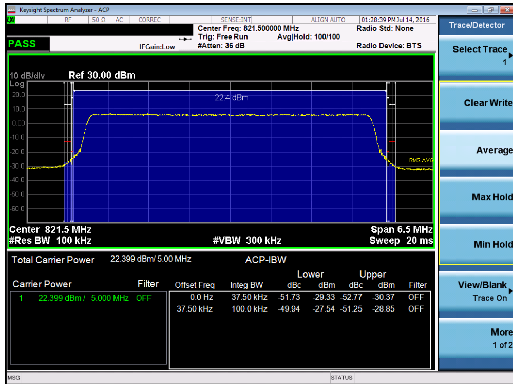
Plot 7-28. Channel Edge Plot (LTE Band 26, 5MHz QPSK – RB Size 25 – High Channel)
