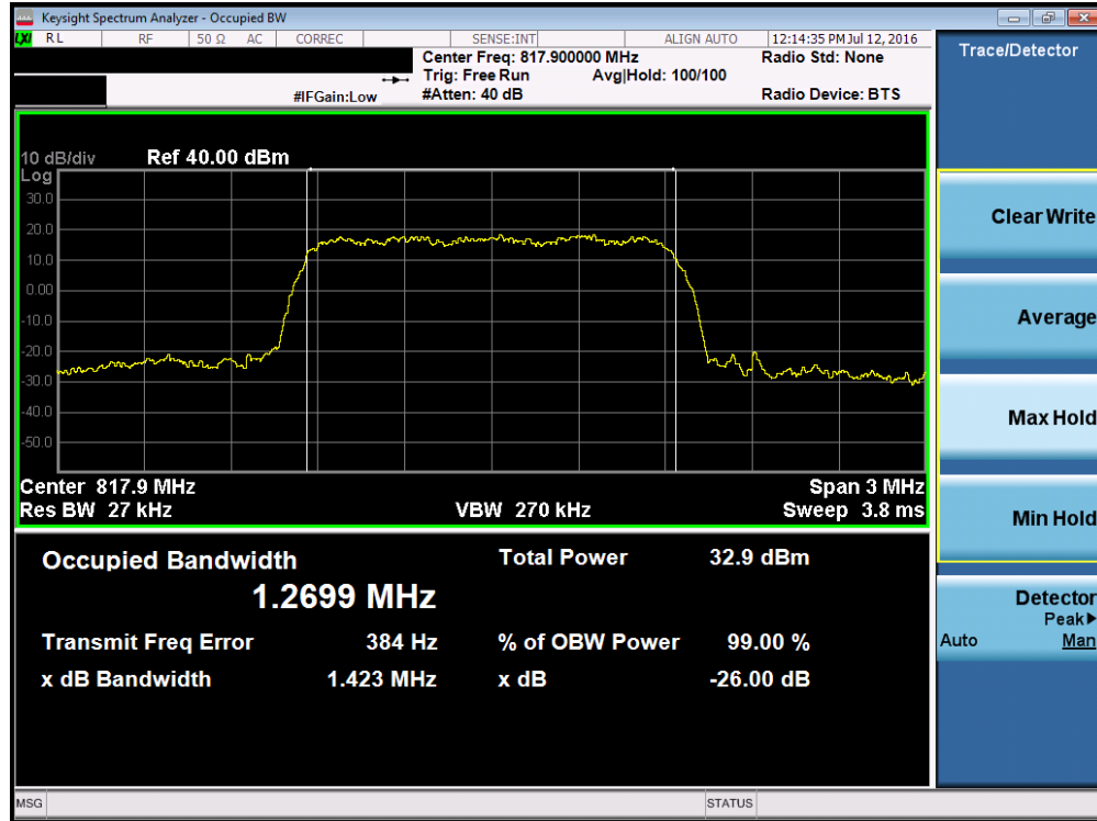
Plot 7-1. Occupied Bandwidth Plot (CDMA B10, Ch. 476)
