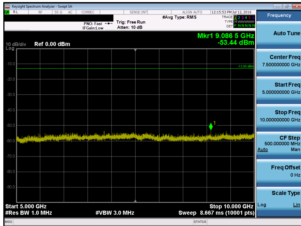
Plot 7-14. Conducted Spurious Plot (CDMA B10, Ch. 476)
