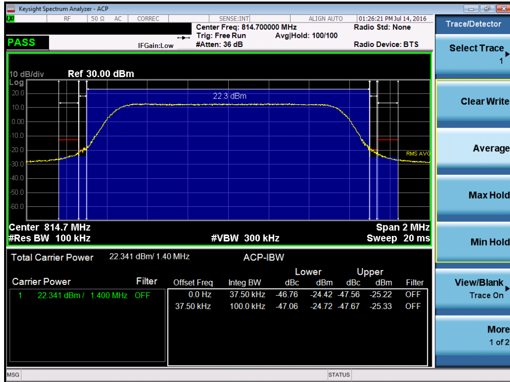
Plot 7-23. Channel Edge Plot (LTE Band 26, 1.4MHz QPSK – RB Size 6– Low Channel)
