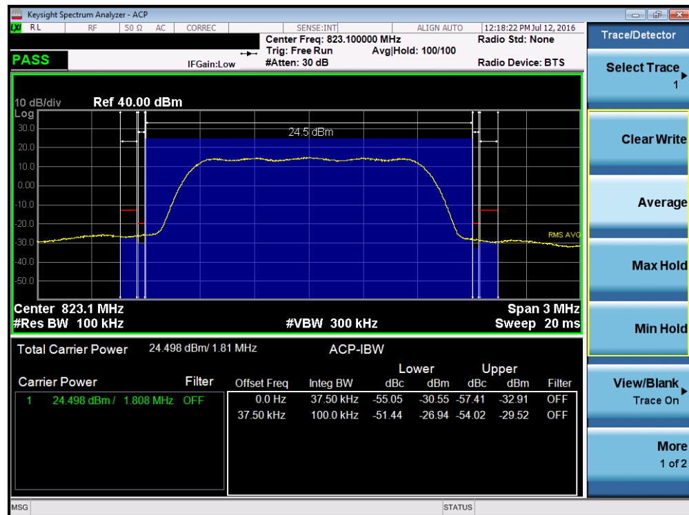
Plot 7-22. Channel Edge Plot (CDMA B10, Ch. 684)
