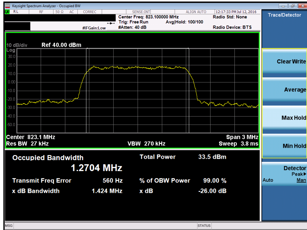
Plot 7-2. Occupied Bandwidth Plot (CDMA B10, Ch. 684)
