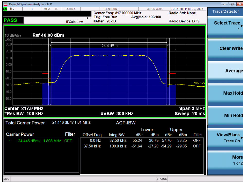
Plot 7-21. Channel Edge Plot (CDMA B10, Ch. 476)
