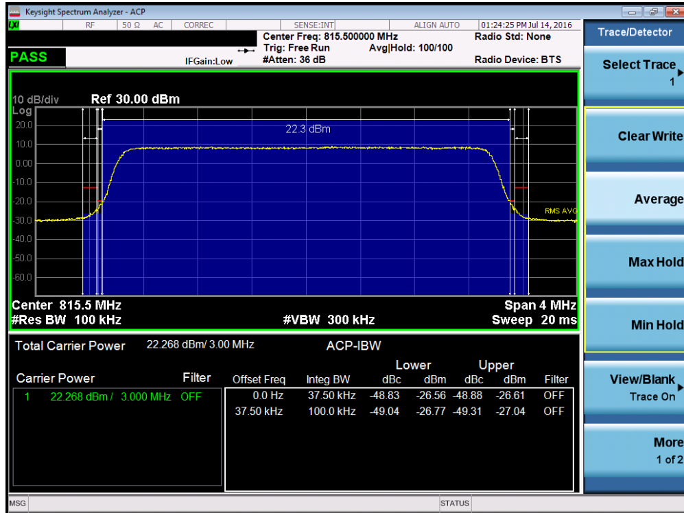
Plot 7-25. Channel Edge Plot (LTE Band 26, 3MHz QPSK – RB Size 15– Low Channel)
