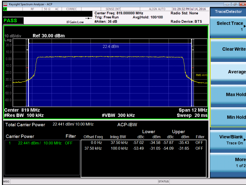
Plot 7-29. Channel Edge Plot (LTE Band 26, 10MHz QPSK – RB Size 50)
