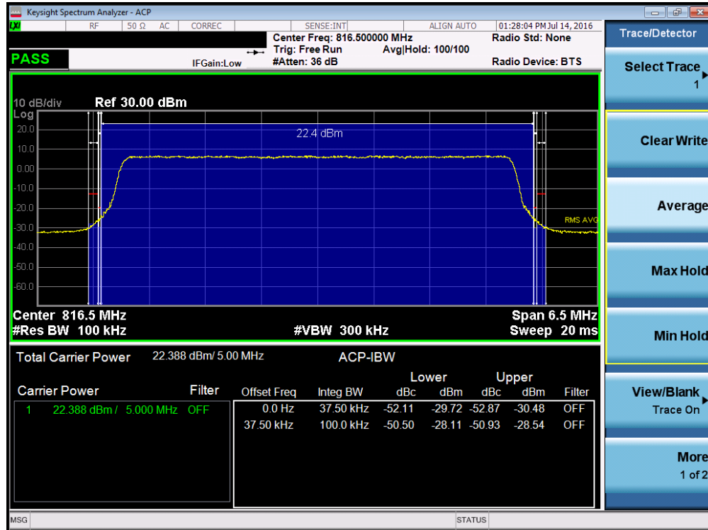
Plot 7-27. Channel Edge Plot (LTE Band 26, 5MHz QPSK – RB Size 25– Low Channel)
