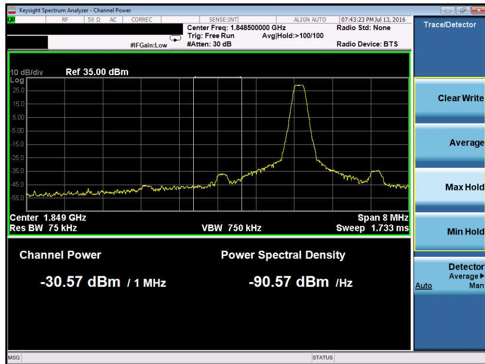
Plot 7-76. Extended Band Edge Plot (PCS GPRS Mode – Ch. 512)
