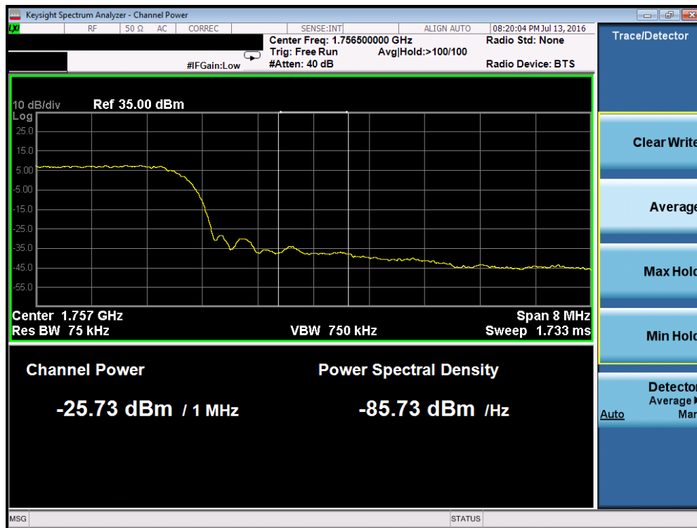
Plot 7-92. Band Edge Plot (AWS WCDMA Mode – Ch. 1513)
