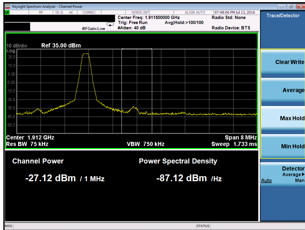
Plot 7-78. Extended Band Edge Plot (PCS GPRS Mode – Ch. 810)
