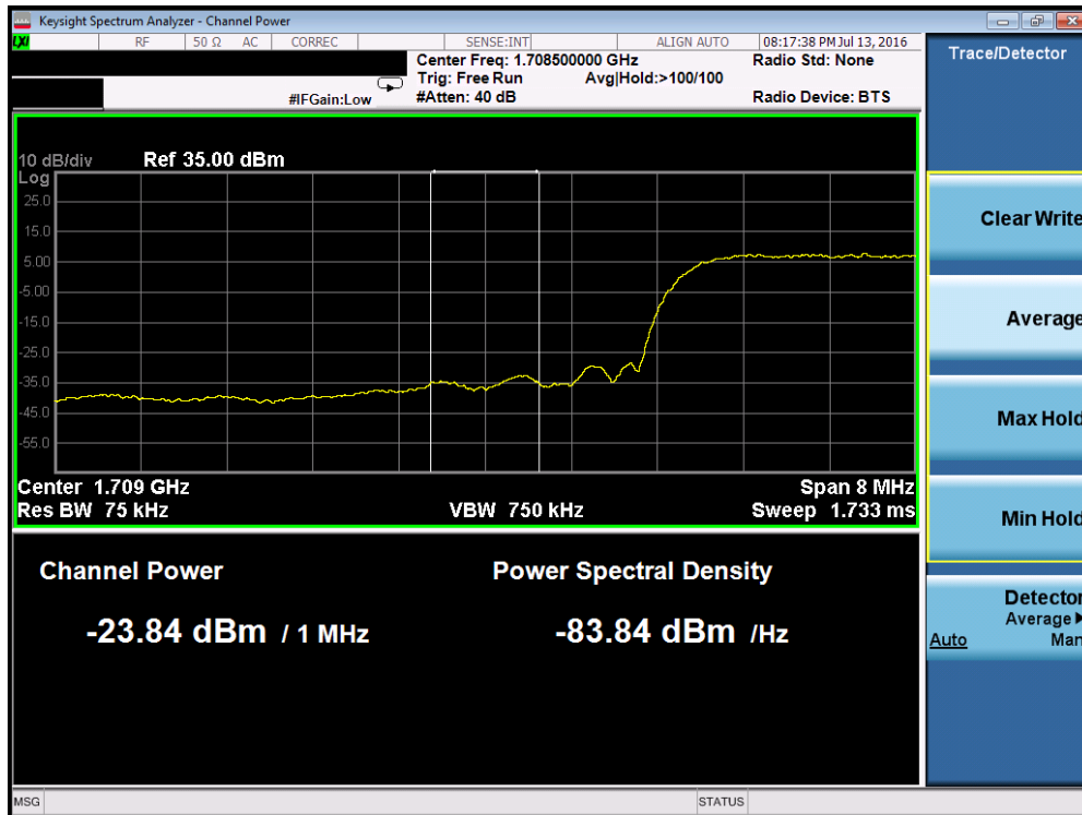
Plot 7-90. Extended Band Edge Plot (AWS WCDMA Mode – Ch. 1312)
