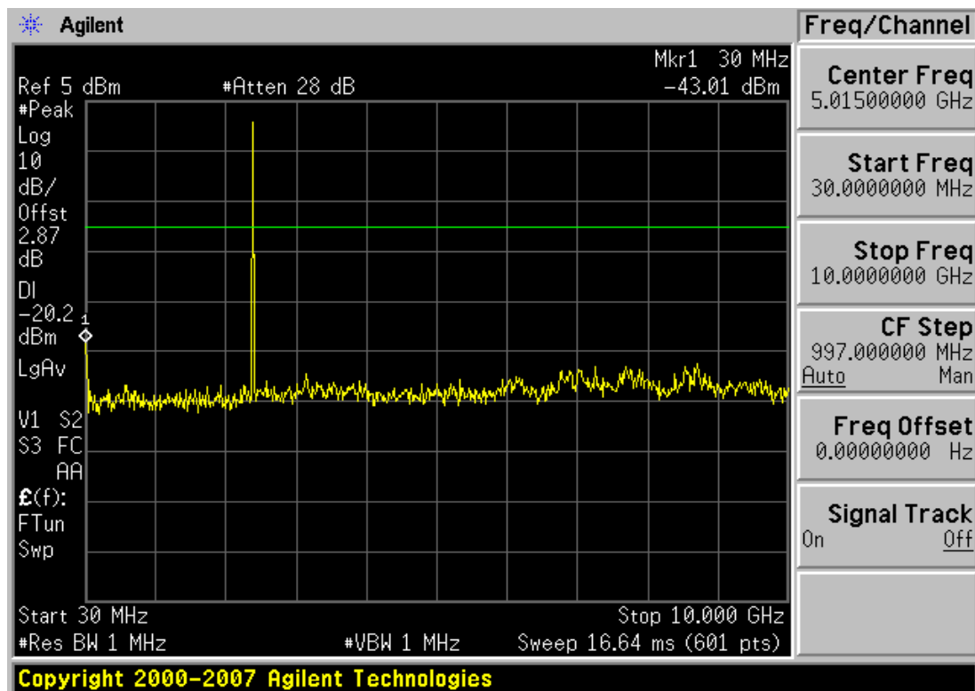
Plot 6-16. Conducted Spurious Plot (Bluetooth, 2Mbps – Ch. 0)
