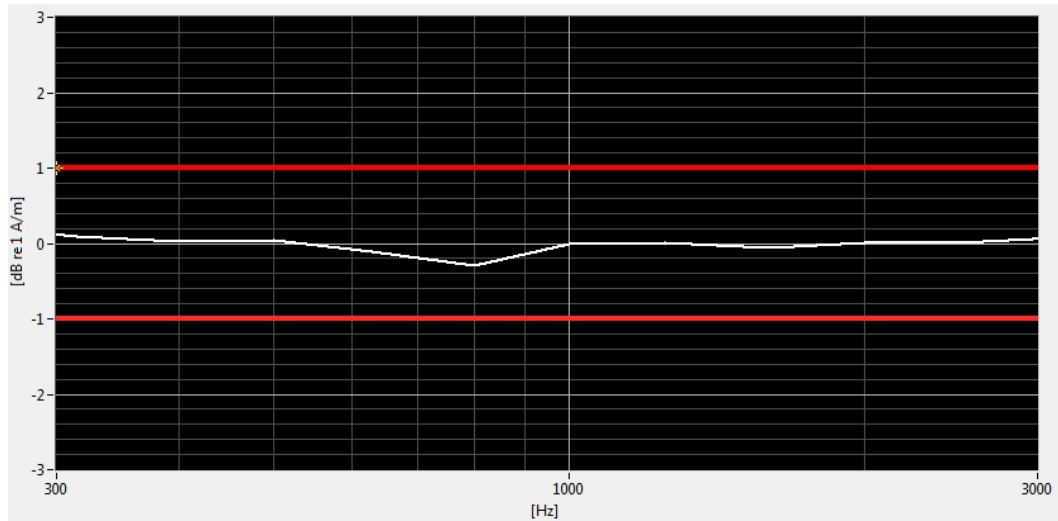
Figure 6-3 Helmholtz Coil Validation for Frequency Response
