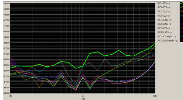
Figure 7-1 CDMA Audio Band Magnetic Noise
