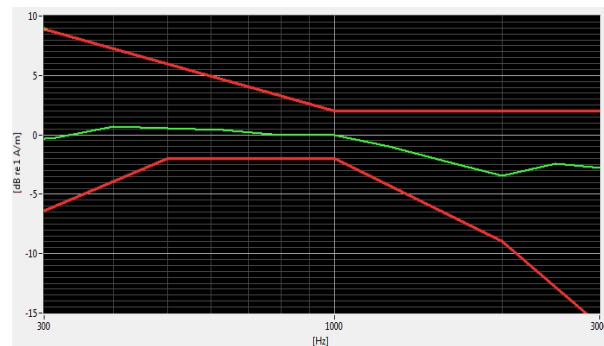
Figure 6-1 Axial Frequency Response
