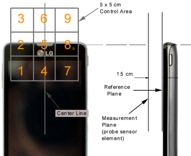
Figure 18-3: 5cm x 5cm Scan grid above WD
