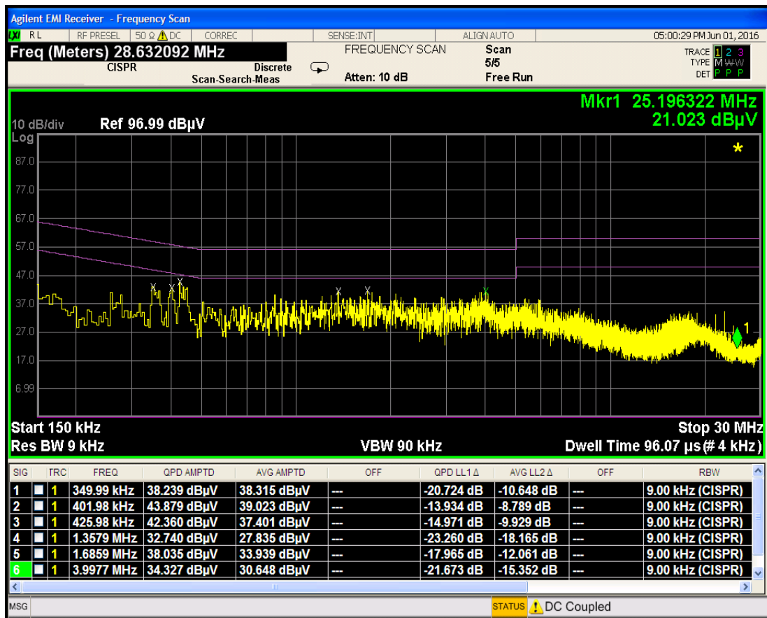
Plot 7-20. Line Conducted Plot with Bluetooth LE (L1)
