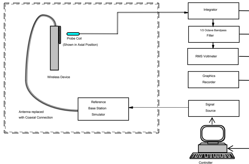
Figure 4-14 Audio Magnetic Field Test Setup
