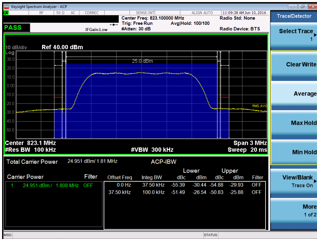
Plot 7-22. Extended Band Edge Plot (CDMA Ch. 684)
