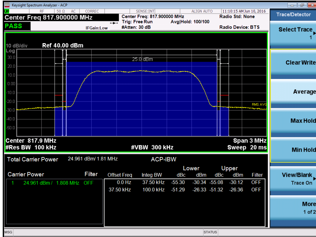
Plot 7-21. Extended Band Edge Plot (CDMA Ch. 476)
