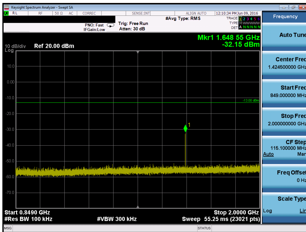
Plot 7-11. Conducted Spurious Plot (Cellular GSM Mode – Ch. 128)
