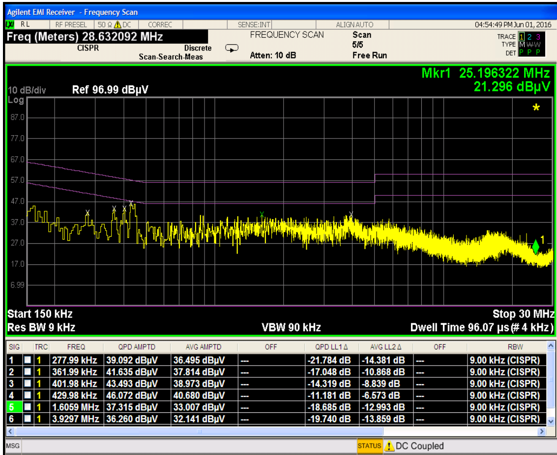
Plot 7-54. Line-Conducted Test Plot (L1)
