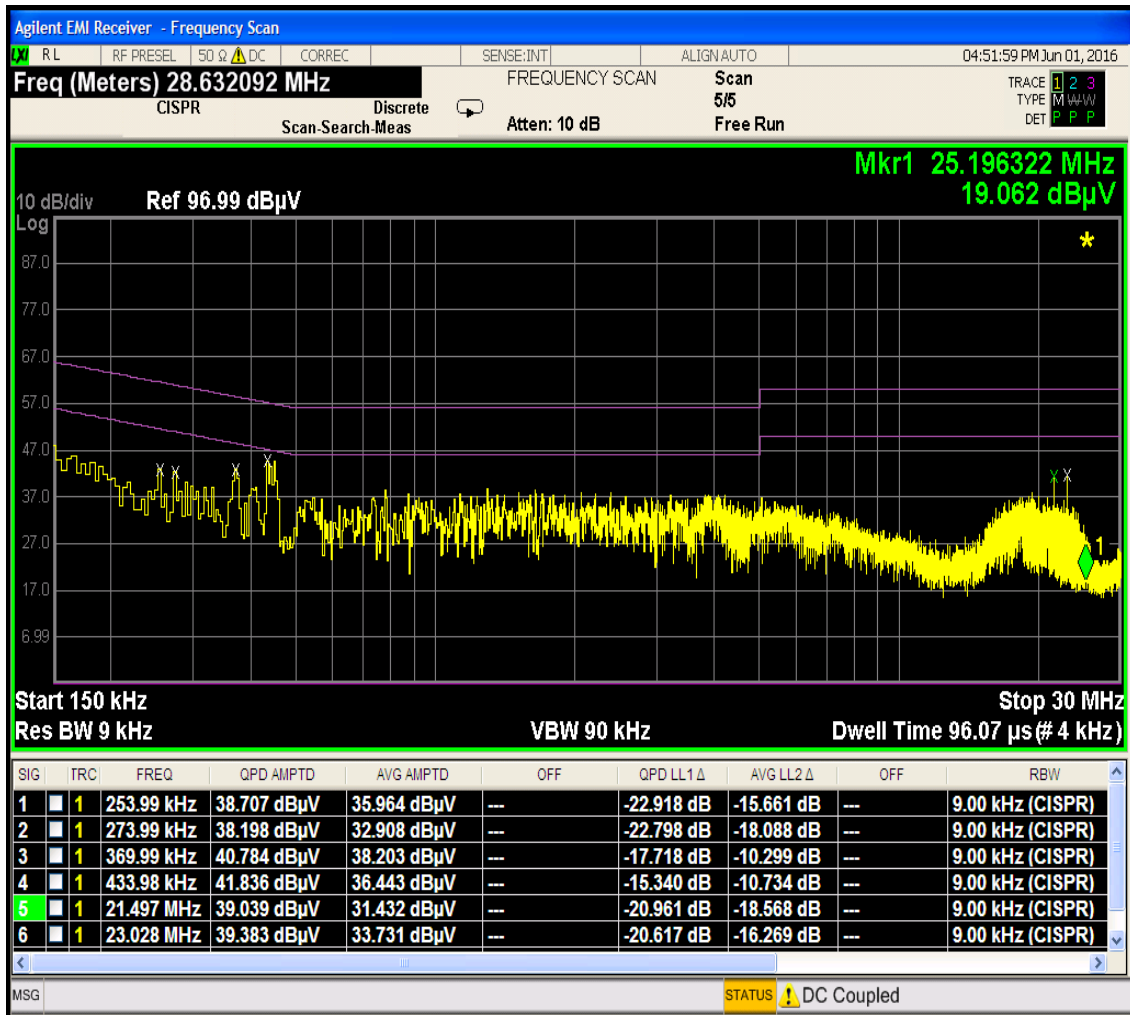
Plot 7-55. Line-Conducted Test Plot (N)
