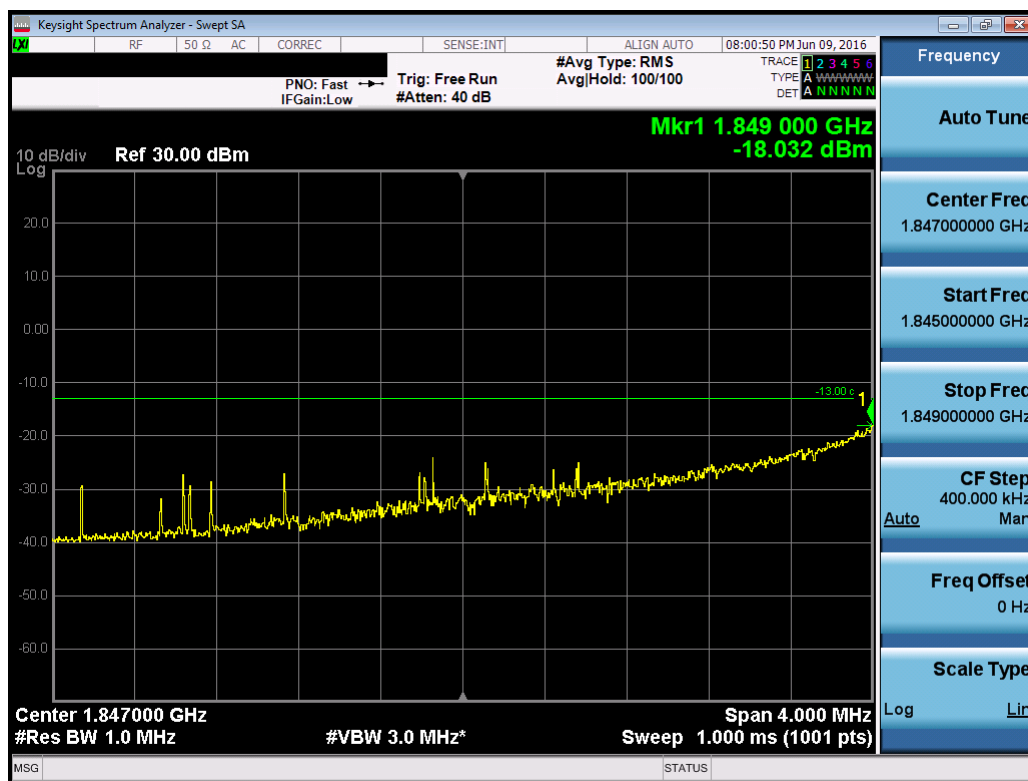
Plot 7-84. 4MHz Span Plot (PCS CDMA Mode – Ch. 25)
