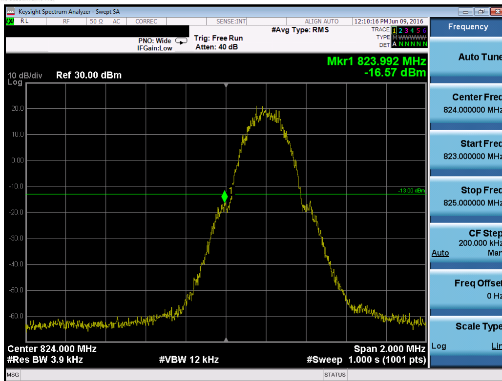
Plot 7-73. Band Edge Plot (Cellular GSM Mode – Ch. 128)
