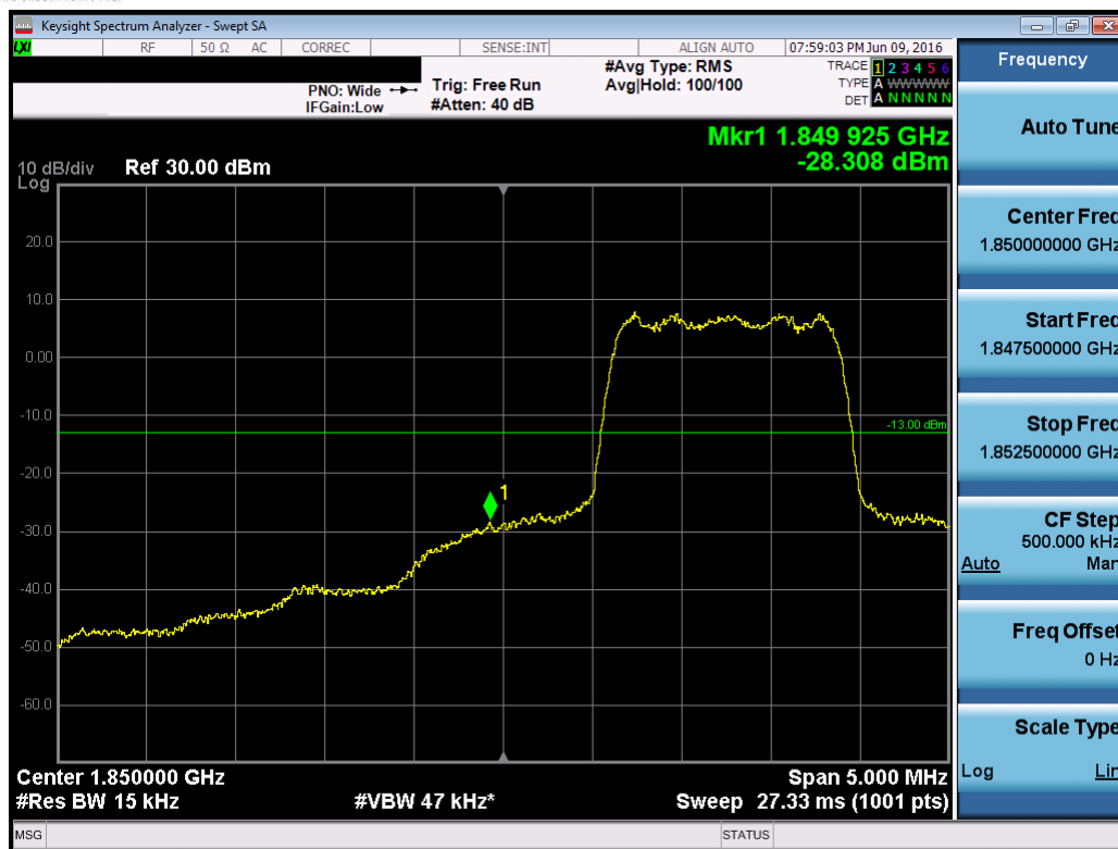
Plot 7-83. Band Edge Plot (PCS CDMA Mode – Ch. 25)
