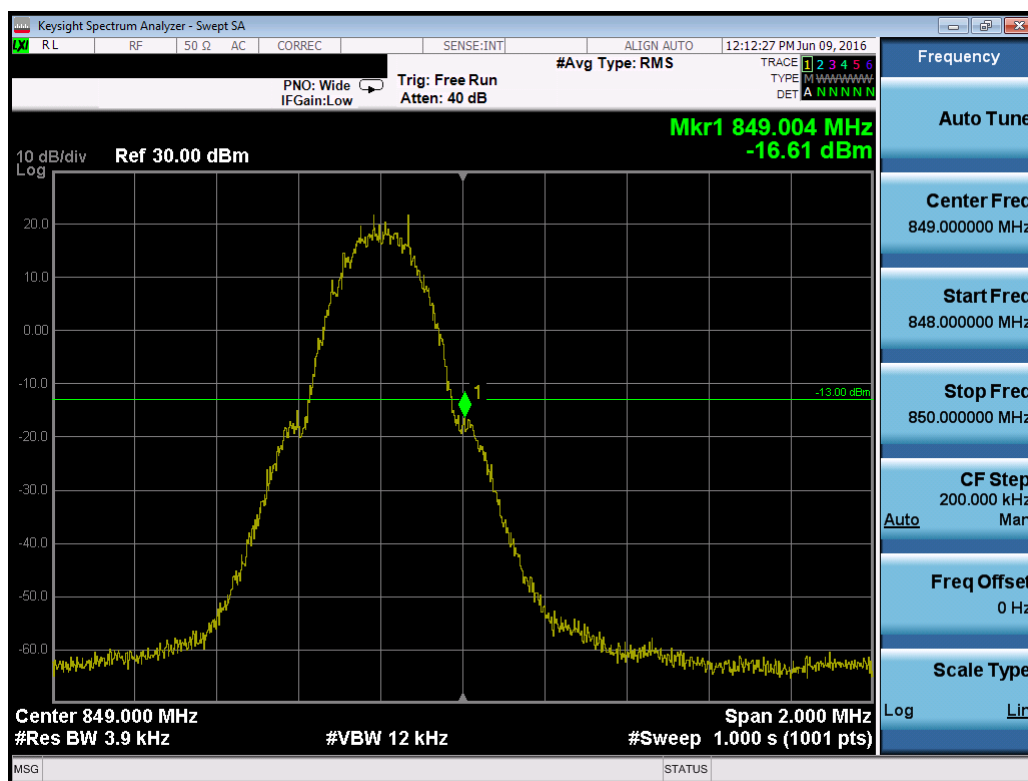
Plot 7-74. Band Edge Plot (Cellular GSM Mode – Ch. 251)
