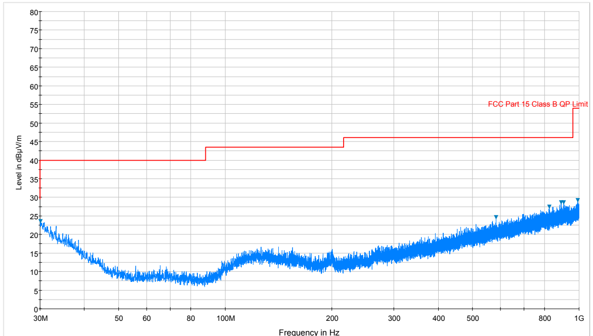
Plot 7-44. Radiated Spurious Plot below 1GHz (Pol. V)
