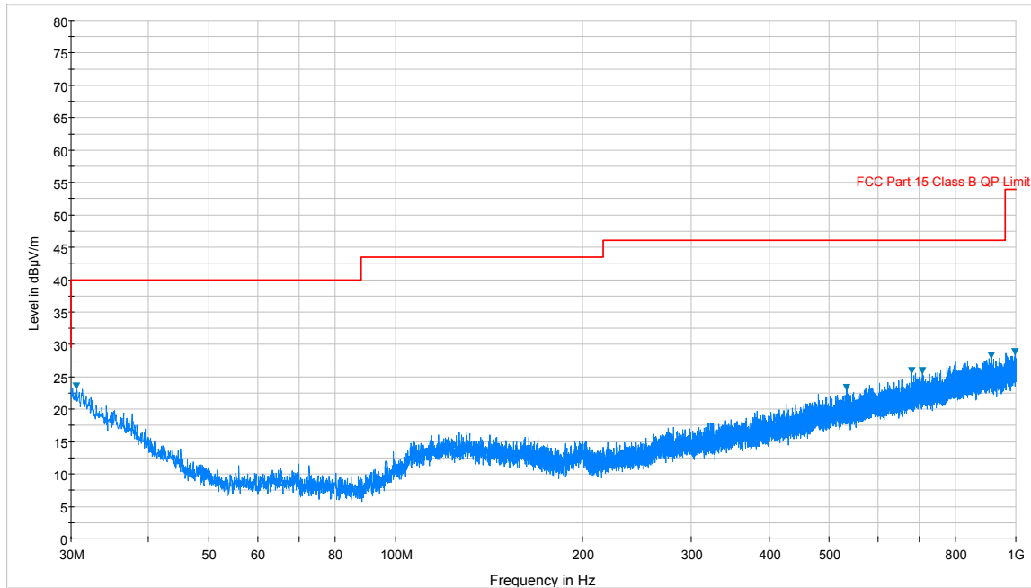
Plot 7-43. Radiated Spurious Plot below 1GHz (Pol. H)
