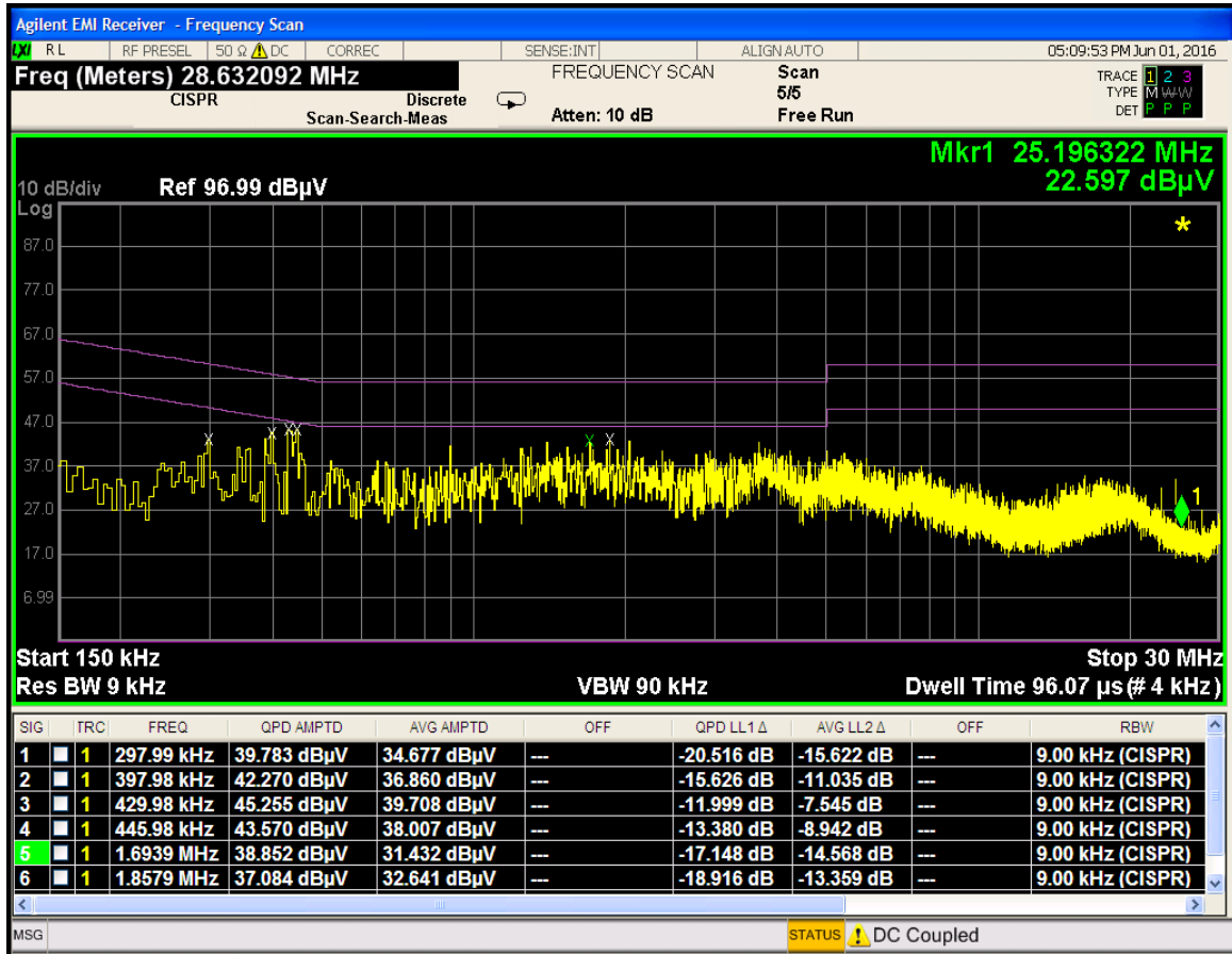
Plot 7-45. Line Conducted Plot with 802.11b (1)
