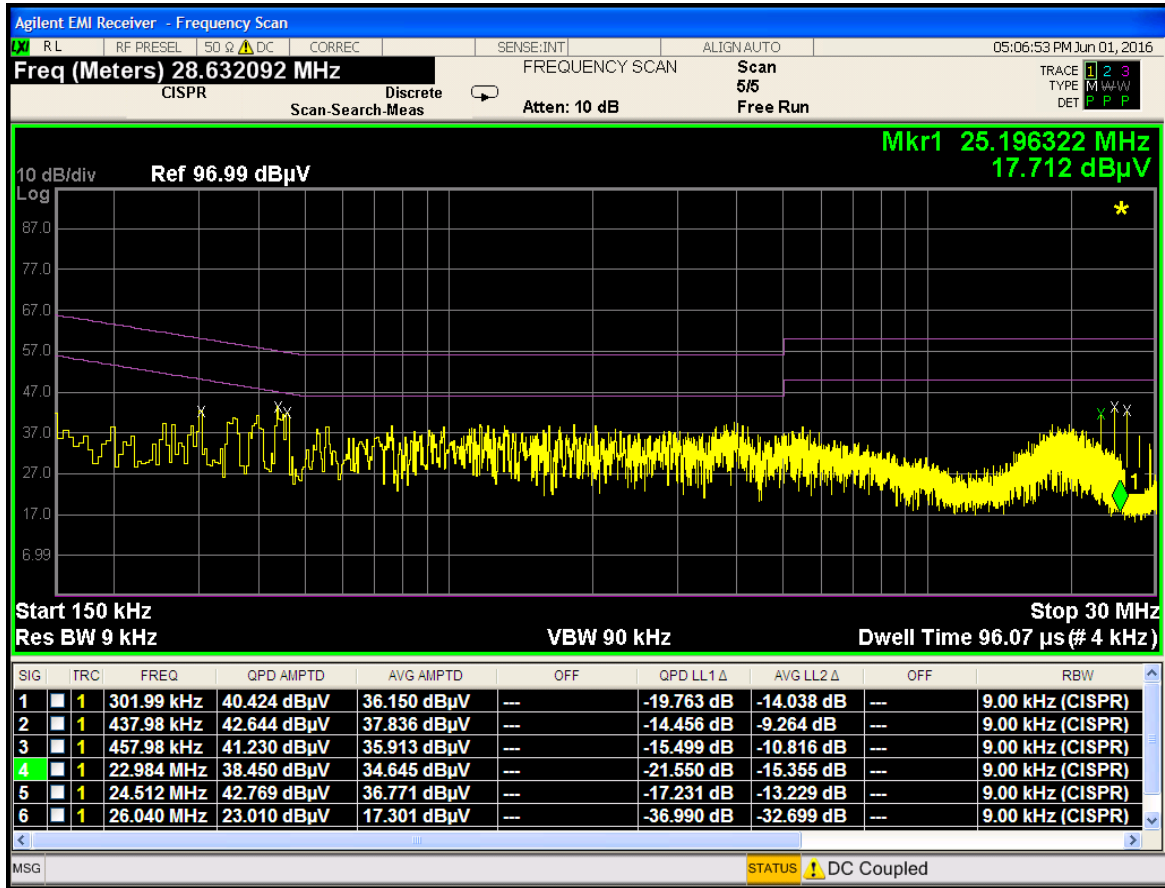
Plot 7-46. Line Conducted Plot with 802.11b (N)
