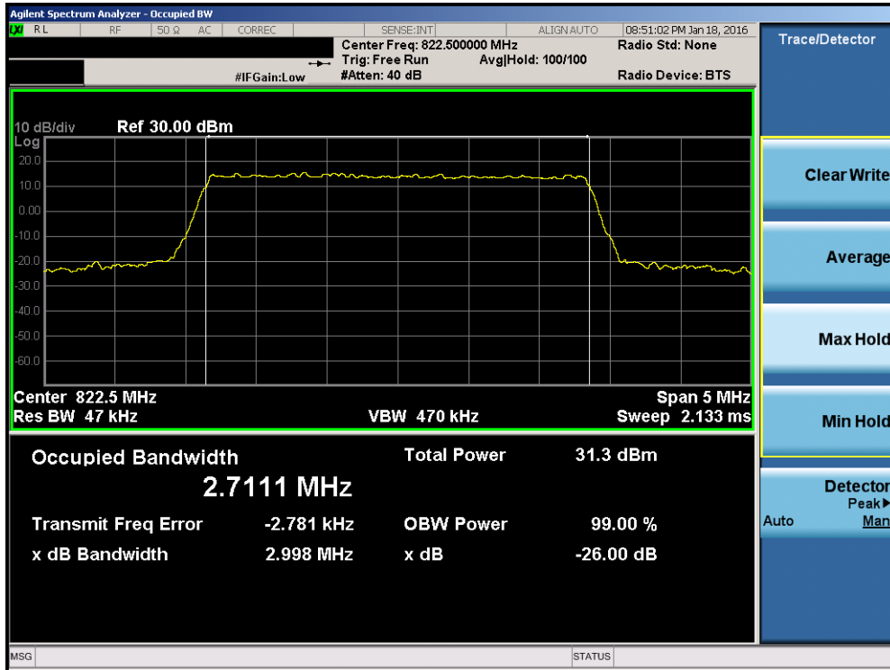
Plot 7-9. Occupied Bandwidth Plot (LTE Band 26 - 3MHz QPSK – RB Size 15– High Channel)
