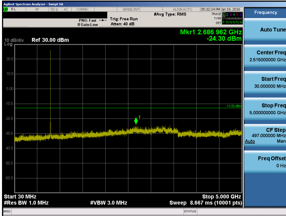
Plot 7-17. Conducted Spurious Plot (CDMA BC10 - Ch. 476)
