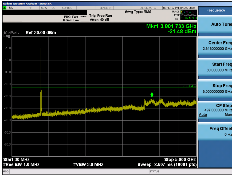
Plot 7-21. Conducted Spurious Plot (LTE Band 26 - 10MHz QPSK – RB Size 1, RB Offset 0)
