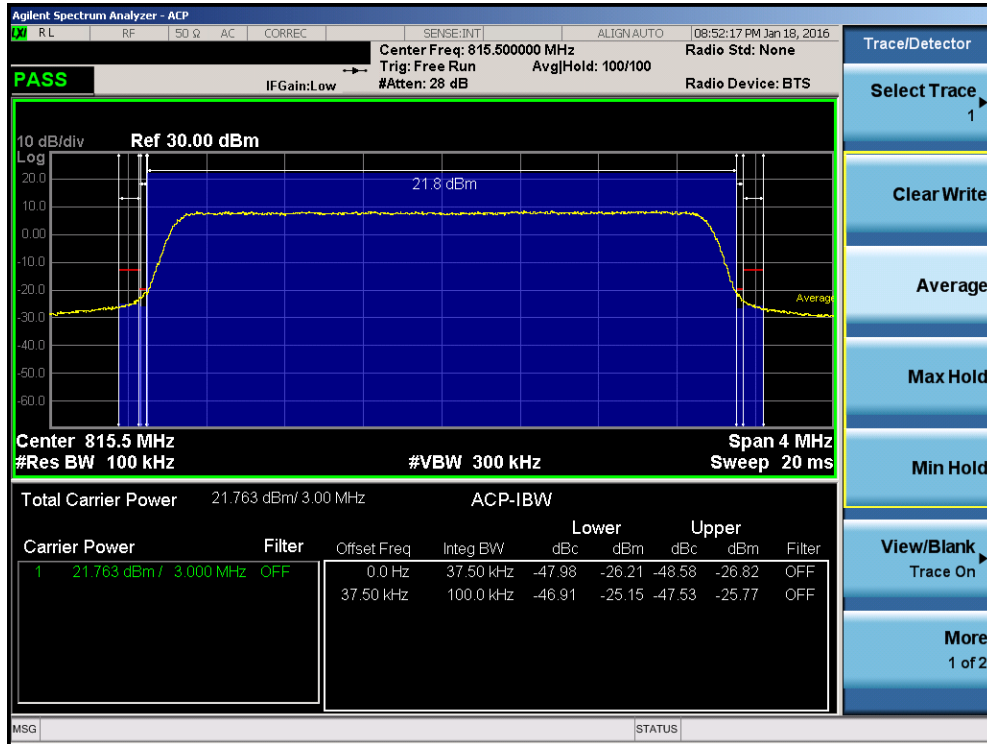
Plot 7-27. Channel Edge Plot (LTE Band 26 - 3MHz QPSK – RB Size 15– Low Channel)
