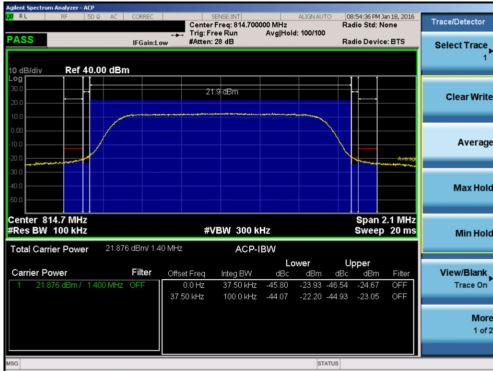
Plot 7-25. Channel Edge Plot (LTE Band 26 - 1.4MHz QPSK – RB Size 6– Low Channel)
