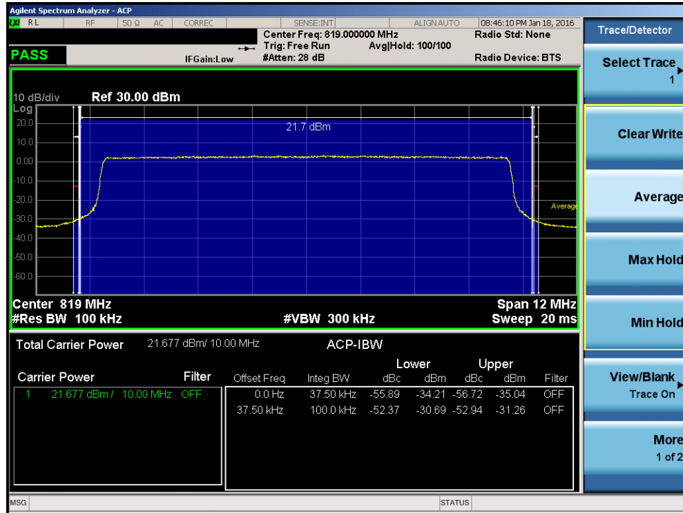
Plot 7-31. Channel Edge Plot (LTE Band 26 - 10MHz QPSK – RB Size 50)
