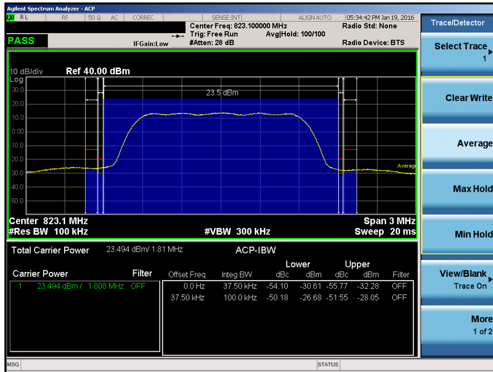
Plot 7-24. Channel Edge Plot (CDMA BC10 - Ch. 684)
