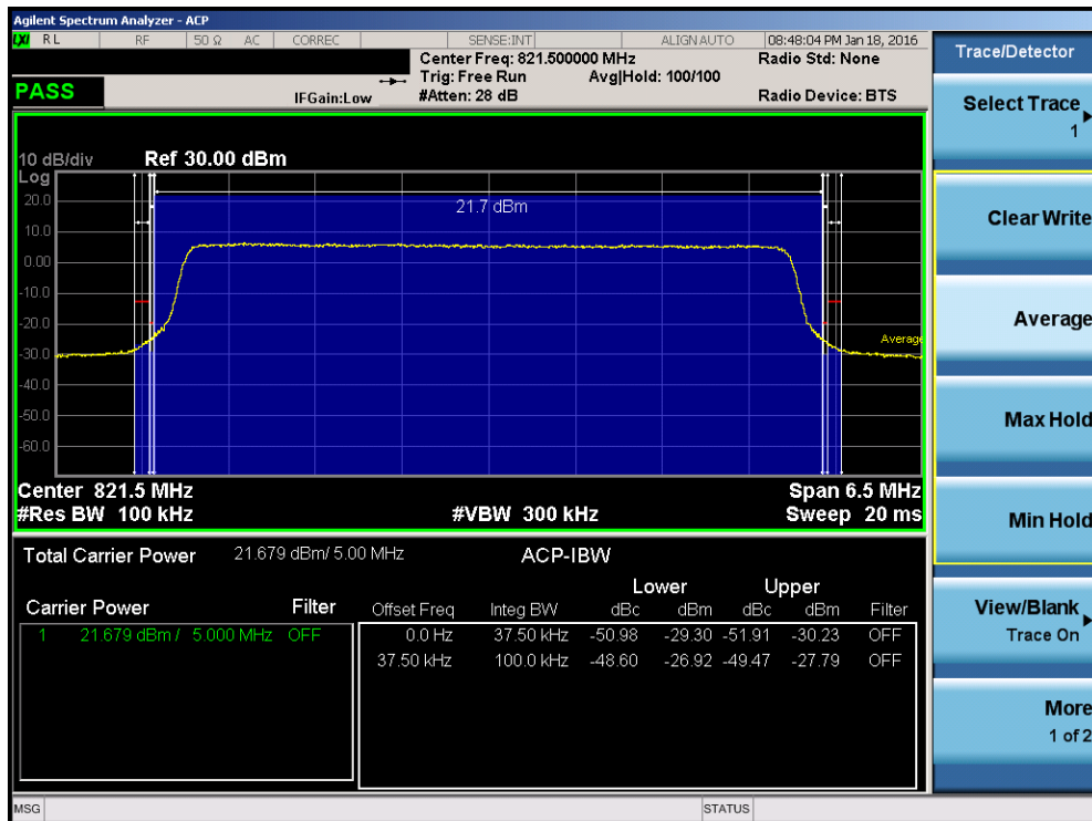
Plot 7-30. Channel Edge Plot (LTE Band 26 - 5MHz QPSK – RB Size 25 – High Channel)
