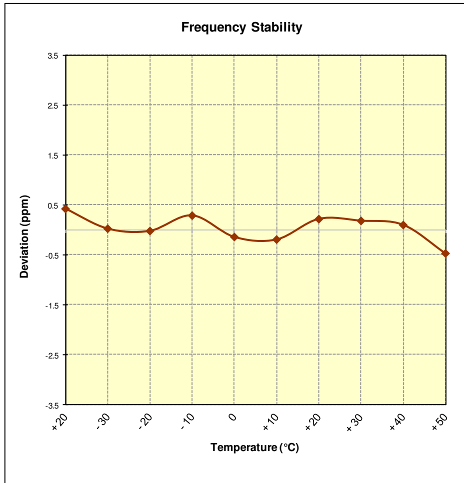
Figure 7-5. Frequency Stability Graph (CDMA BC10 - Ch. 476)
