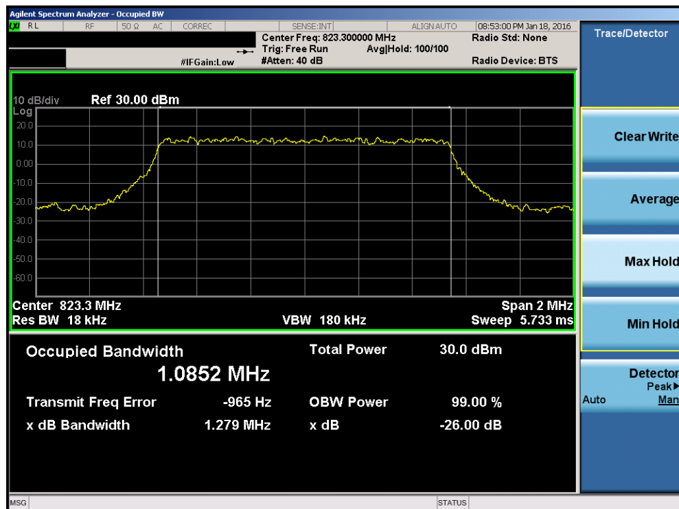
Plot 7-6. Occupied Bandwidth Plot (LTE Band 26 - 1.4MHz 16-QAM – RB Size 6– High Channel)
