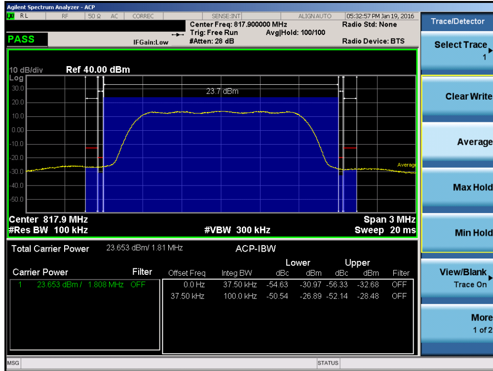
Plot 7-23. Channel Edge Plot (CDMA BC10 - Ch. 476)
