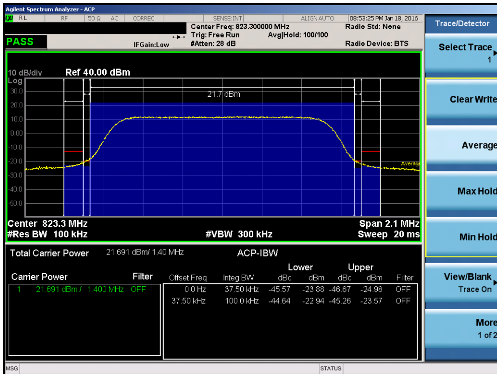
Plot 7-26. Channel Edge Plot (LTE Band 26 - 1.4MHz QPSK – RB Size 6 – High Channel)
