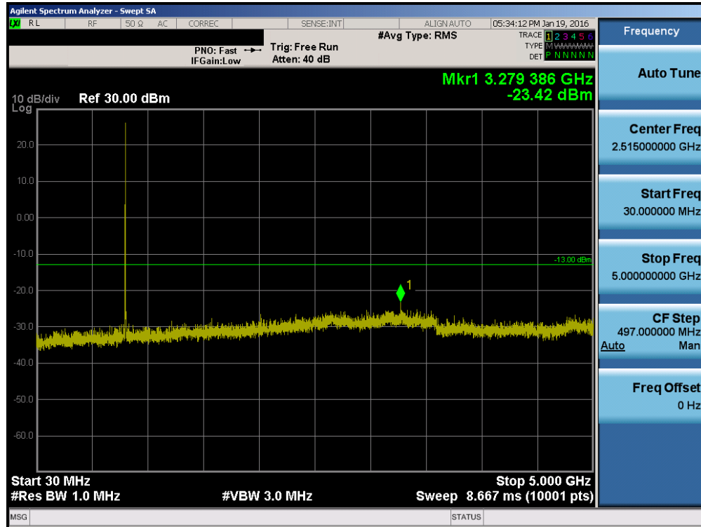
Plot 7-19. Conducted Spurious Plot (CDMA BC10 - Ch. 684)
