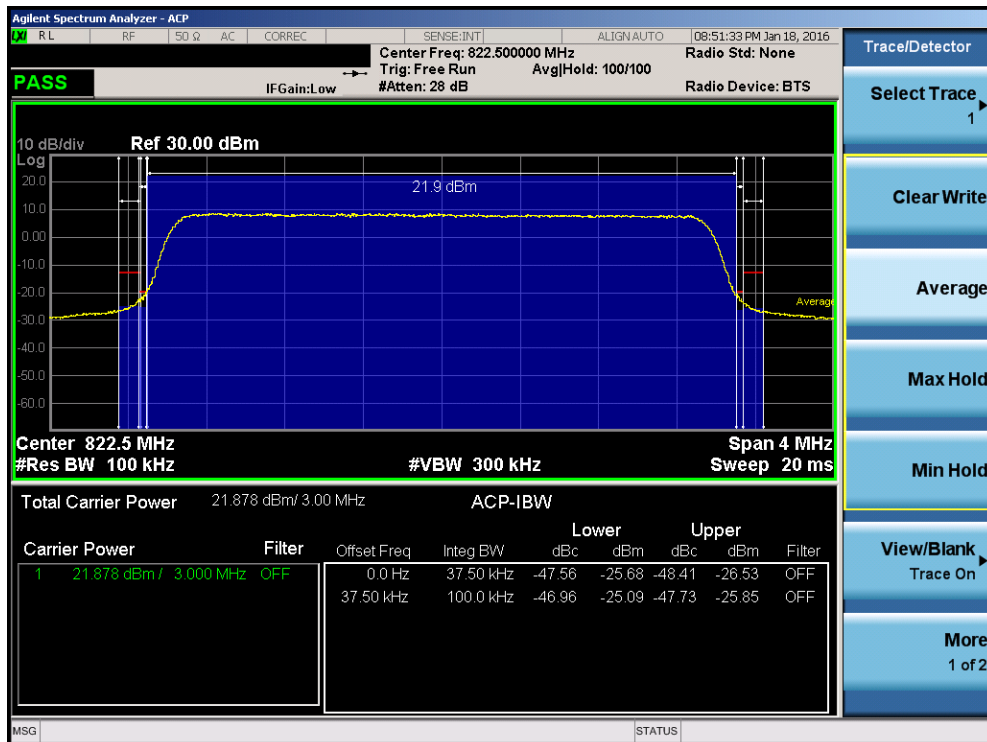
Plot 7-28. Channel Edge Plot (LTE Band 26 - 3MHz QPSK – RB Size 15 – High Channel)
