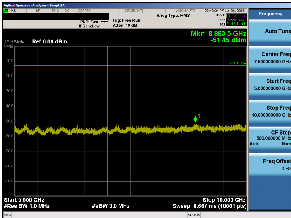
Plot 7-22. Conducted Spurious Plot (LTE Band 26 - 10MHz QPSK – RB Size 1, RB Offset 0)
