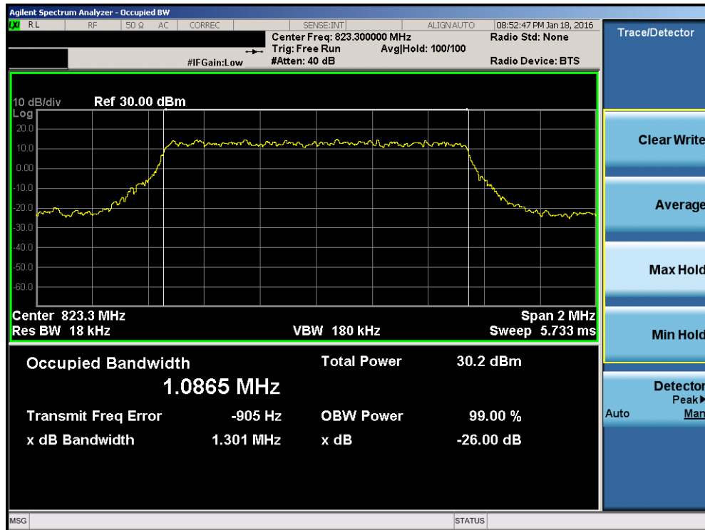
Plot 7-5. Occupied Bandwidth Plot (LTE Band 26 - 1.4MHz QPSK – RB Size 6– High Channel)
