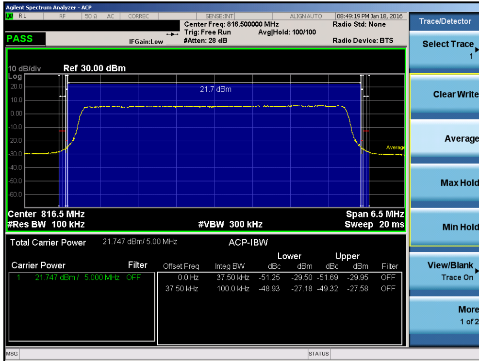
Plot 7-29. Channel Edge Plot (LTE Band 26 - 5MHz QPSK – RB Size 25– Low Channel)
