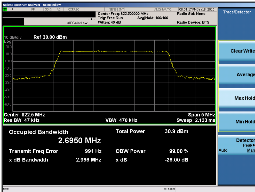
Plot 7-10. Occupied Bandwidth Plot (LTE Band 26 - 3MHz 16-QAM – RB Size 15– High Channel)
