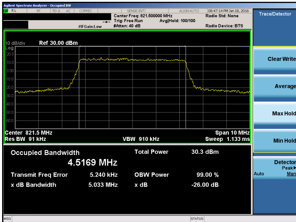
Plot 7-14. Occupied Bandwidth Plot (LTE Band 26 - 5MHz 16-QAM – RB Size 25– High Channel)
