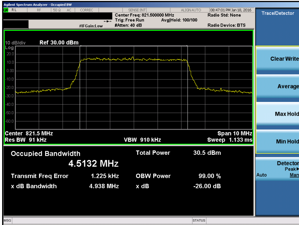
Plot 7-13. Occupied Bandwidth Plot (LTE Band 26 - 5MHz QPSK – RB Size 25– High Channel)
