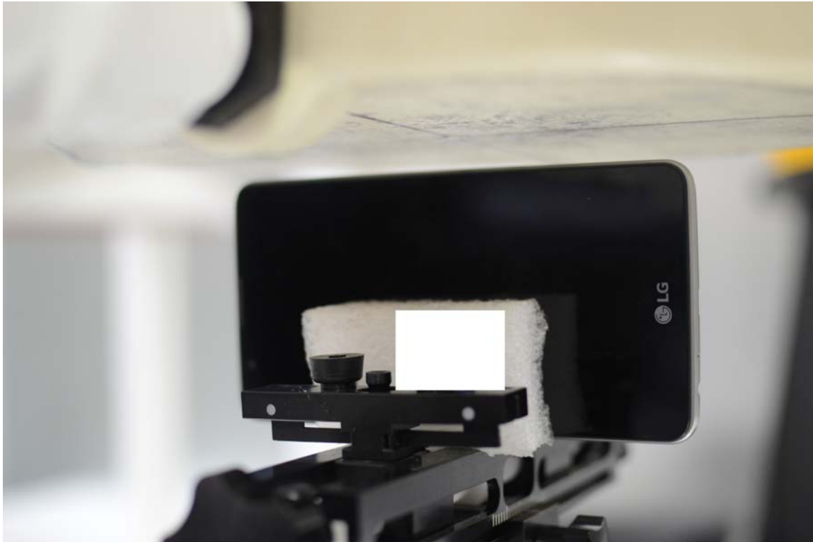
SAR Test Setup Photo 9 – Right Edge (10 mm)
