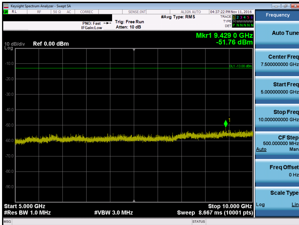
Plot 7-18. Conducted Spurious Plot (5MHz QPSK – RB Size 1, RB Offset 0 – Low Channel)
