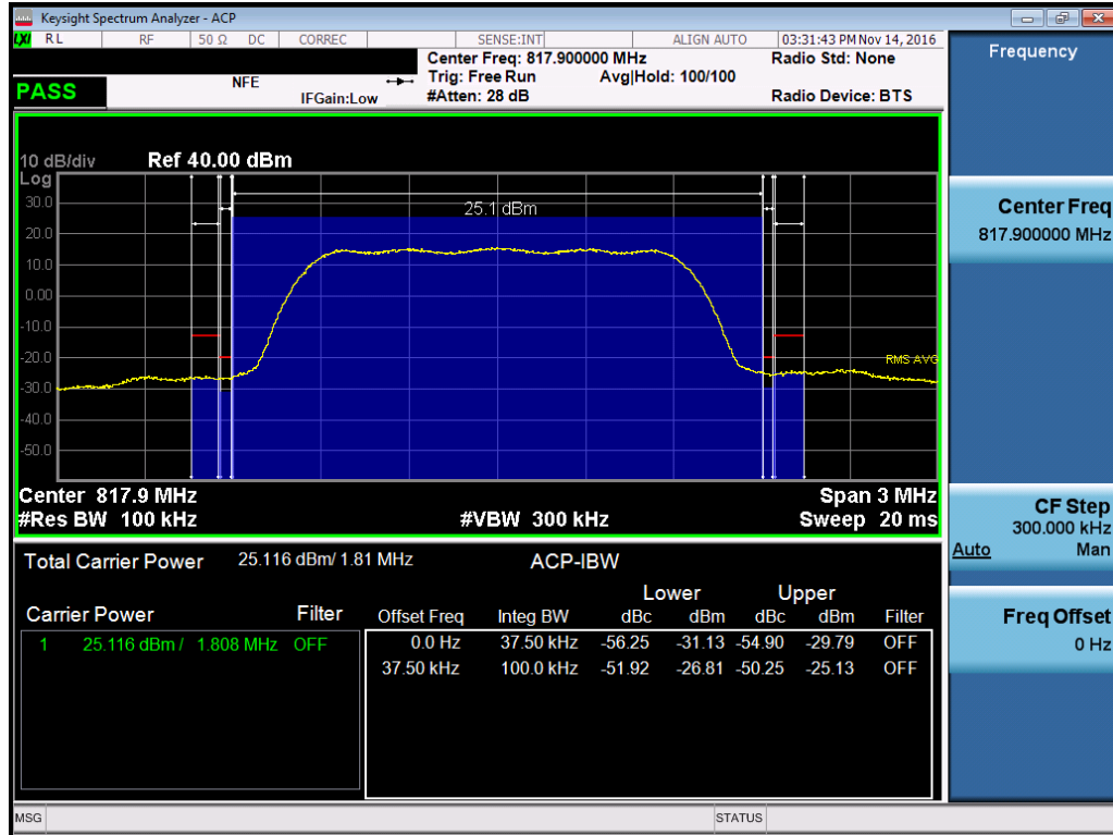
Plot 7-21. Channel Edge Plot (Ch. 476)
