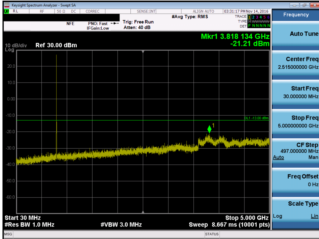
Plot 7-13. Conducted Spurious Plot (Ch. 476)
