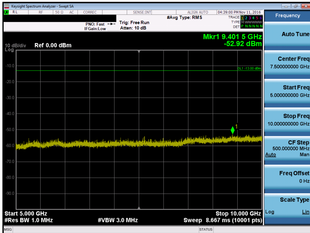
Plot 7-20. Conducted Spurious Plot (5MHz QPSK – RB Size 1, RB Offset 0 – High Channel)
