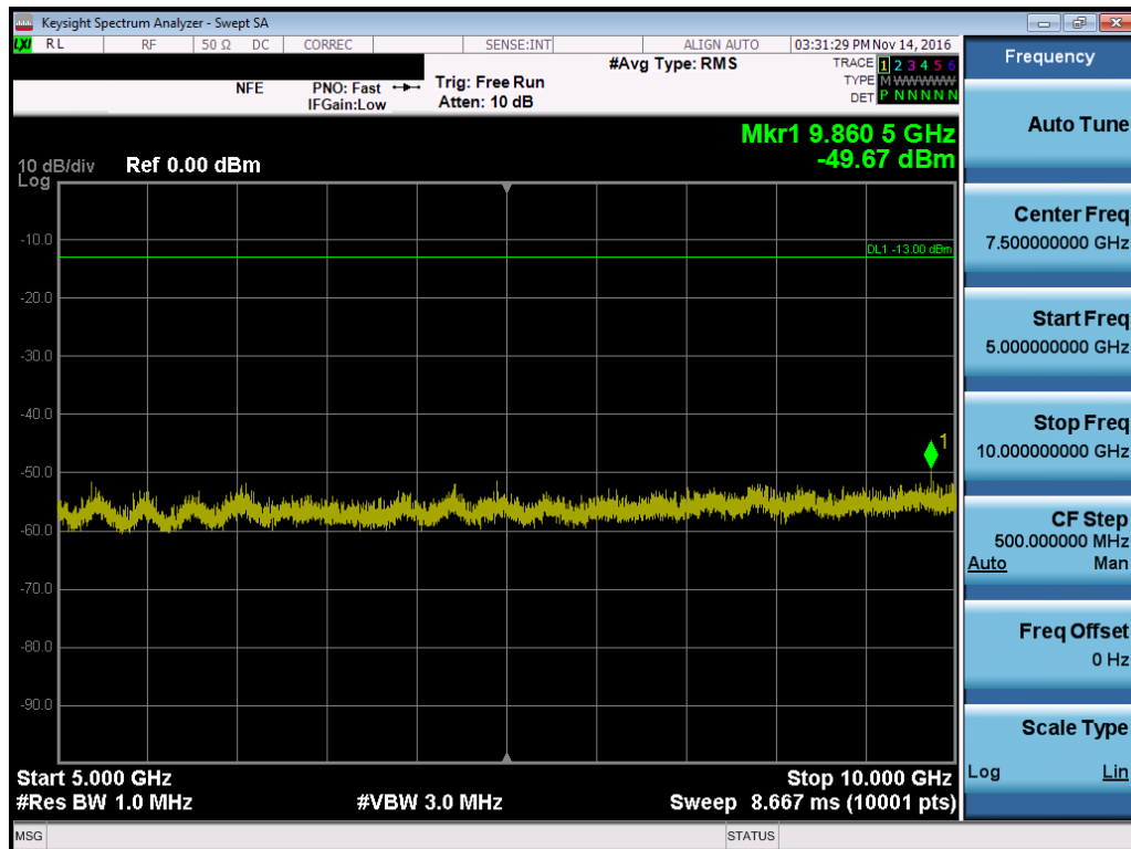
Plot 7-14. Conducted Spurious Plot (Ch. 476)
