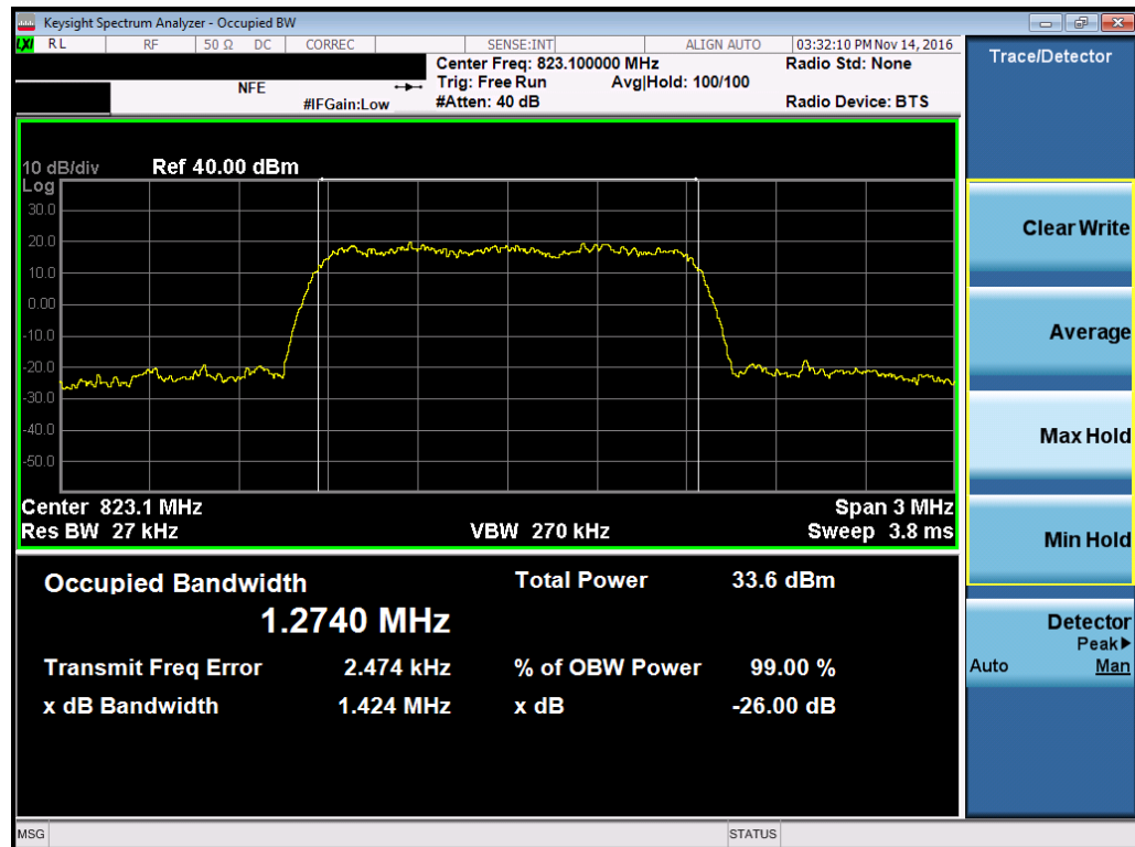
Plot 7-2. Occupied Bandwidth Plot (Ch. 684)
