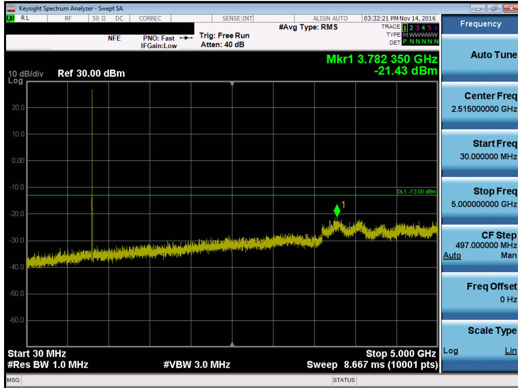
Plot 7-15. Conducted Spurious Plot (Ch. 684)
