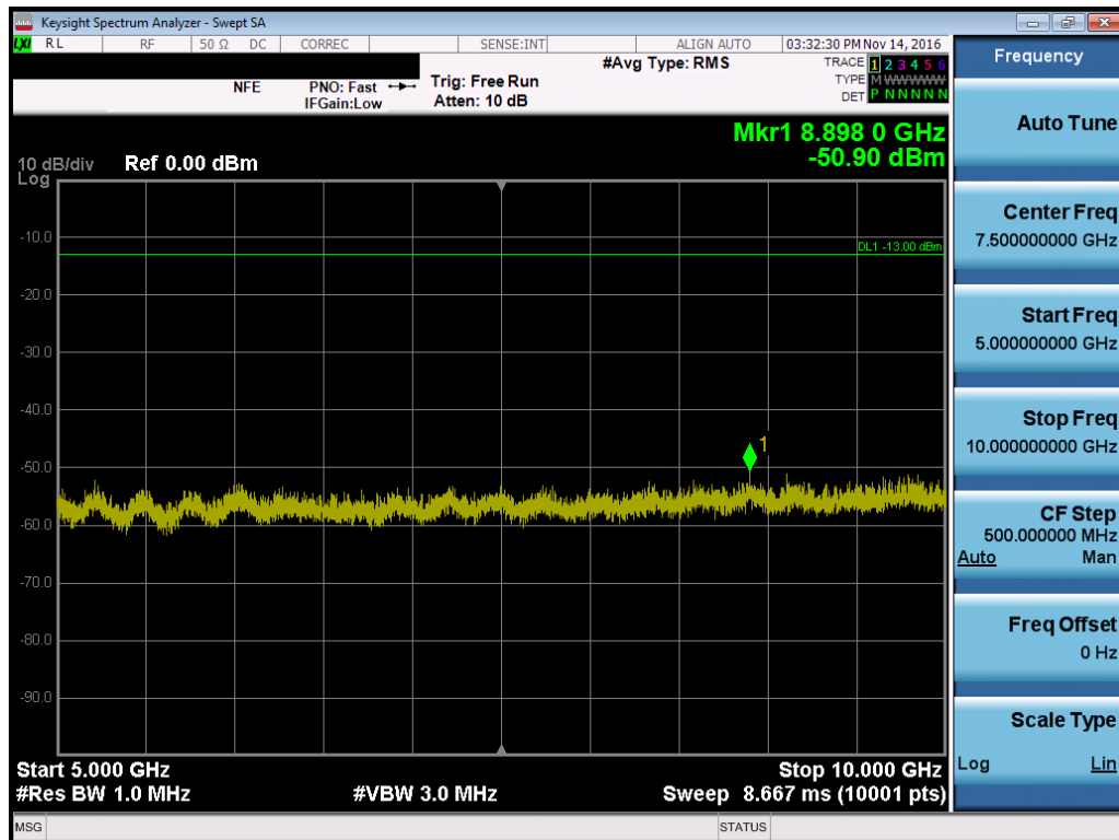
Plot 7-16. Conducted Spurious Plot (Ch. 684)
