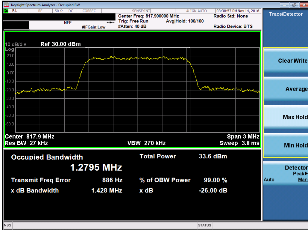
Plot 7-1. Occupied Bandwidth Plot (Ch. 476)
