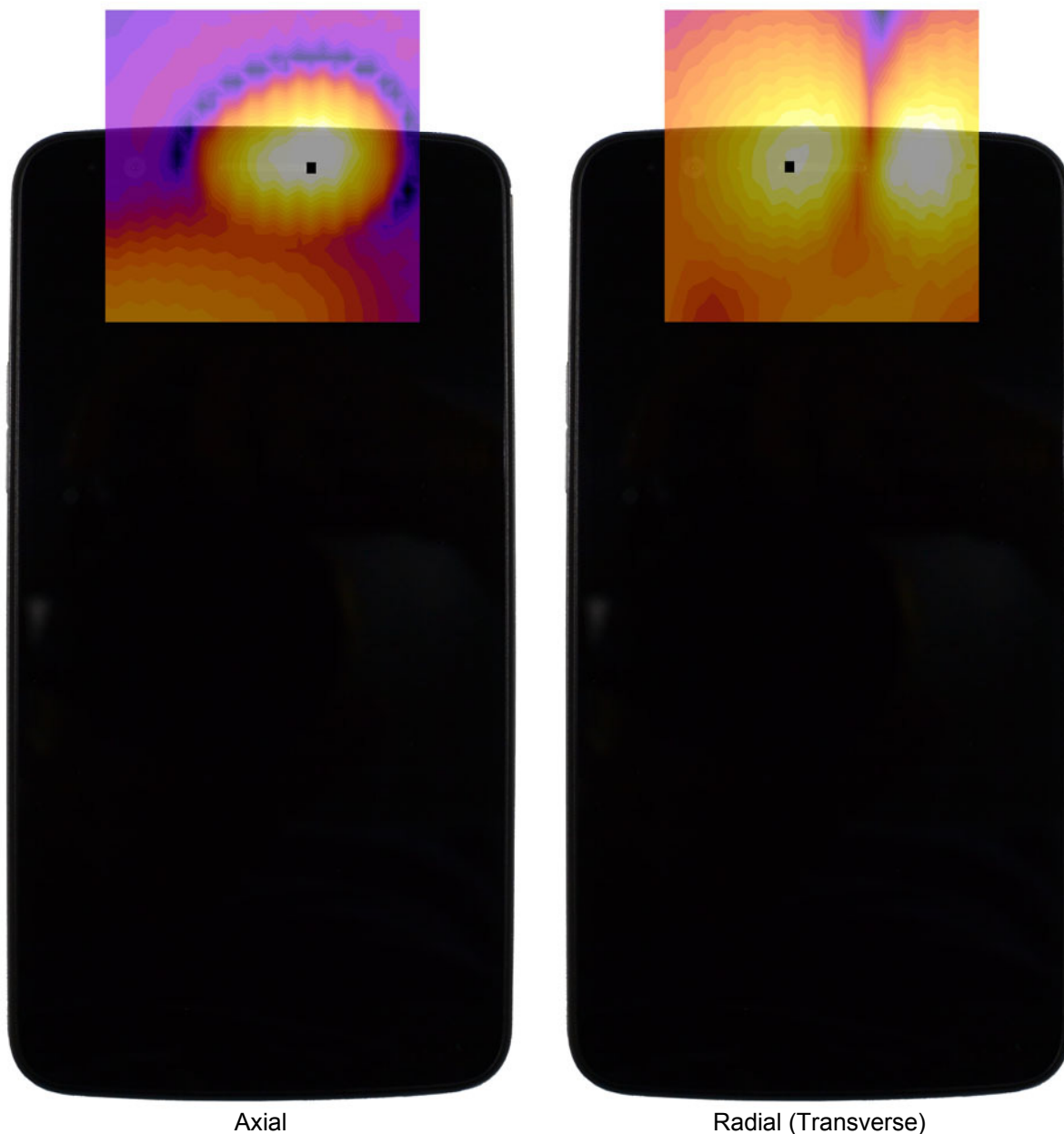
Axial Radial (Transverse) Figure 13-3 T-Coil Scan Overlay Magnetic Field Distributions
