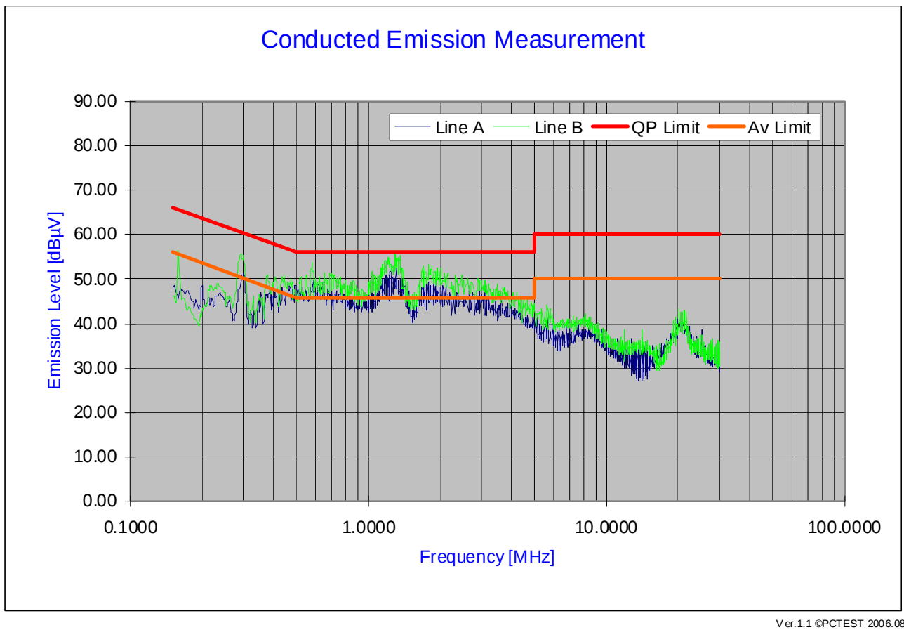
Plot 6-22. Line Conducted Plot with Bluetooth
