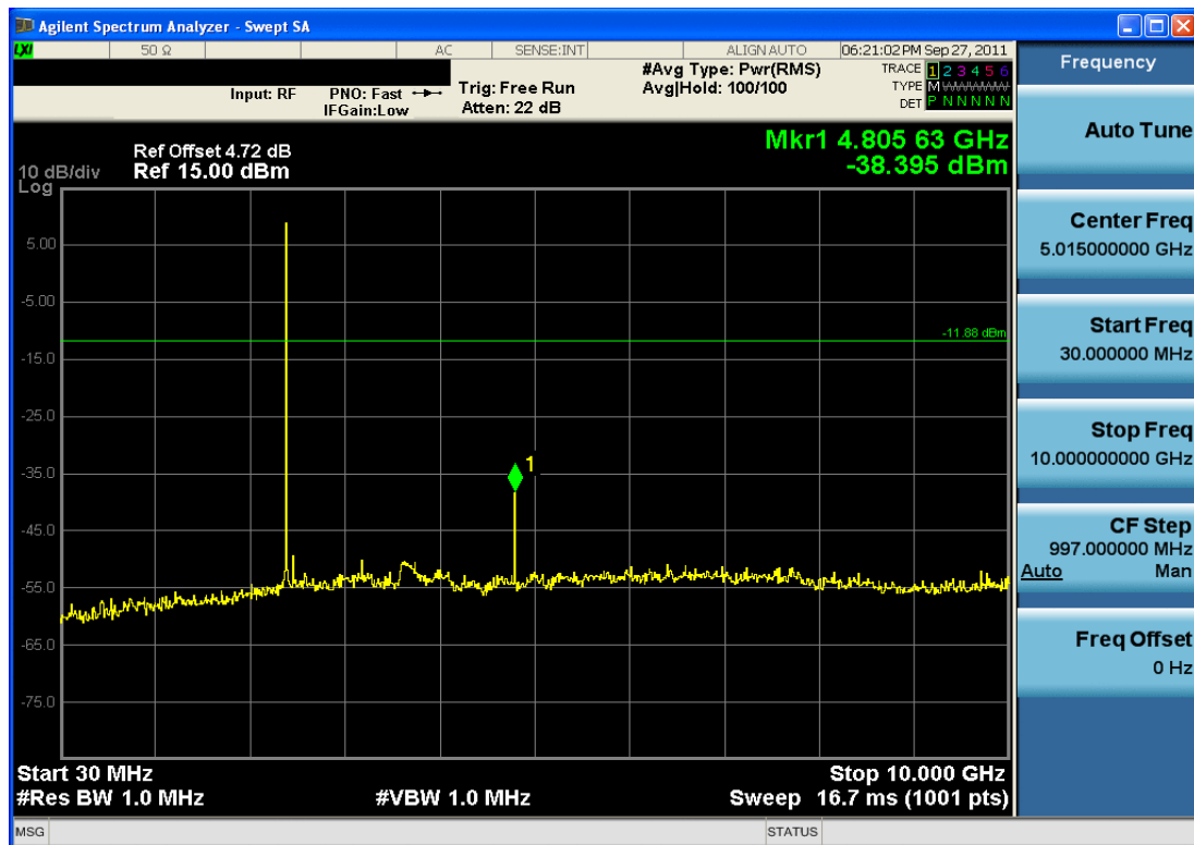
Plot 6-16. Conducted Spurious Plot (Bluetooth, 3Mbps – Ch. 0)
