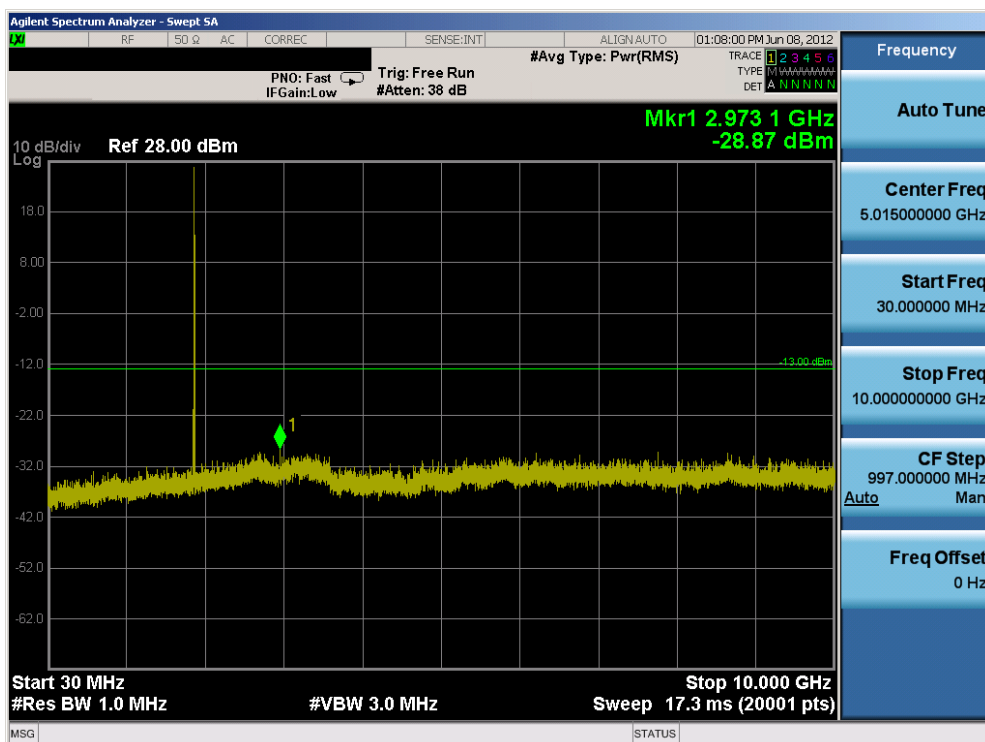
Plot 7-9. Conducted Spurious Plot (Mid Channel - QPSK – 5MHz BW - RB Size 1, Offset 0)
