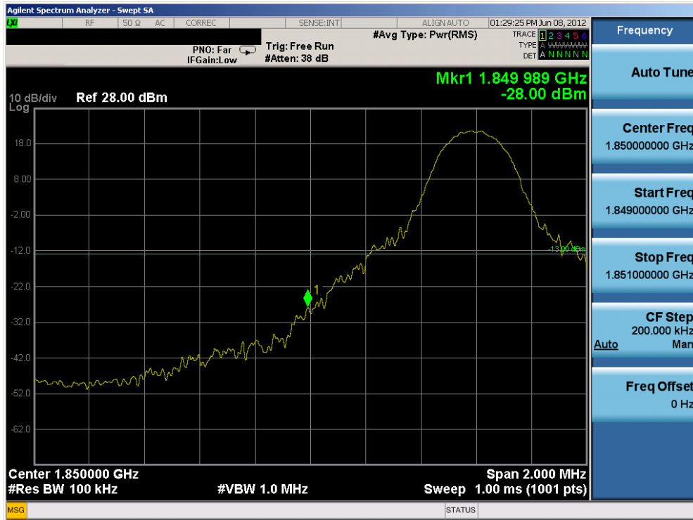
Plot 7-16. Lower Band Edge Plot (QPSK – 10MHz BW – RB Size 1, Offset 0)
