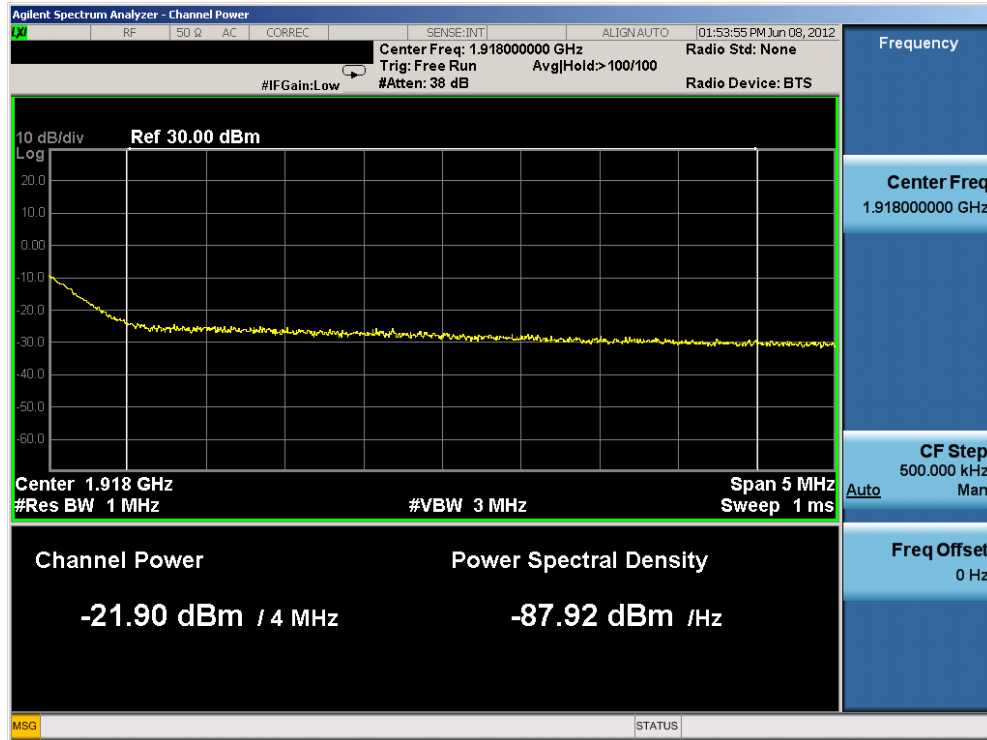
Plot 7-28. Upper Band Edge Plot (QPSK – 10MHz BW – RB Size 50)
