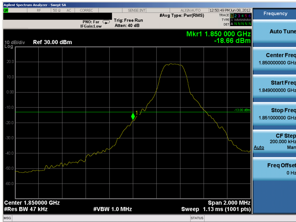
Plot 7-2. Lower Band Edge Plot (QPSK – 5MHz BW – RB Size 1, Offset 0)
