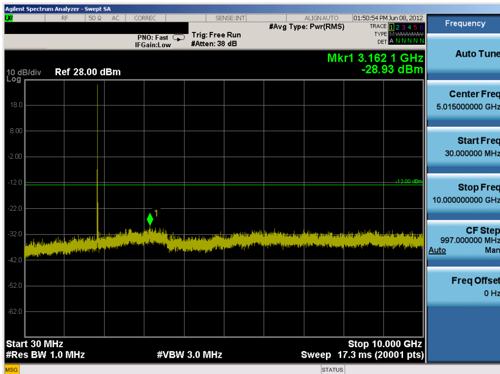
Plot 7-21. Conducted Spurious Plot (Low Channel – QPSK – 10MHz BW – - RB Size 1, Offset 0)
