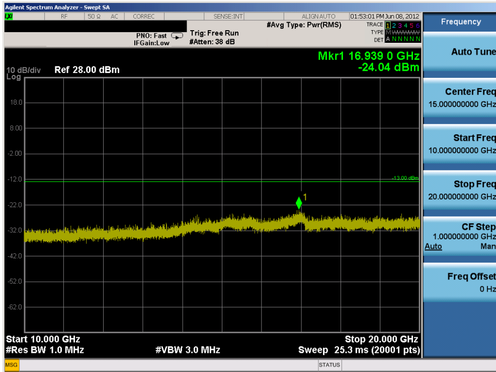
Plot 7-26. Conducted Spurious Plot (High Channel – QPSK – 10MHz BW - RB Size 1, Offset 0)
