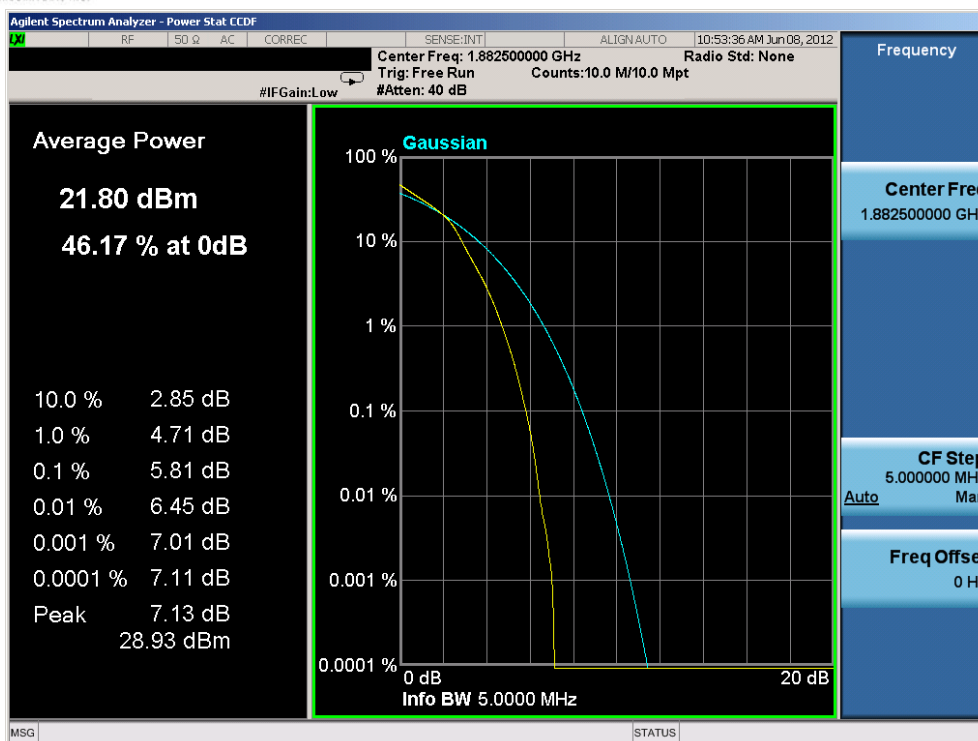
Plot 7-6. Peak-Average Ratio Plot (16-QAM – 5MHz BW – RB Size 25)
