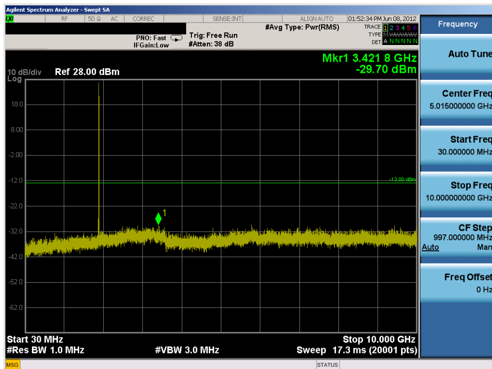
Plot 7-25. Conducted Spurious Plot (High Channel – QPSK – 10MHz BW - RB Size 1, Offset 0)
