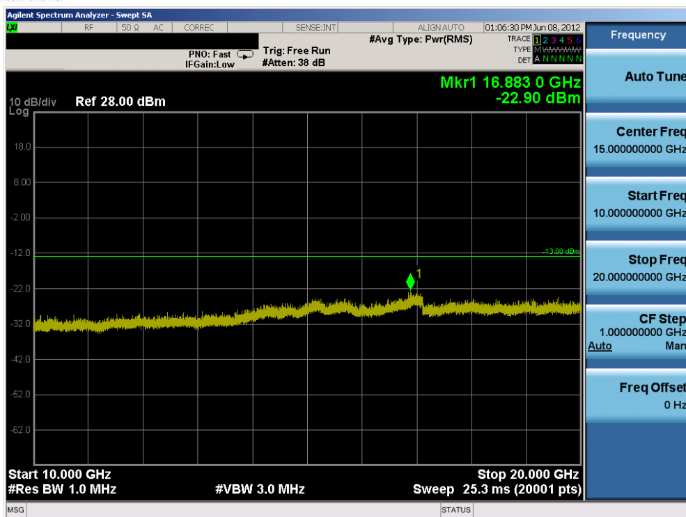
Plot 7-8. Conducted Spurious Plot (Low Channel – QPSK – 5MHz BW – RB Size 1, RB Offset 0)
