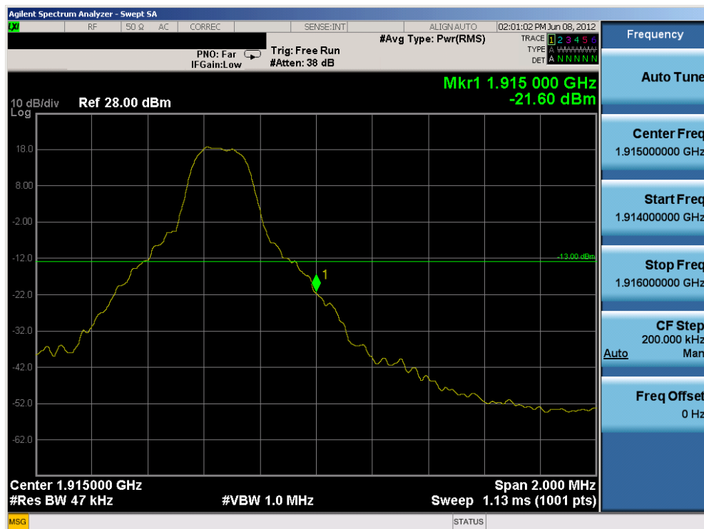
Plot 7-13. Upper Band Edge Plot (QPSK – 5MHz BW – RB Size 1, Offset 24)
