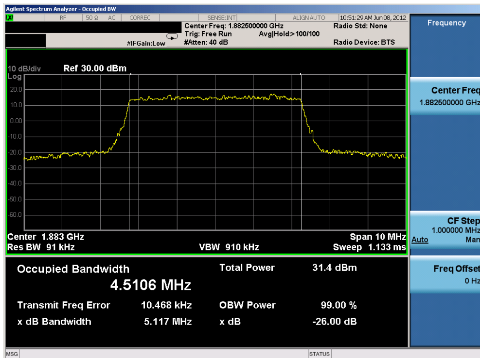
Plot 7-3. Occupied Bandwidth Plot (QPSK – 5MHz BW – RB Size 25)
