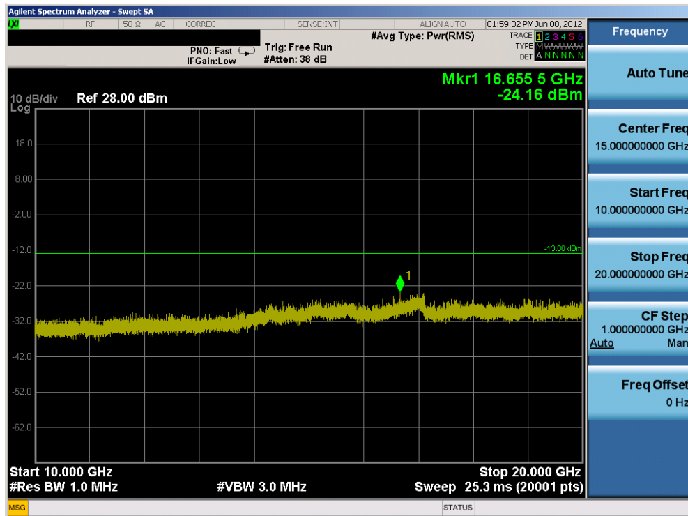
Plot 7-24. Conducted Spurious Plot (Mid Channel – QPSK – 10MHz BW - RB Size 1, Offset 0)
