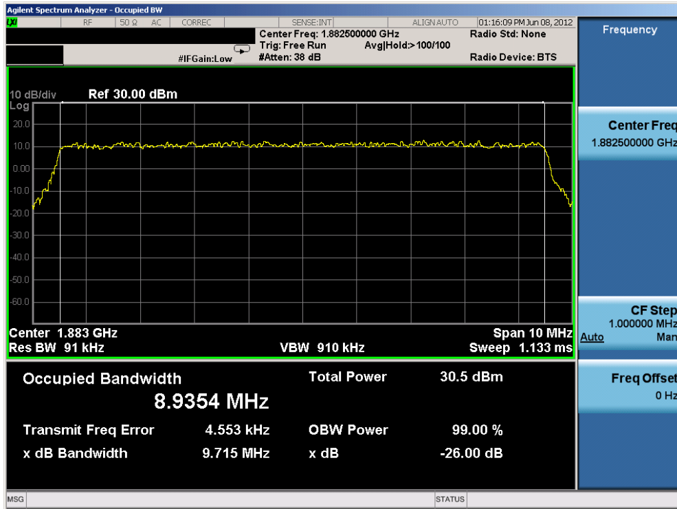
Plot 7-18. Occupied Bandwidth Plot (16-QAM – 10MHz BW – RB Size 50)
