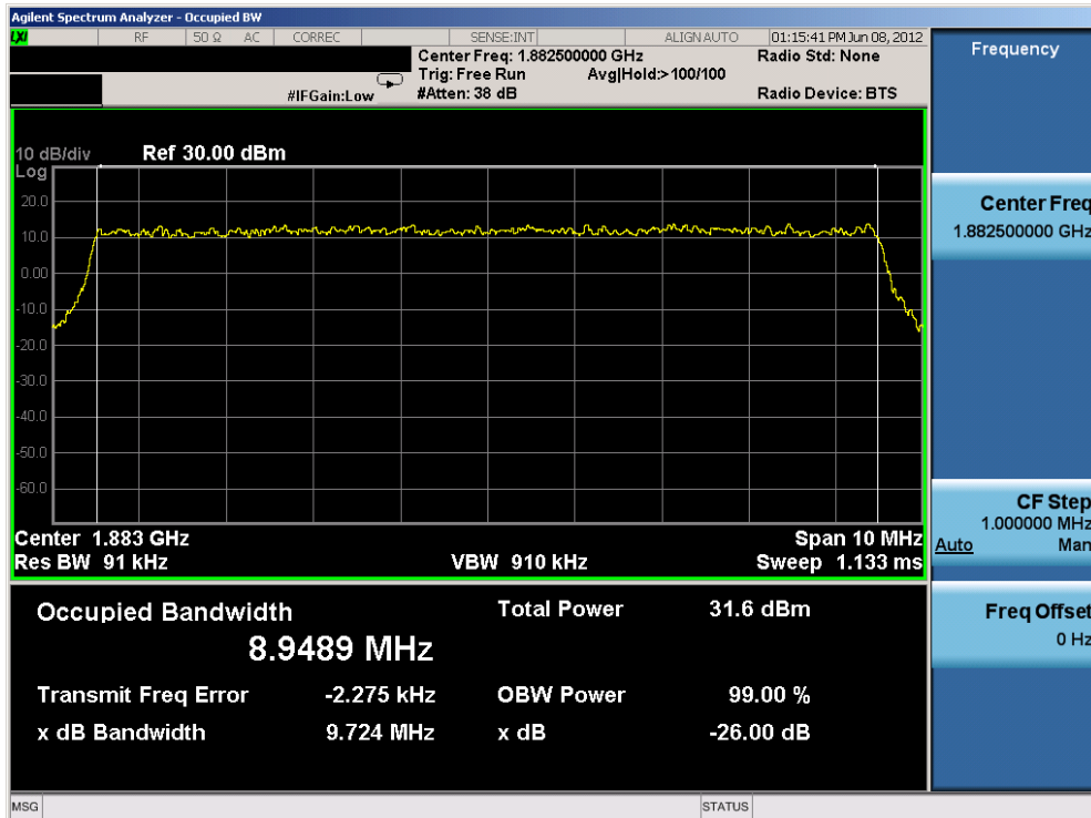
Plot 7-17. Occupied Bandwidth Plot (QPSK – 10MHz BW – RB Size 50)
