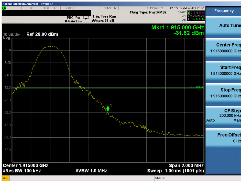
Plot 7-27. Upper Band Edge Plot (QPSK – 10MHz BW – RB Size 1, Offset 49)
