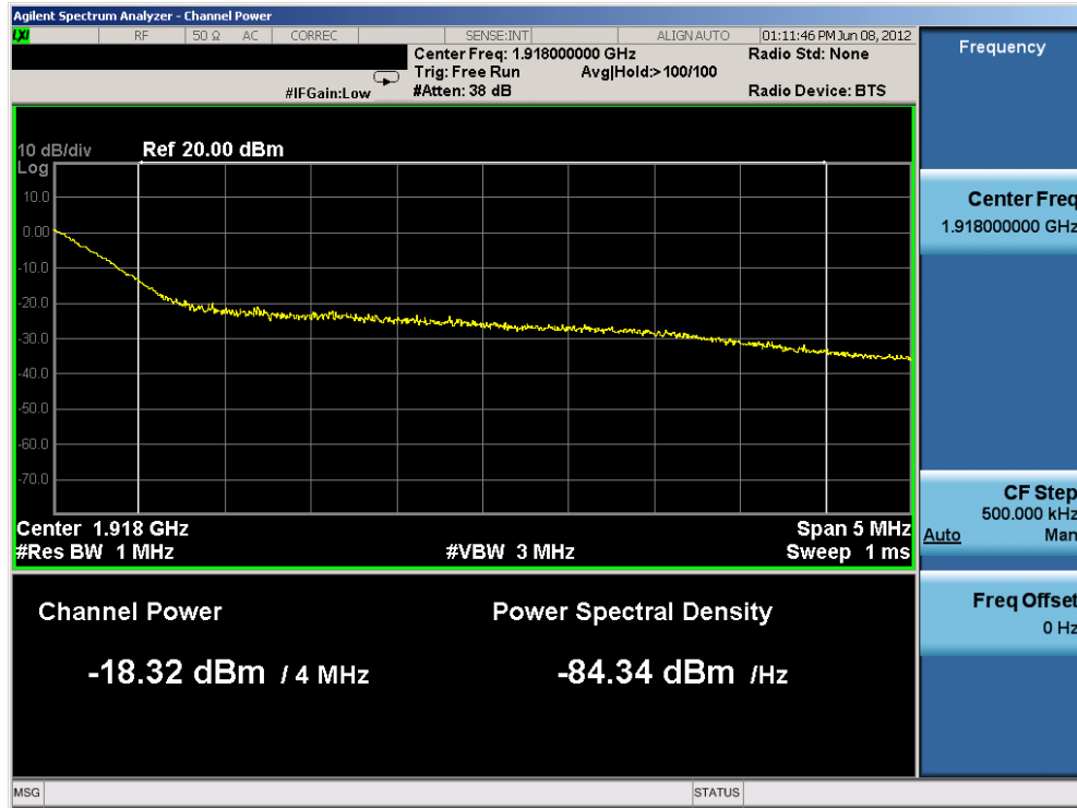
Plot 7-14. Upper Band Edge Plot (QPSK - 5MHz BW - RB Size 25)
