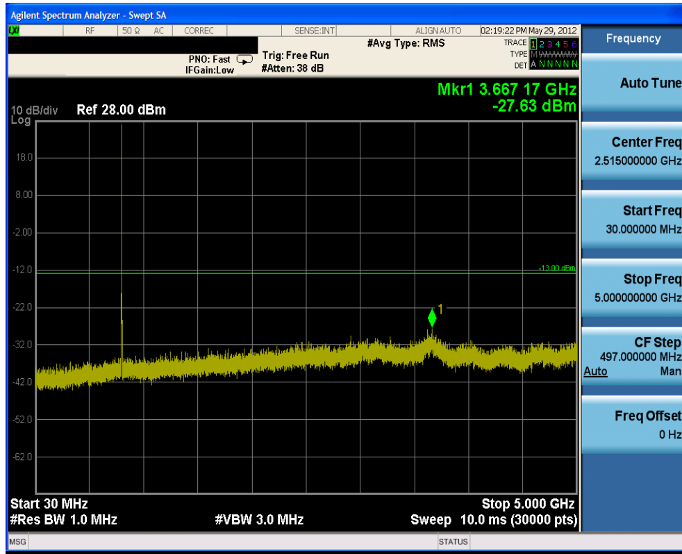
Plot 7-5. Conducted Spurious Plot (Ch. 684)
