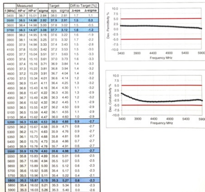
Figure D-4 5GHz Head Tissue Equivalent Matter
