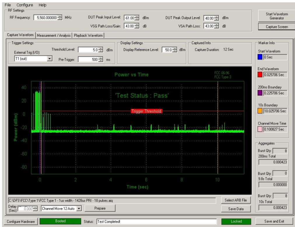
Figure 5-2. Band 2C Move Time and Aggregate Time
