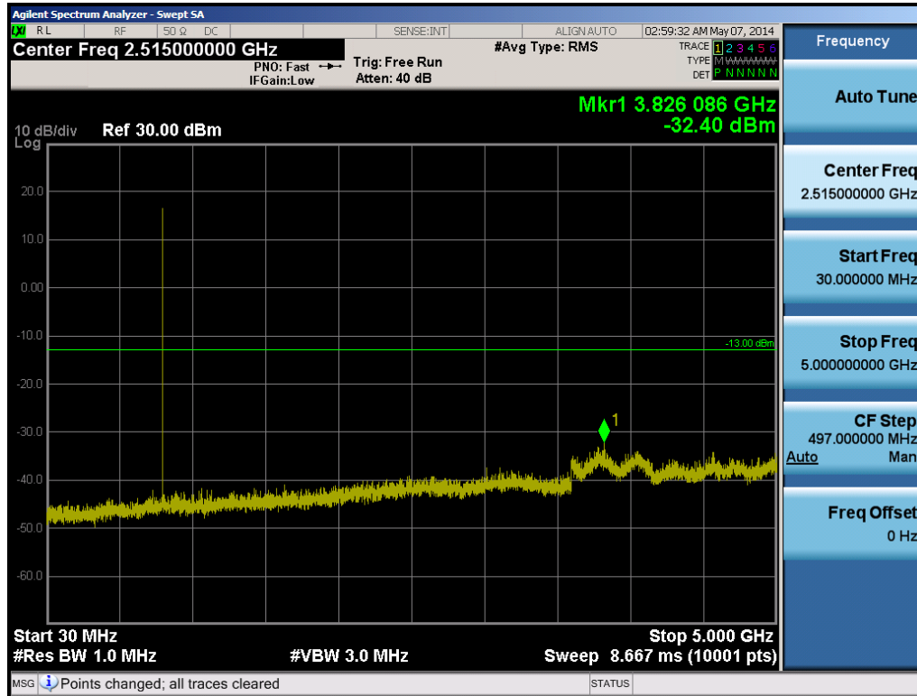
Plot 6-15. Conducted Spurious Plot (1.4MHz QPSK – RB Size 1, RB Offset 0 – Low Channel)
