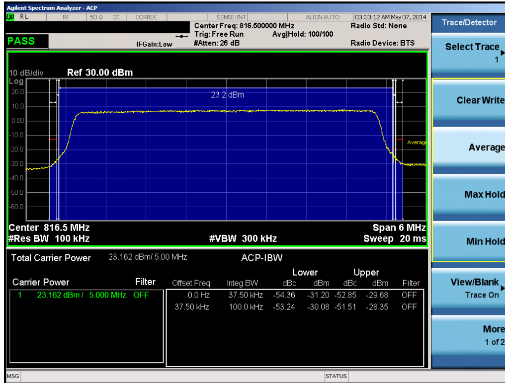
Plot 6-29. Channel Edge Plot (5MHz QPSK – RB Size 25– Low Channel)
