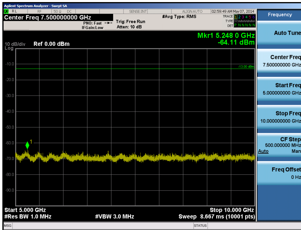
Plot 6-16. Conducted Spurious Plot (1.4MHz QPSK – RB Size 1, RB Offset 0 – Low Channel)
