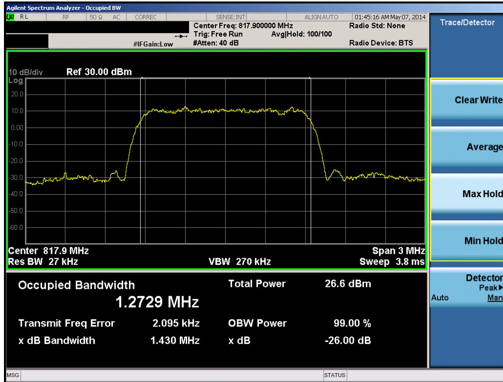
Plot 6-1. CDMA BC10 Occupied Bandwidth Plot (Ch. 476)
