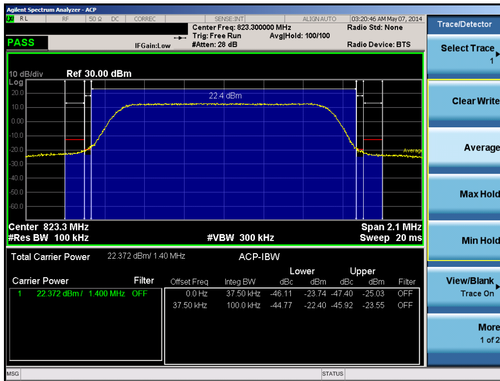
Plot 6-26. Channel Edge Plot (1.4MHz QPSK – RB Size 6 – High Channel)
