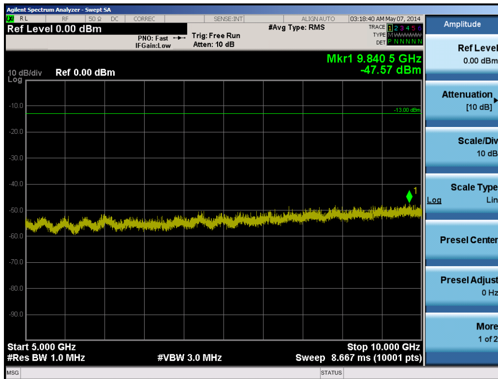
Plot 6-18. Conducted Spurious Plot (1.4MHz QPSK – RB Size 1, RB Offset 0 – High Channel)
