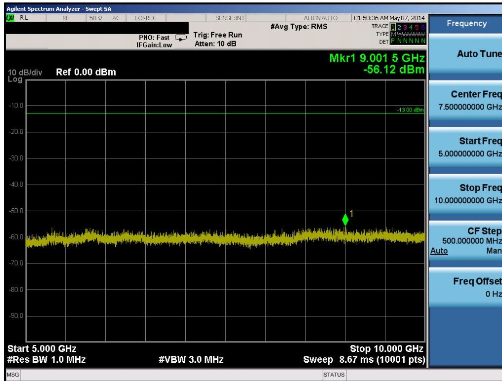
Plot 6-14. CDMA BC10 Conducted Spurious Plot (Ch. 684)
