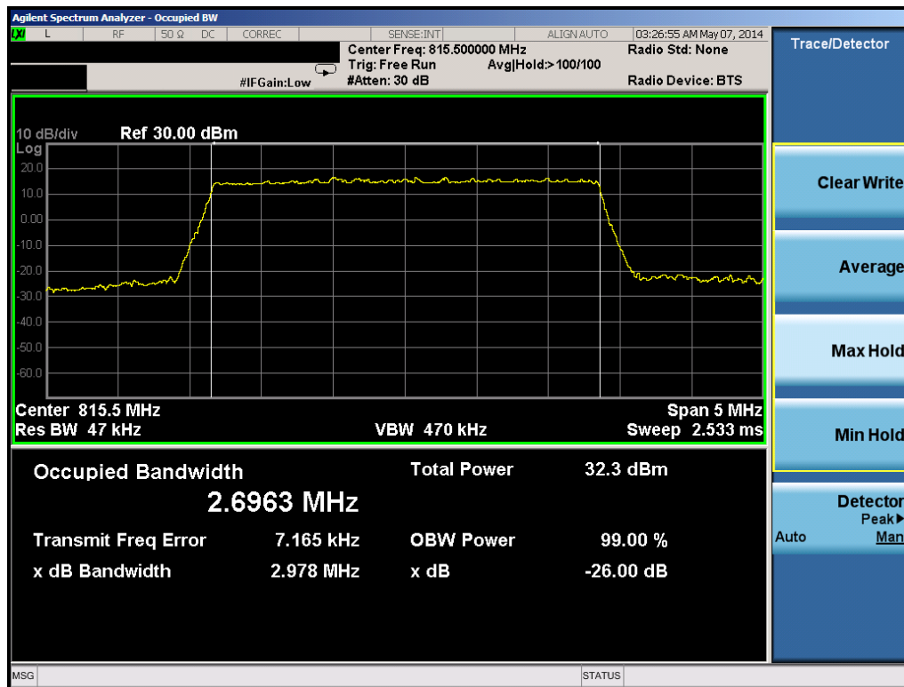
Plot 6-6. B26 Occupied Bandwidth Plot (3MHz 16-QAM – RB Size 15– Low Channel))
