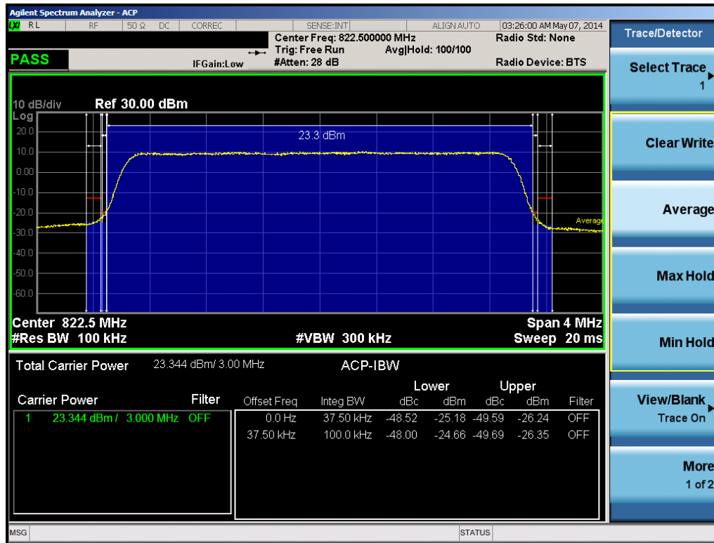
Plot 6-28. Channel Edge Plot (3MHz QPSK – RB Size 15 – High Channel)
