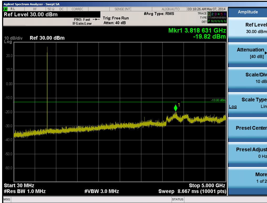
Plot 6-17. Conducted Spurious Plot (1.4MHz QPSK – RB Size 1, RB Offset 0 – High Channel)
