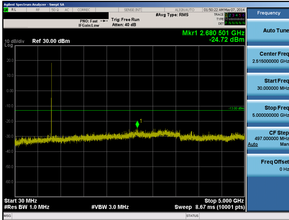
Plot 6-13. CDMA BC10 Conducted Spurious Plot (Ch. 684)
