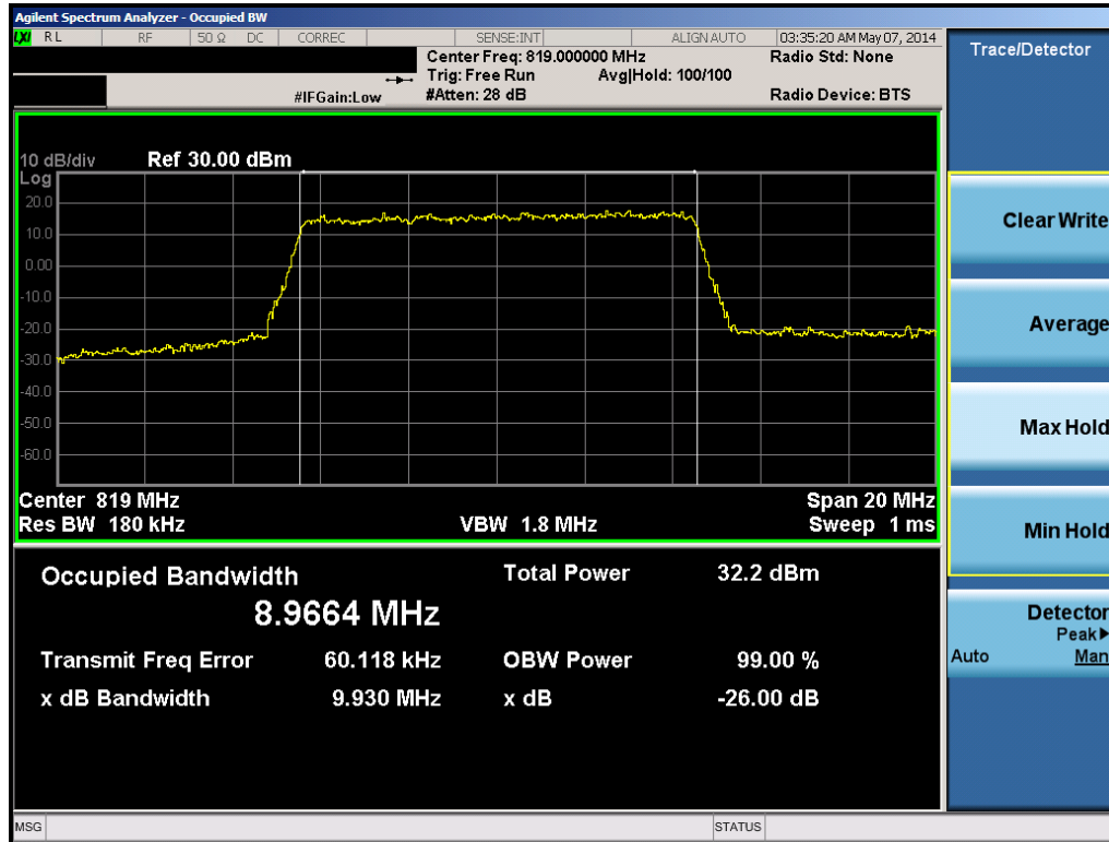
Plot 6-9. B26 Occupied Bandwidth Plot (10MHz QPSK – RB Size 50)
