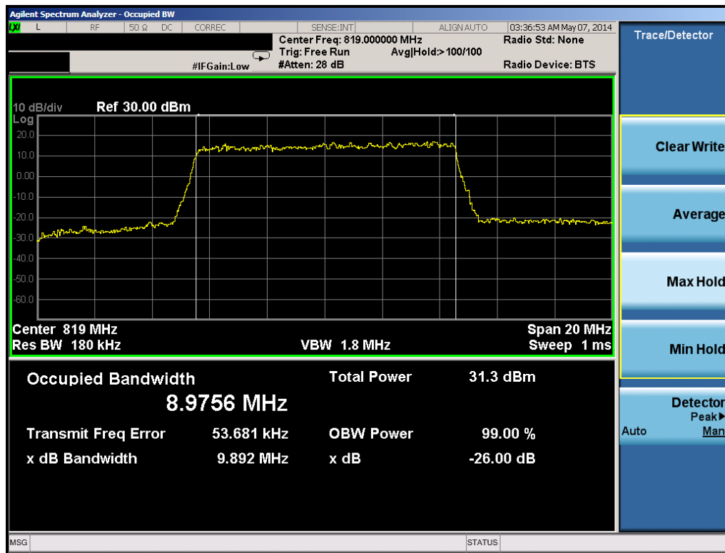
Plot 6-10. B26 Occupied Bandwidth Plot (10MHz 16-QAM – RB Size 50)
