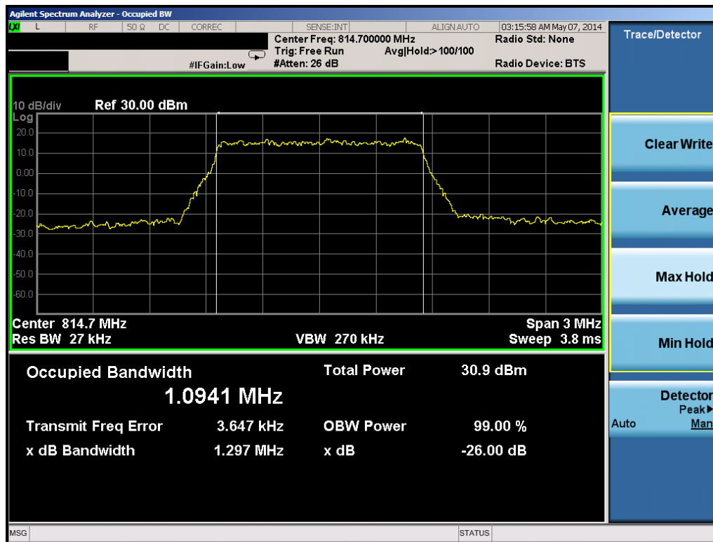
Plot 6-4. B26 Occupied Bandwidth Plot (1.4MHz 16-QAM – RB Size 6– Low Channel)
