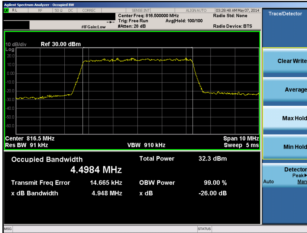
Plot 6-7. B26 Occupied Bandwidth Plot (5MHz QPSK – RB Size 25– Low Channel)
