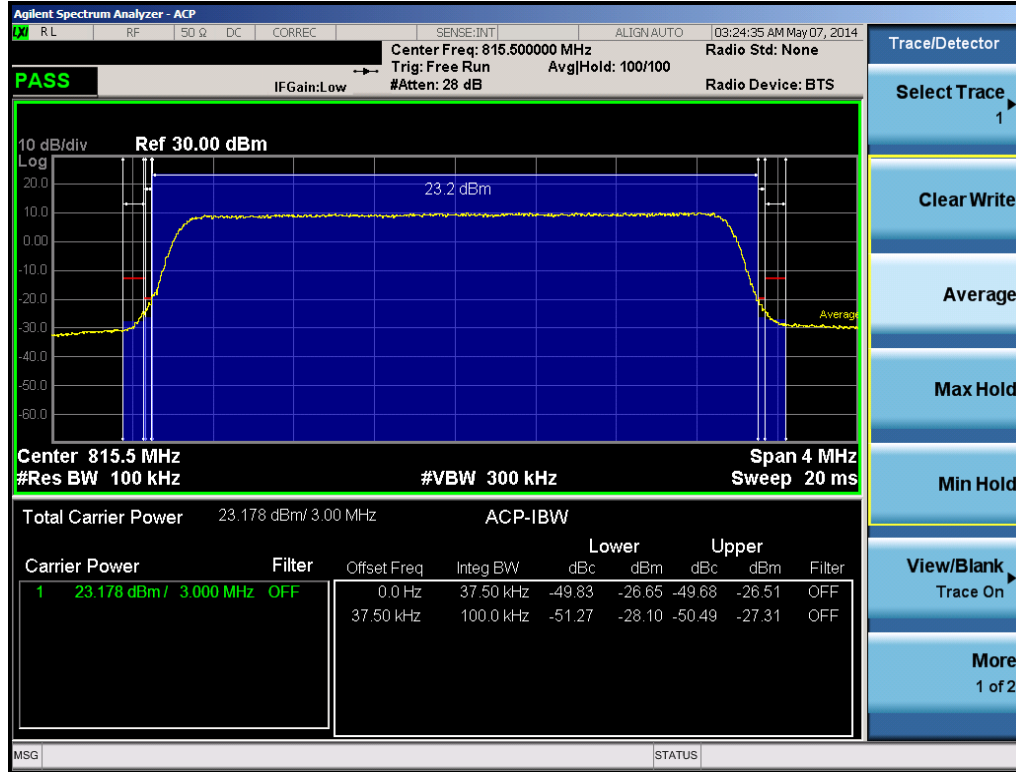
Plot 6-27. Channel Edge Plot (3MHz QPSK – RB Size 15– Low Channel)
