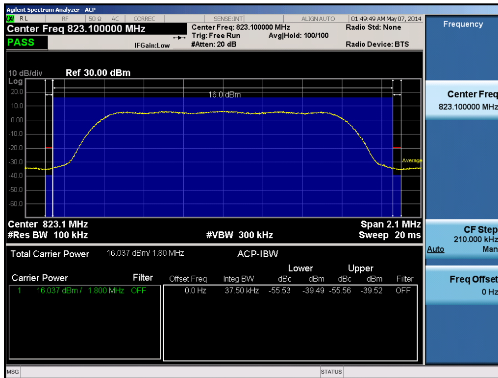
Plot 6-22. CDMA BC10 Channel Edge Plot (Ch. 684)
