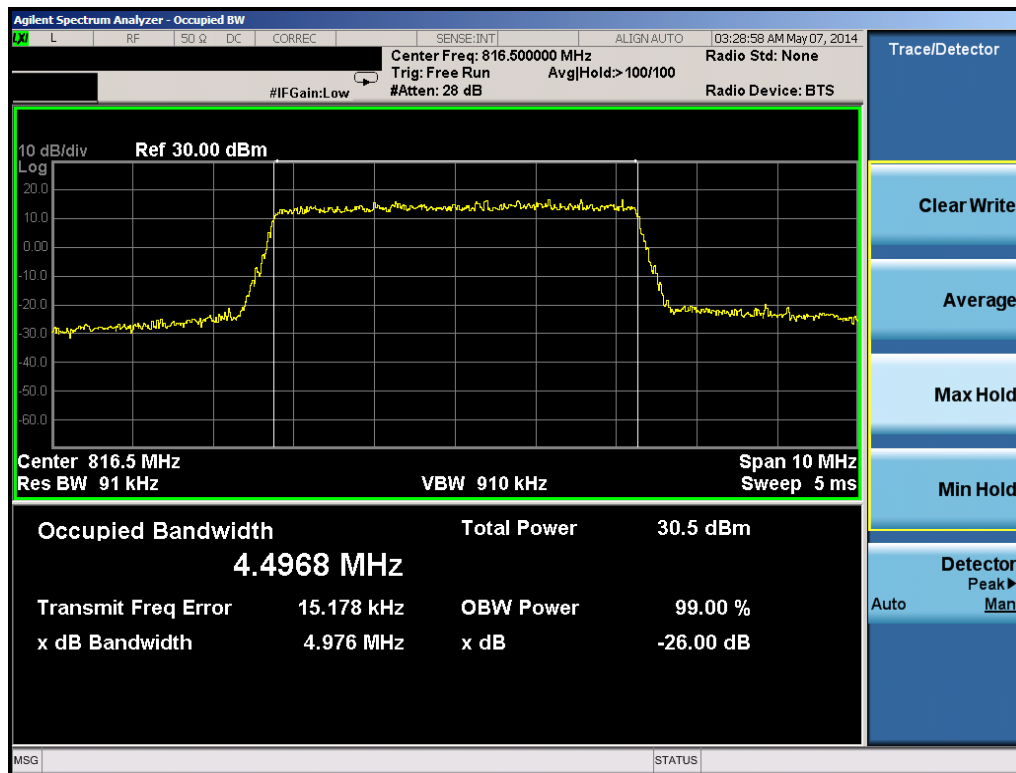
Plot 6-8. B26 Occupied Bandwidth Plot (5MHz 16-QAM – RB Size 25– Low Channel))
