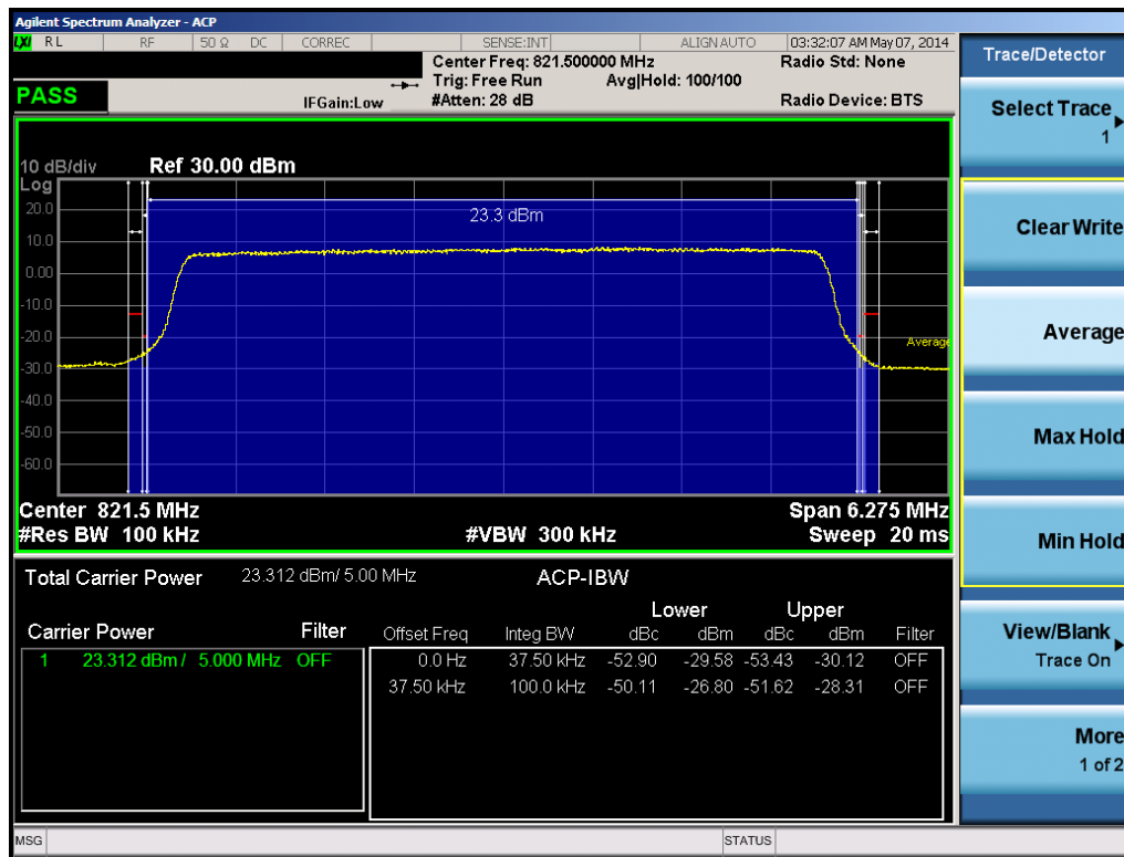
Plot 6-30. Channel Edge Plot (5MHz QPSK – RB Size 25 – High Channel)
