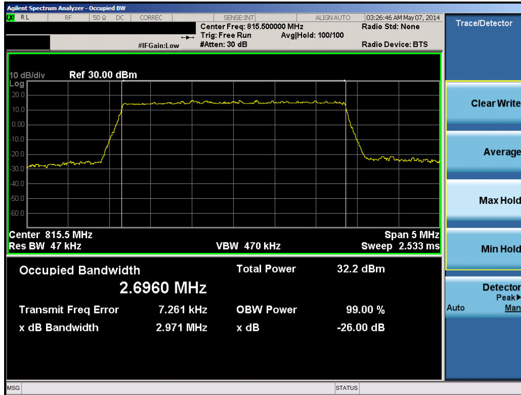
Plot 6-5. B26 Occupied Bandwidth Plot (3MHz QPSK – RB Size 15– Low Channel)
