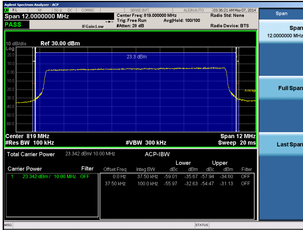
Plot 6-31. Channel Edge Plot (10MHz QPSK – RB Size 50)
