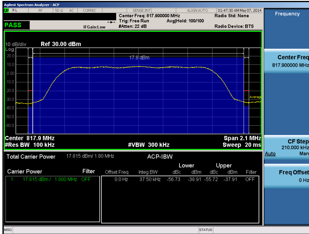
Plot 6-19. CDMA BC10 Channel Edge Plot (Ch. 476)
