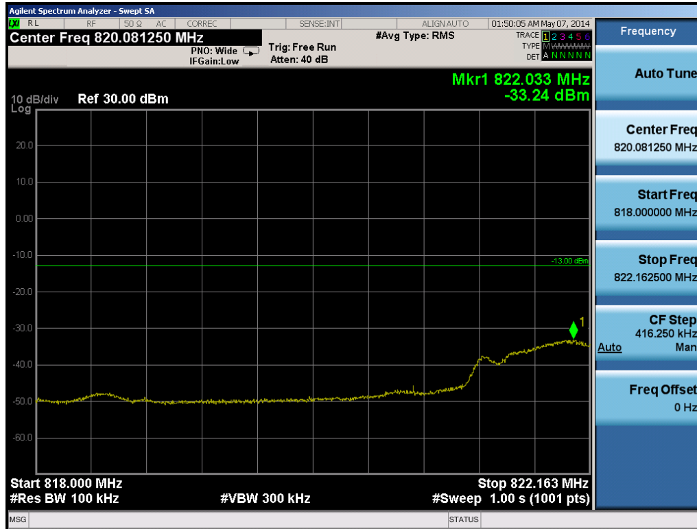
Plot 6-23. CDMA BC10 Inner Extended Band Edge Plot (Ch. 684)
