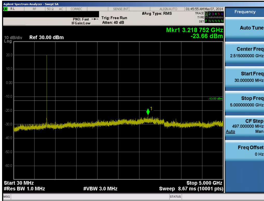
Plot 6-11. CDMA BC10 Conducted Spurious Plot (Ch. 476)
