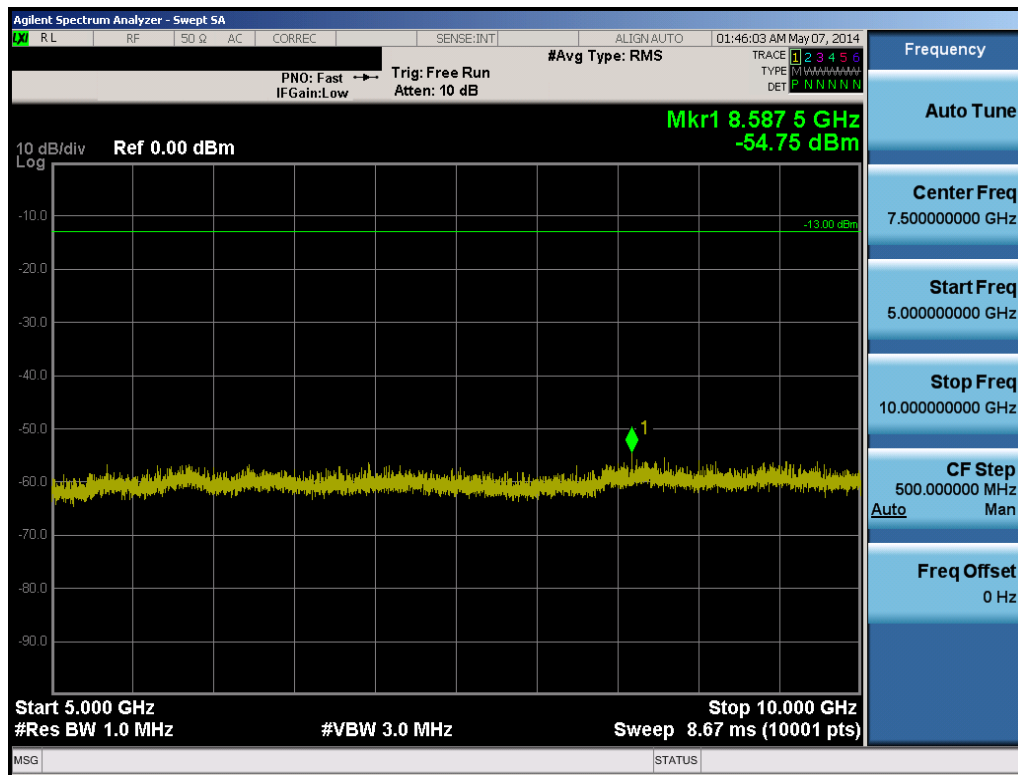
Plot 6-12. CDMA BC10 Conducted Spurious Plot (Ch. 476)
