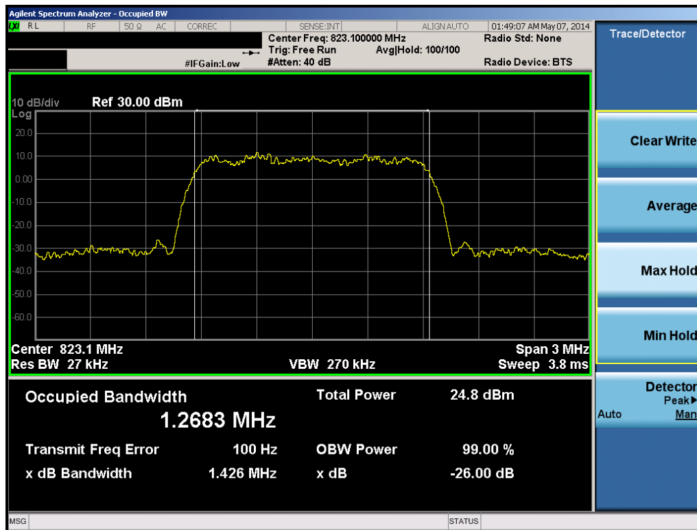
Plot 6-2. CDMA BC10 Occupied Bandwidth Plot (Ch. 684)
