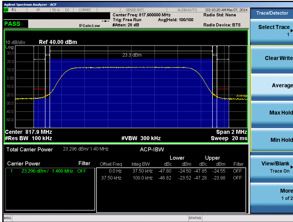
Plot 6-25. Channel Edge Plot (1.4MHz QPSK – RB Size 6– Low Channel)
