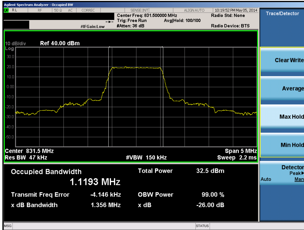
Plot 6-3. Occupied Bandwidth Plot (1.4MHz QPSK – RB Size 6– Low Channel)
