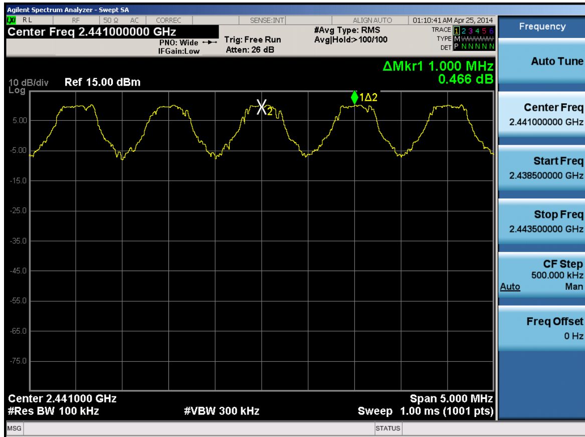
Plot 6-32. Channel Spacing Plot (Bluetooth)
