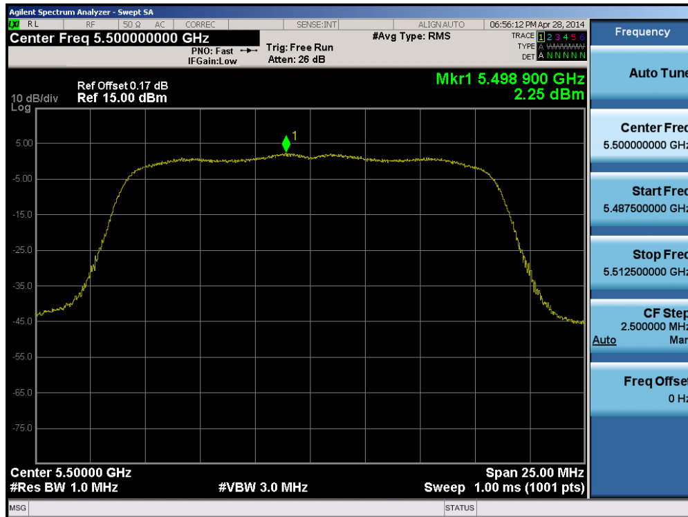
Plot 6-44. Peak Power Spectral Density Plot (802.11a (UNII Band 2C) – Ch. 100)
