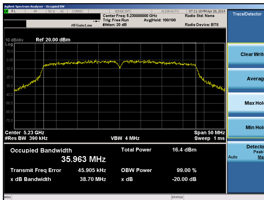
Plot 6-26. 20dB Bandwidth Plot (40MHz BW 802.11n (UNII Band 1) – Ch. 46)
