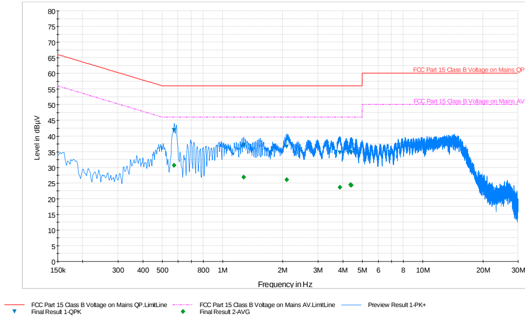
Plot 6-75. Line Conducted Plot with 802.11a UNII Band 2C (N)
