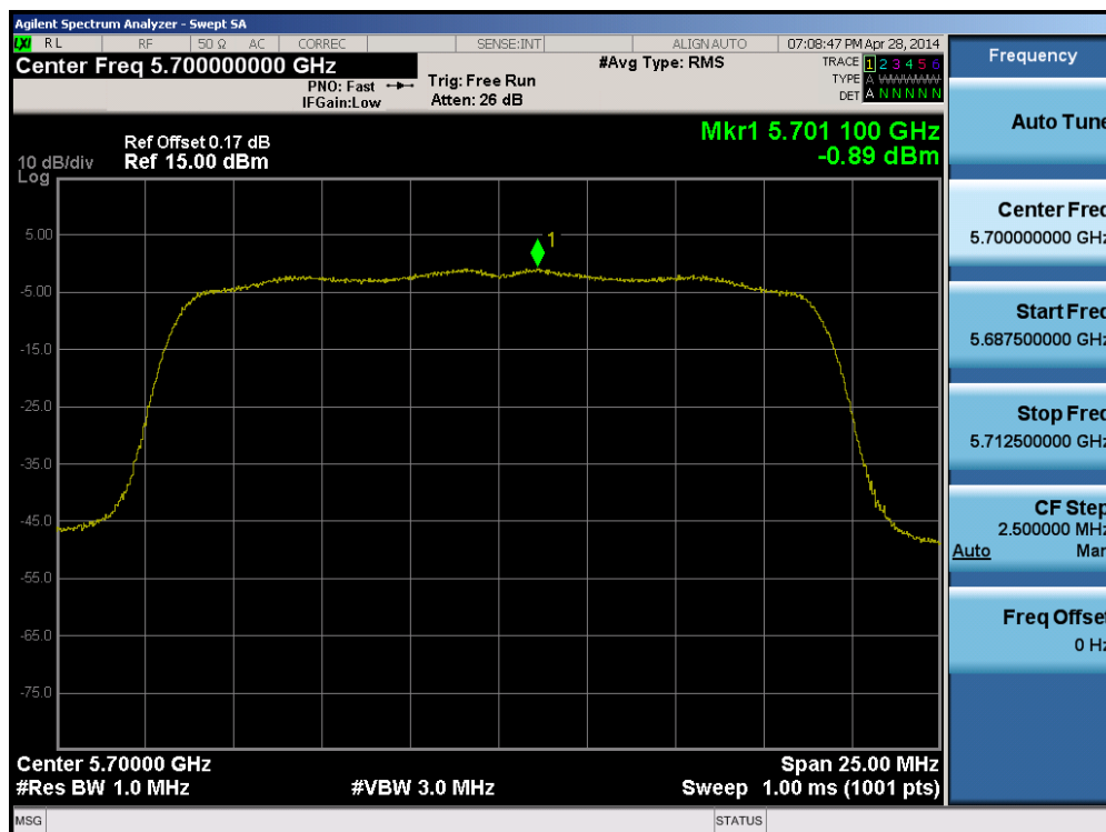
Plot 6-49. Peak Power Spectral Density Plot (20MHz BW 802.11n (UNII Band 2C) – Ch. 140)
