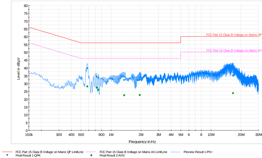
Plot 6-72. Line Conducted Plot with 802.11a UNII Band 2A (L1)
