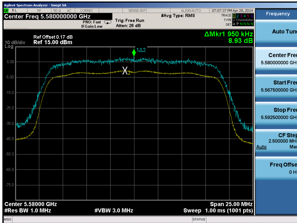
Plot 6-54. Peak Excursion Ratio Plot (20MHz BW 802.11n (UNII Band 2C) – Ch. 116)
