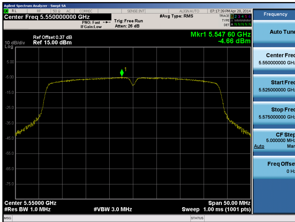
Plot 6-51. Peak Power Spectral Density Plot (40MHz BW 802.11n (UNII Band 2C) – Ch. 110)
