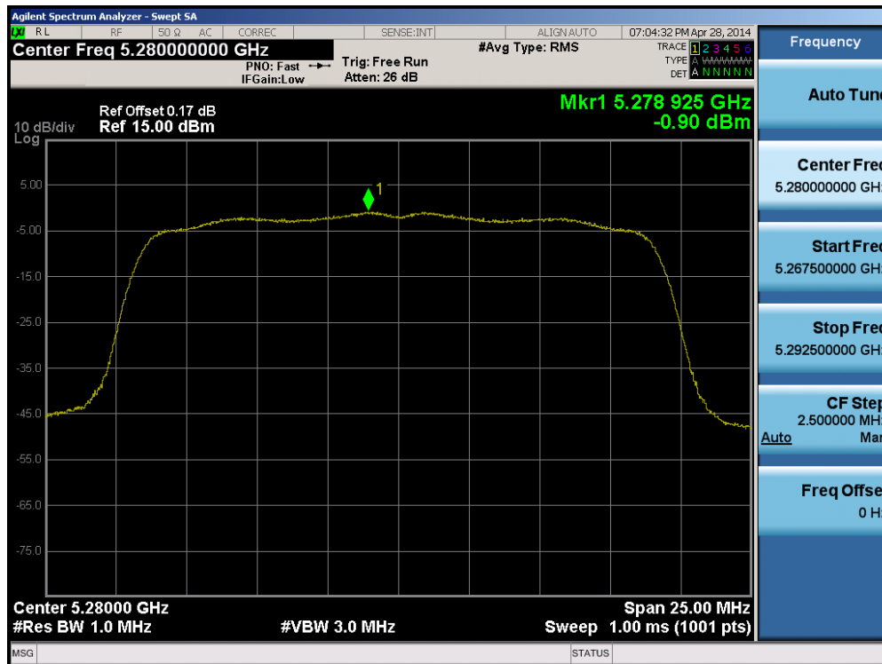
Plot 6-40. Peak Power Spectral Density Plot (20MHz BW 802.11n (UNII Band 2A) – Ch. 56)
