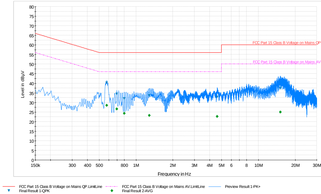
Plot 6-74. Line Conducted Plot with 802.11a UNII Band 2C (L1)
