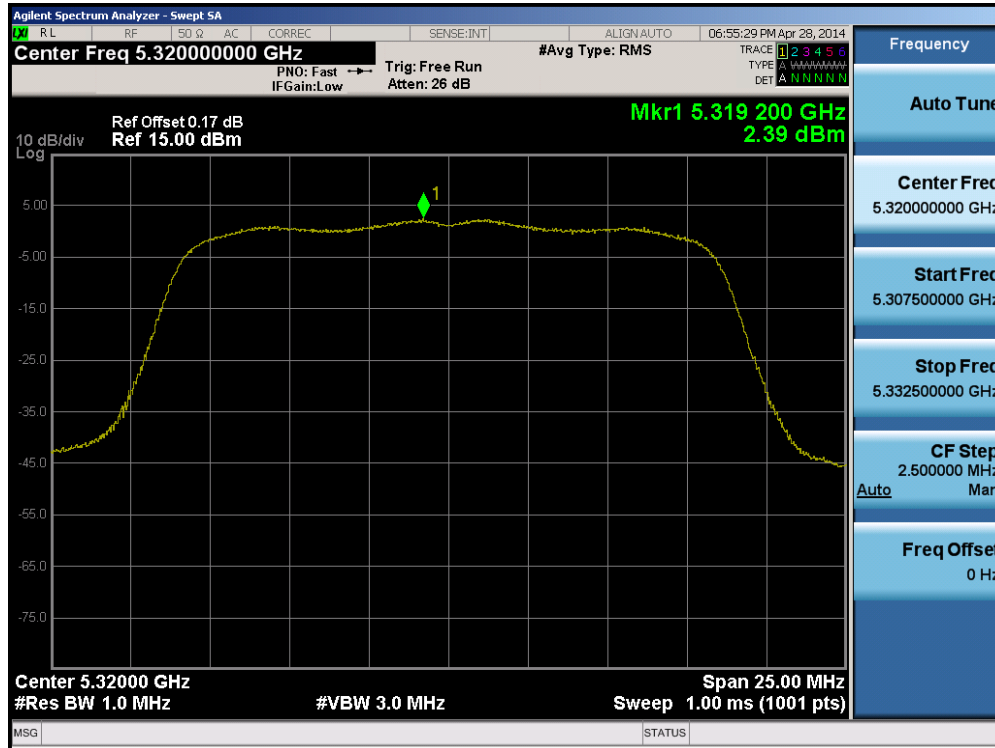
Plot 6-38. Peak Power Spectral Density Plot (802.11a (UNII Band 2A) – Ch. 64)
