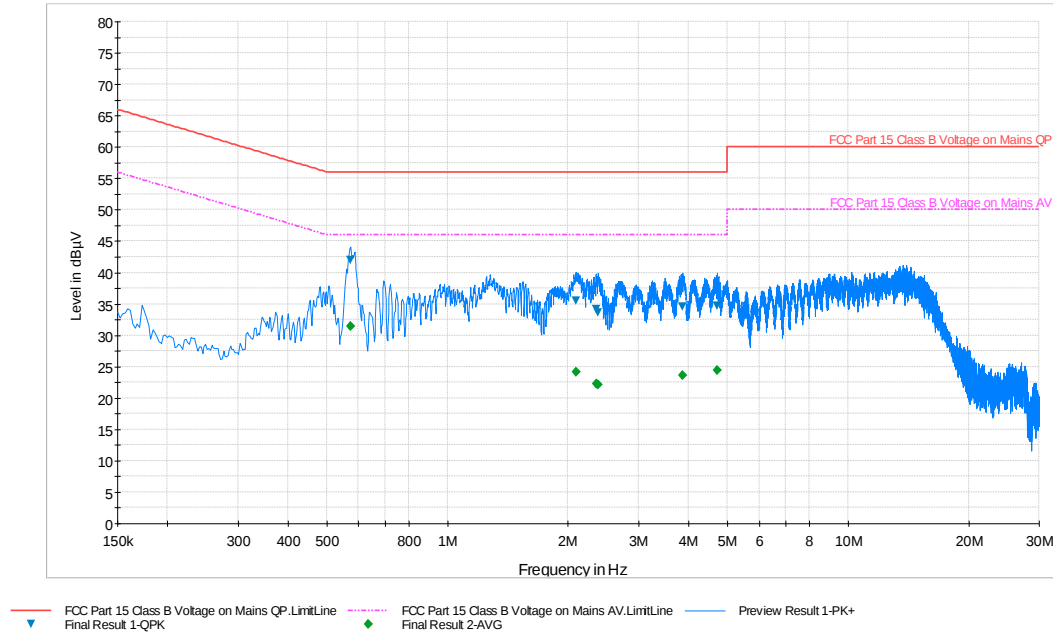
Plot 6-73. Line Conducted Plot with 802.11a UNII Band 2A (N)
