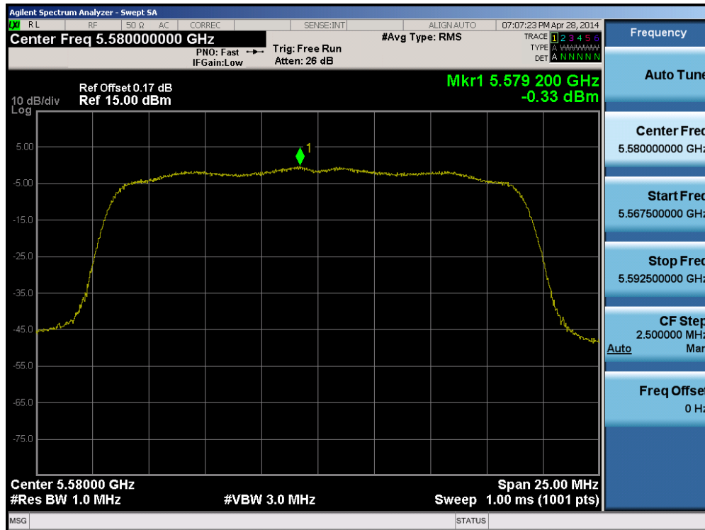
Plot 6-48. Peak Power Spectral Density Plot (20MHz BW 802.11n (UNII Band 2C) – Ch. 116)
