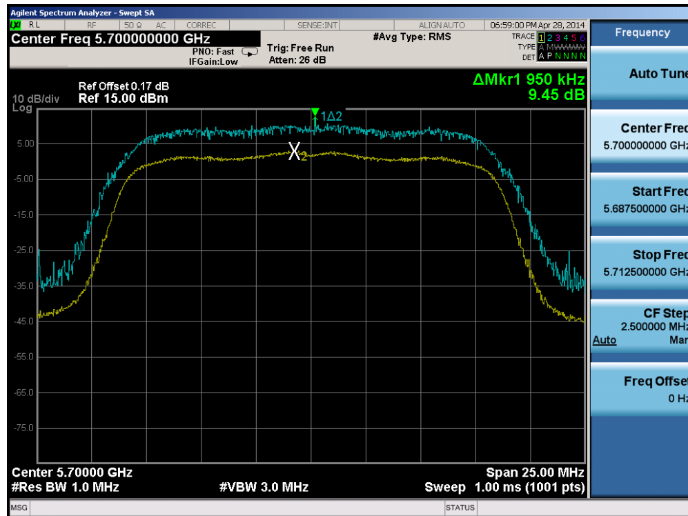
Plot 6-53. Peak Excursion Ratio Plot (802.11a (UNII Band 2C) – Ch. 140)
