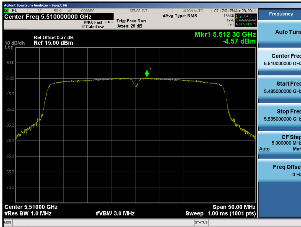
Plot 6-50. Peak Power Spectral Density Plot (40MHz BW 802.11n (UNII Band 2C) – Ch. 102)
