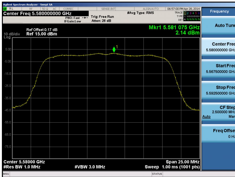
Plot 6-45. Peak Power Spectral Density Plot (802.11a (UNII Band 2C) – Ch. 116)
