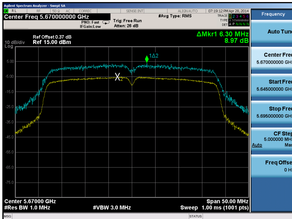
Plot 6-55. Peak Excursion Ratio Plot (40MHz BW 802.11n (UNII Band 2C) – Ch. 134)
