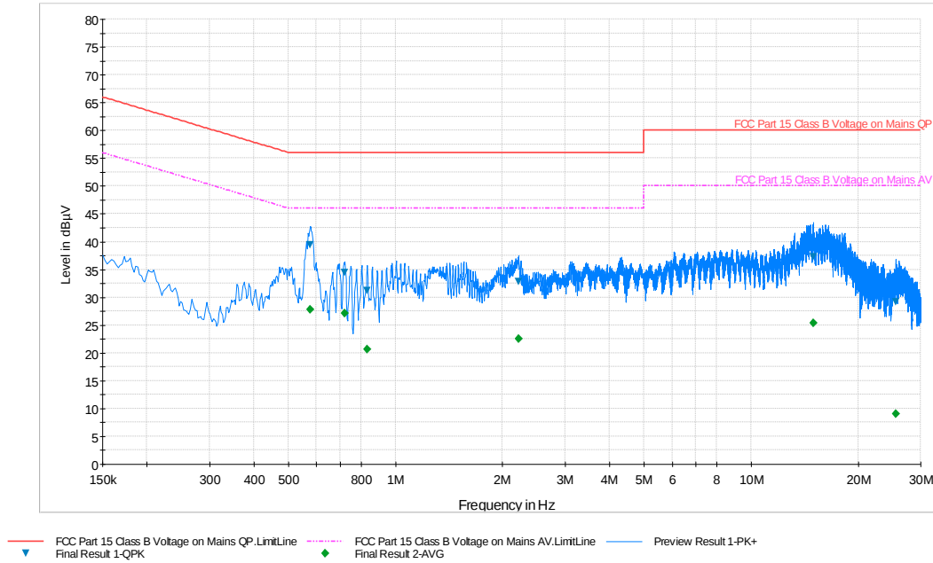
Plot 6-70. Line Conducted Plot with 802.11a UNII Band 1 (L1)
