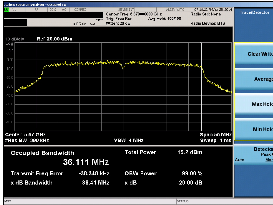
Plot 6-27. 20dB Bandwidth Plot (40MHz BW 802.11n (UNII Band 2C) – Ch. 134)
