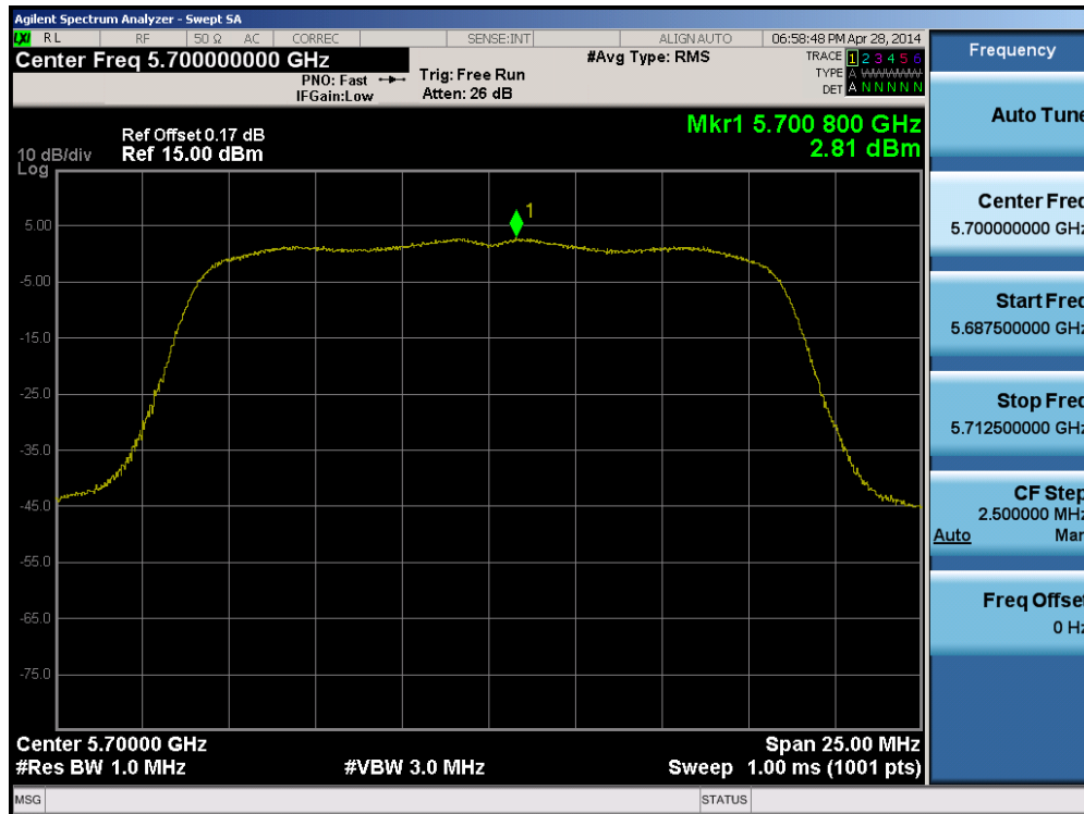
Plot 6-46. Peak Power Spectral Density Plot (802.11a (UNII Band 2C) – Ch. 140)
