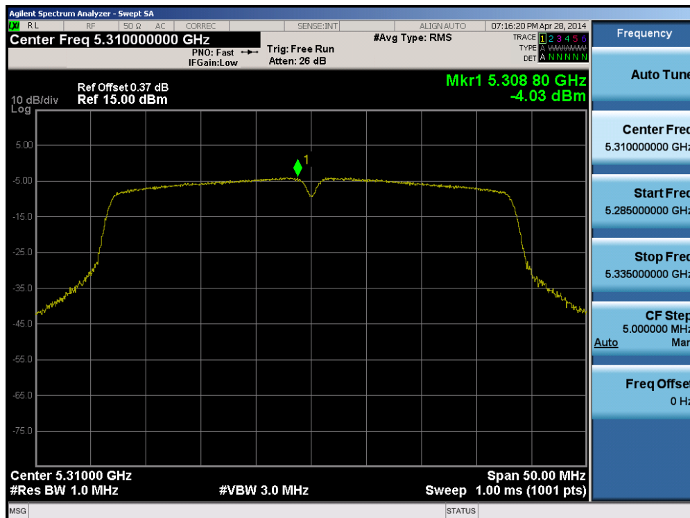
Plot 6-43. Peak Power Spectral Density Plot (40MHz BW 802.11n (UNII Band 2A) – Ch. 62)
