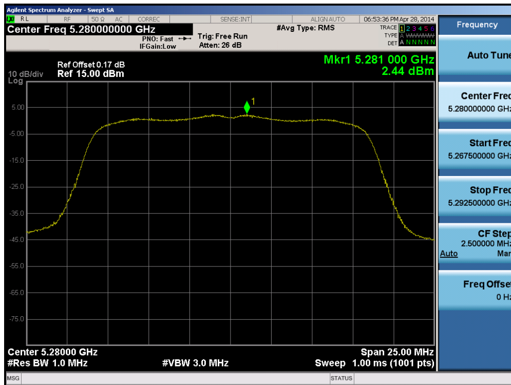
Plot 6-37. Peak Power Spectral Density Plot (802.11a (UNII Band 2A) – Ch. 56)
