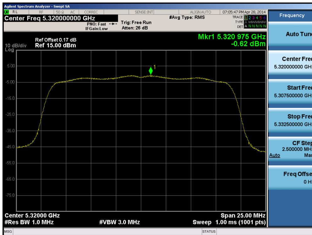
Plot 6-41. Peak Power Spectral Density Plot (20MHz BW 802.11n (UNII Band 2A) – Ch. 64)
