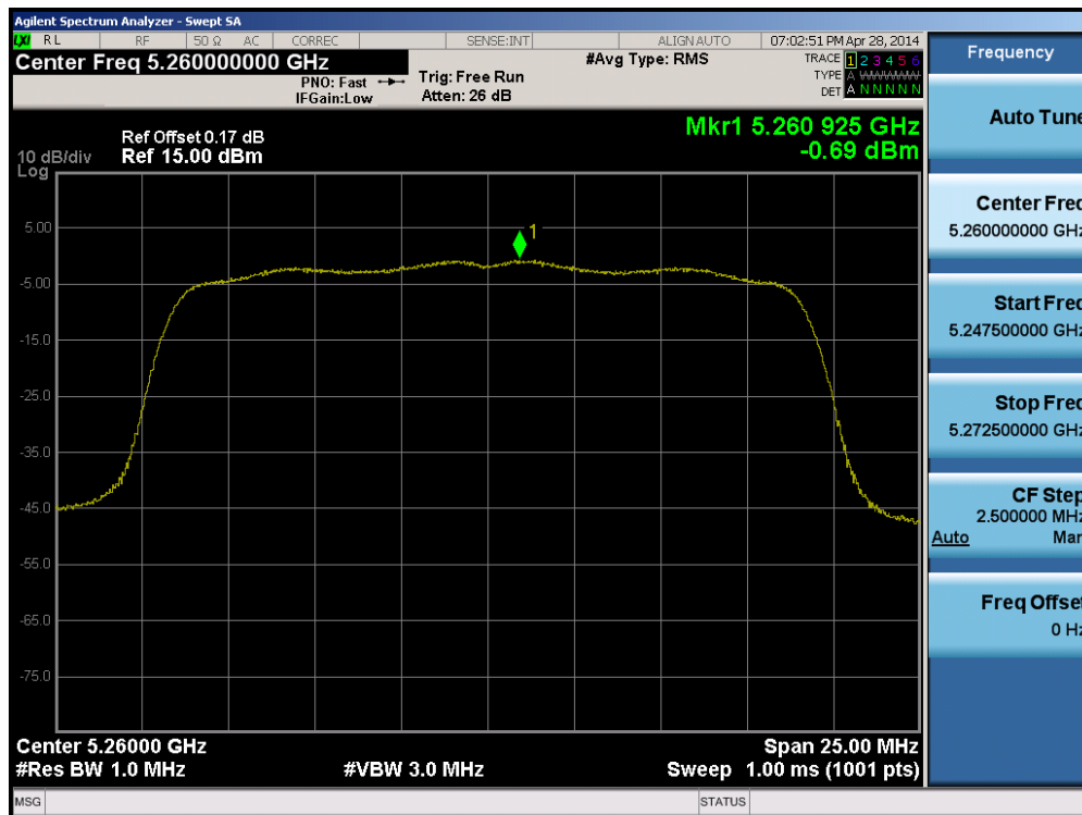
Plot 6-39. Peak Power Spectral Density Plot (20MHz BW 802.11n (UNII Band 2A) – Ch. 52)
