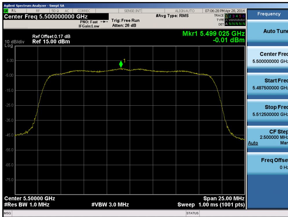
Plot 6-47. Peak Power Spectral Density Plot (20MHz BW 802.11n (UNII Band 2C) – Ch. 100)
