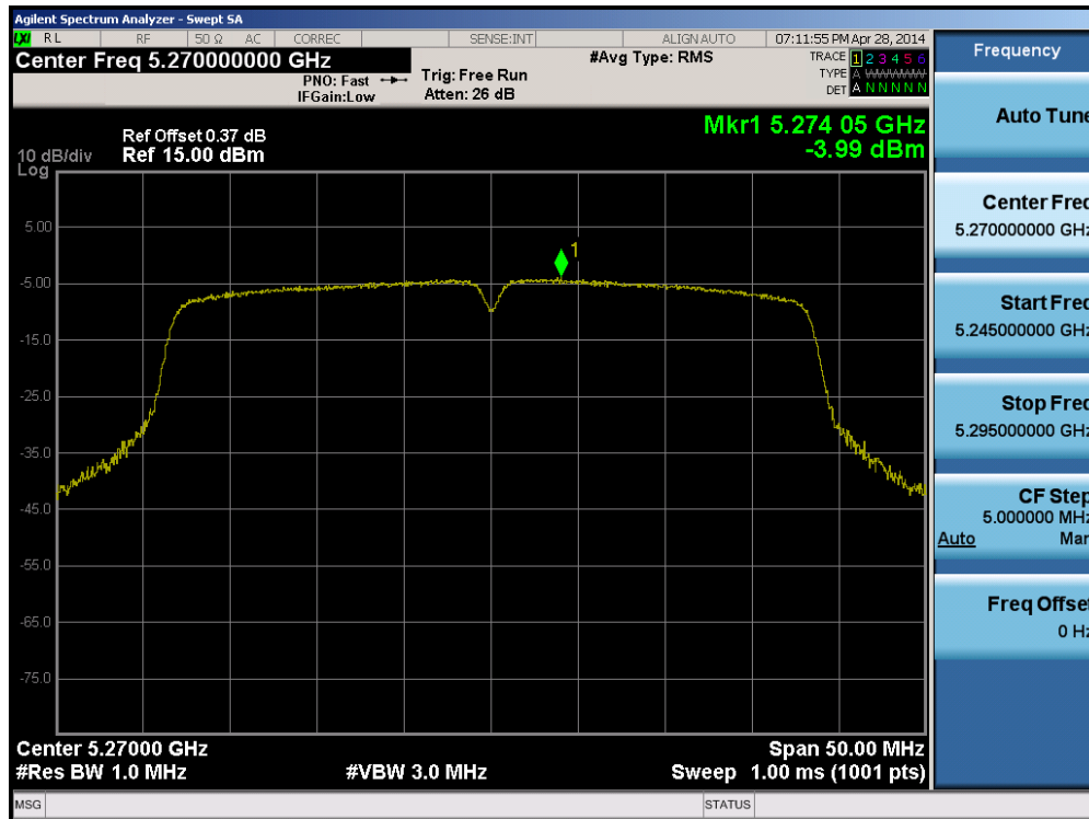
Plot 6-42. Peak Power Spectral Density Plot (40MHz BW 802.11n (UNII Band 2A) – Ch. 54)
