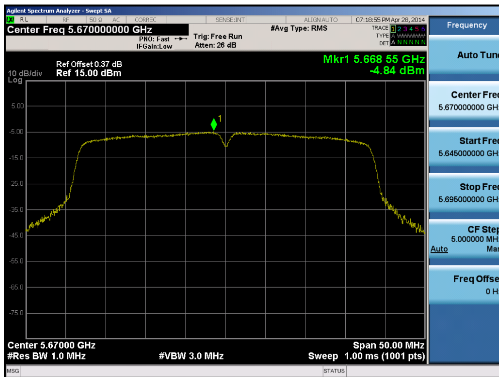
Plot 6-52. Peak Power Spectral Density Plot (40MHz BW 802.11n (UNII Band 2C) – Ch. 134)
