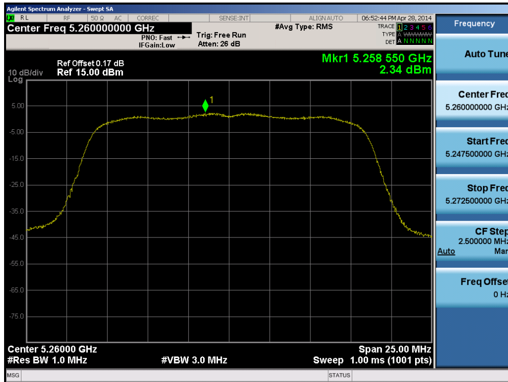
Plot 6-36. Peak Power Spectral Density Plot (802.11a (UNII Band 2A) – Ch. 52)
