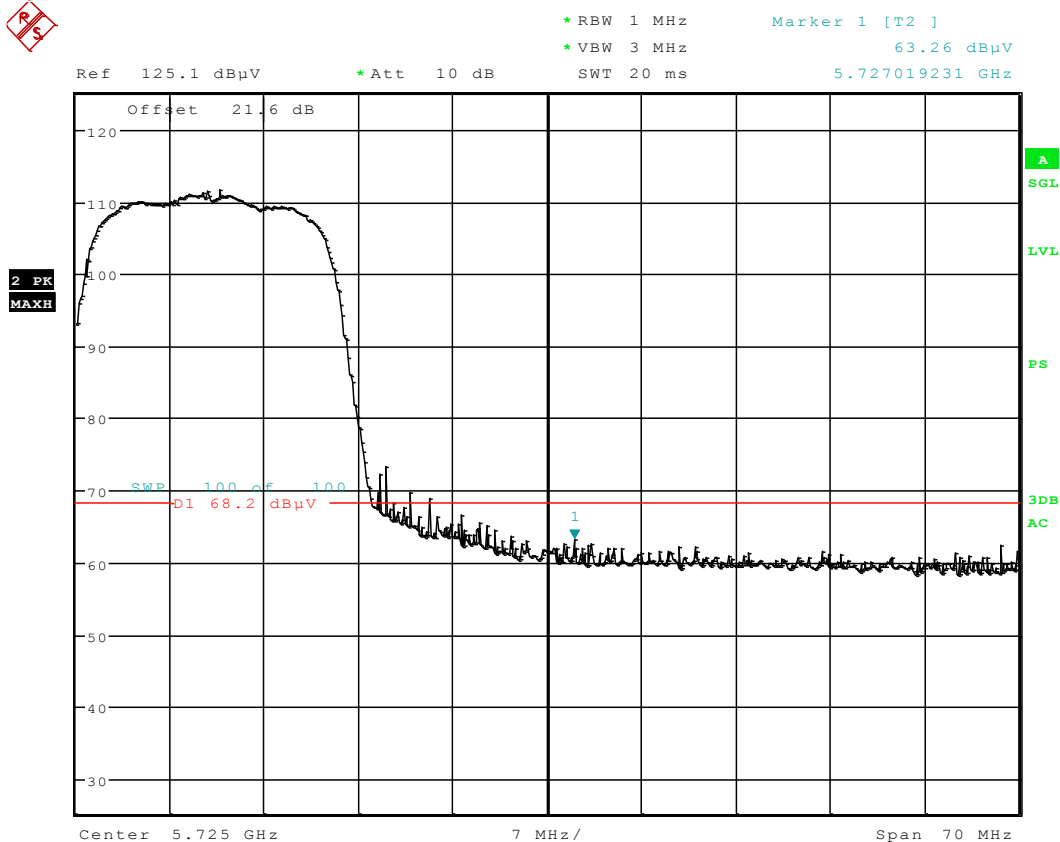
Plot 6-7. Radiated Upper Band Edge Plot (Peak – UNII Band 2C)
