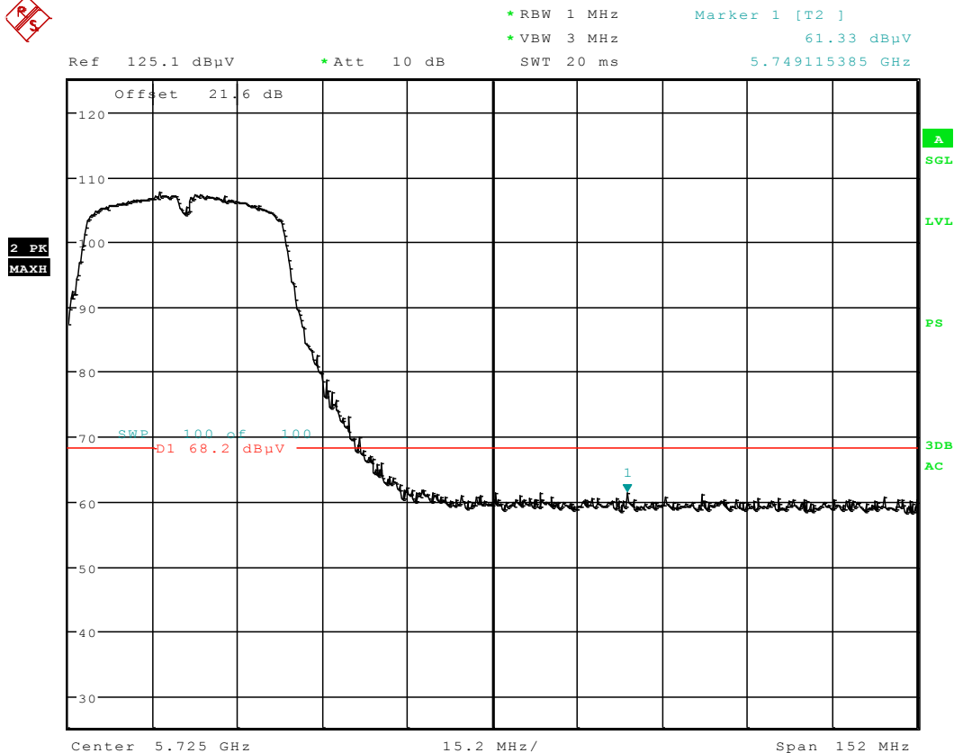
Plot 6-14. Radiated Upper Band Edge Plot (Peak – UNII Band 2C)
