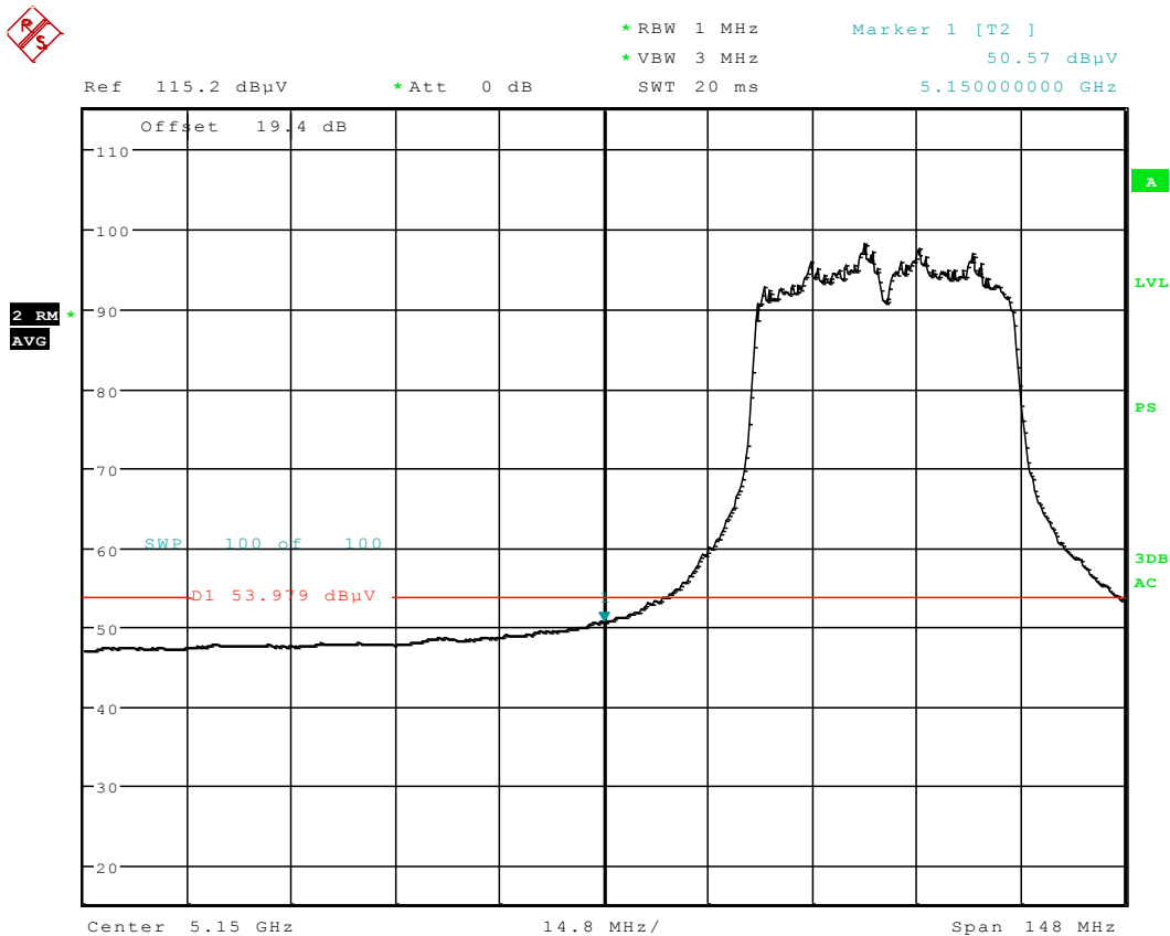
Plot 6-8. Radiated Restricted Lower Band Edge Plot (Average – UNII Band 1)
