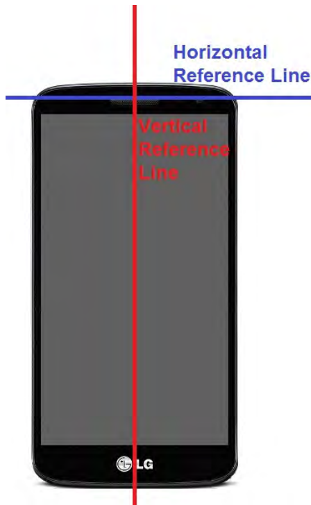
SAR Test Setup Photo 11: Vertical and Horizontal Reference Lines
