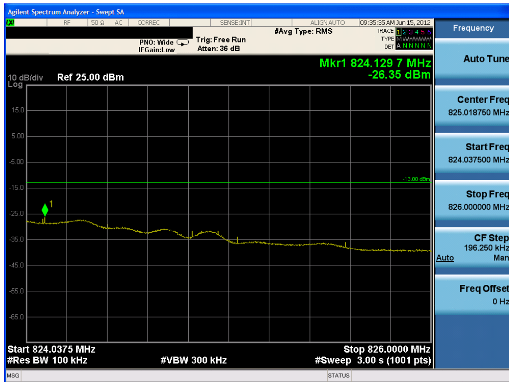
Plot 7-8. Extended Band Edge Plot (Ch. 684)
