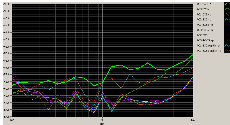
Figure 6-2 CDMA Audio Band Magnetic Noise
