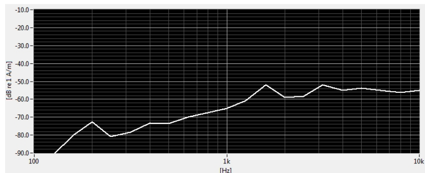
Figure 7-2 Worst-case ABM2 Plot for UMTS
