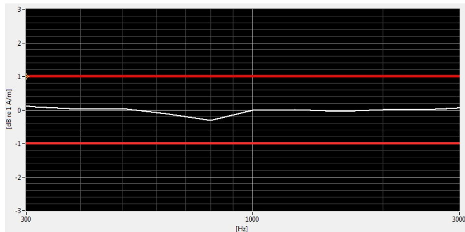
Figure 7-4 Helmholtz Coil Validation for Frequency Response
