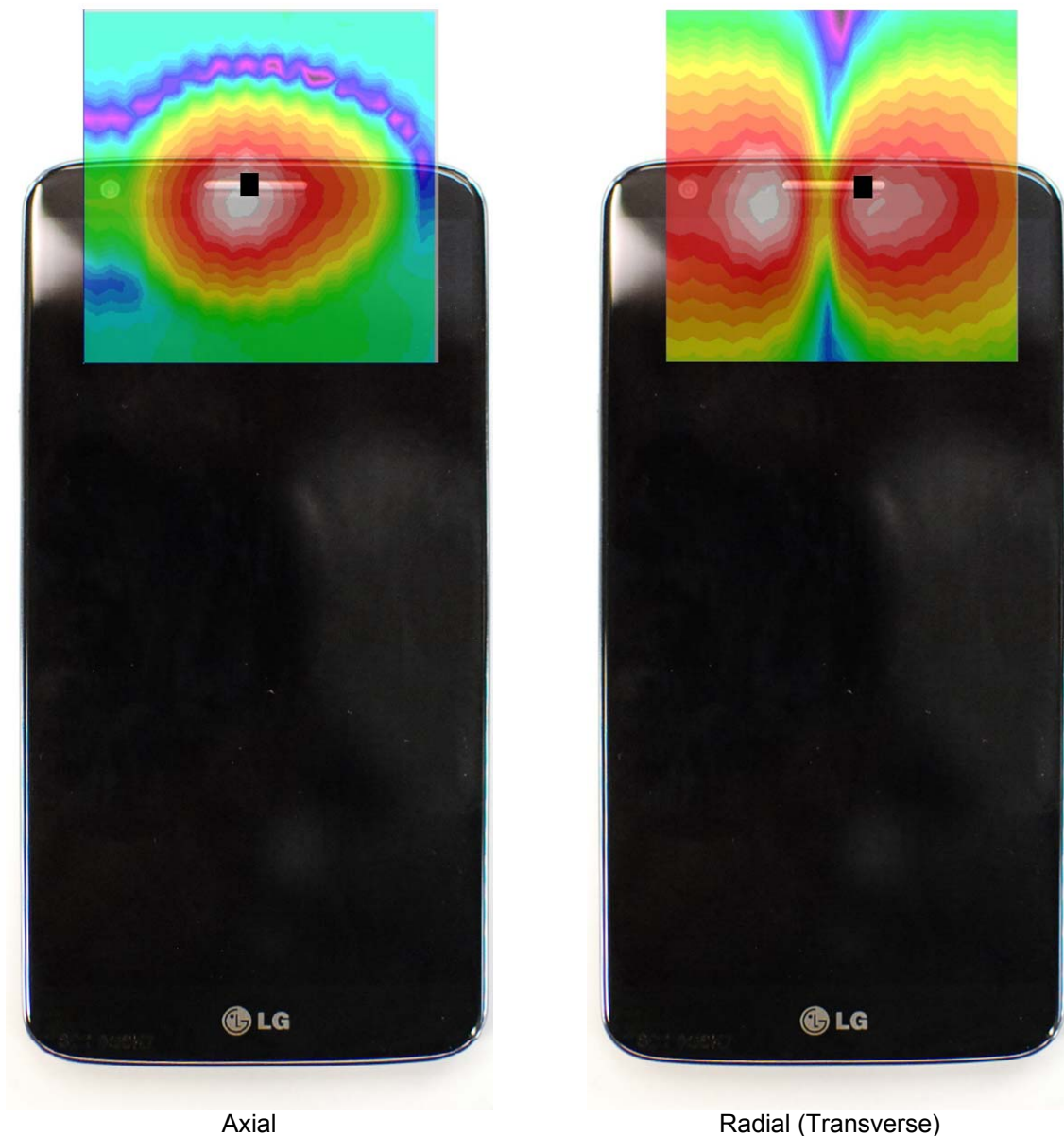
Figure 13-3 T-Coil Scan Overlay Magnetic Field Distributions
