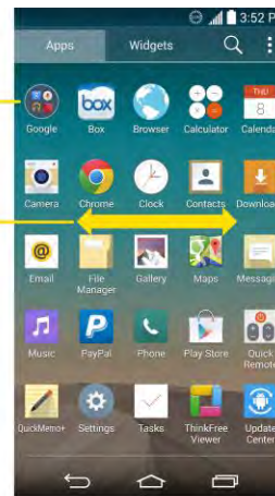
Applications screen
