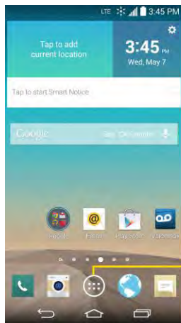
Home screen
