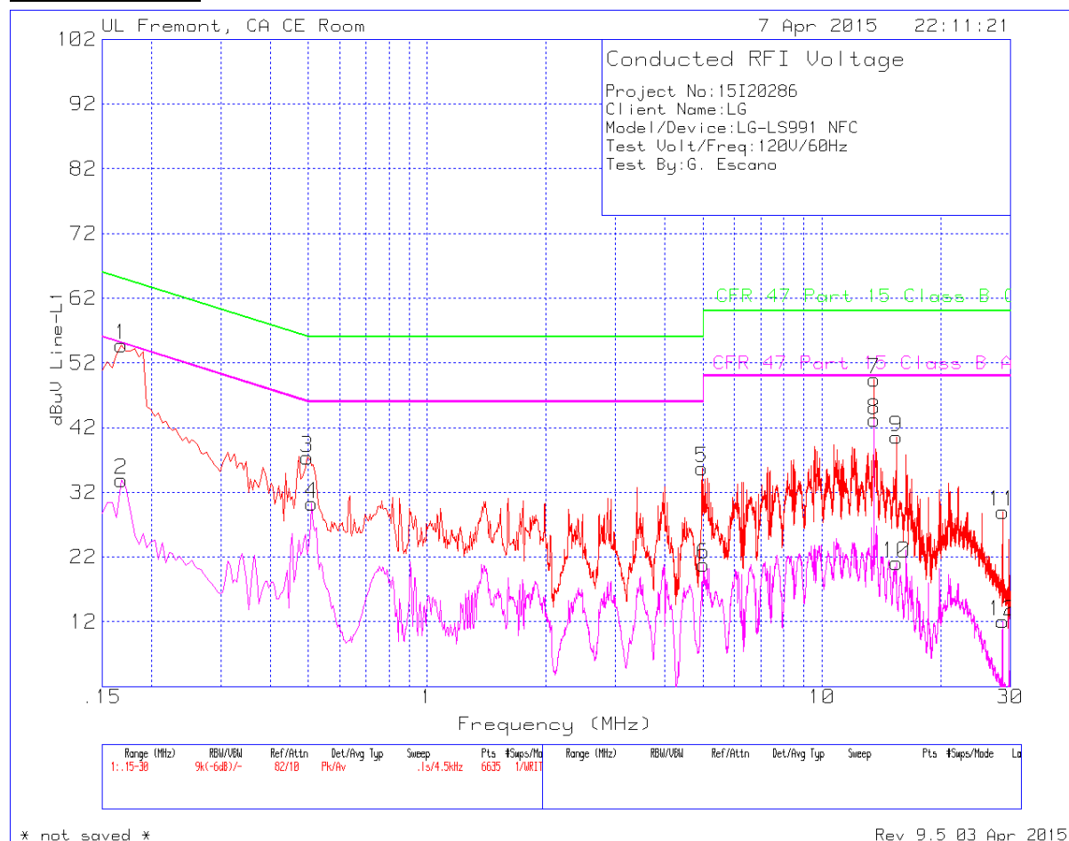
Range 1: Line-L1 .15 - 30MHz
