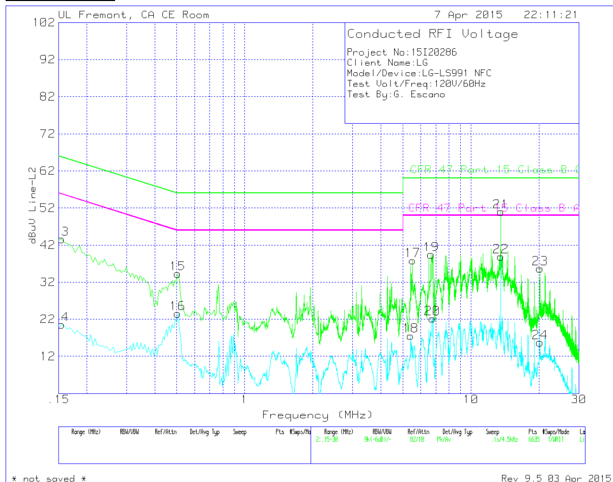
Range 2: Line-L2 .15 - 30MHz
