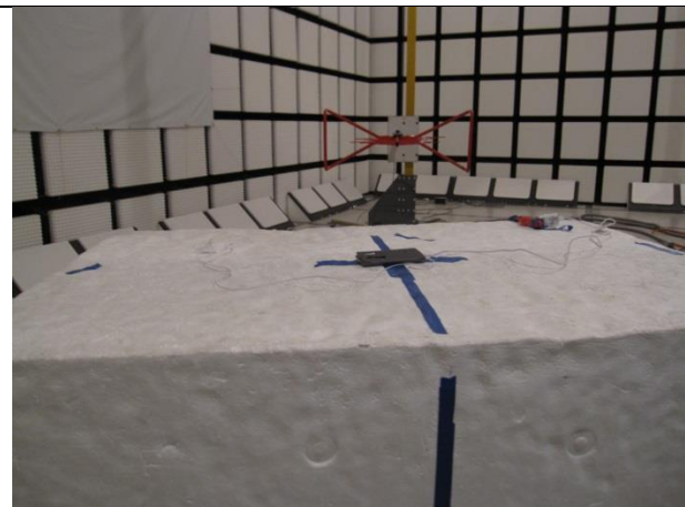
RADIATED EMISSION PHOTO
