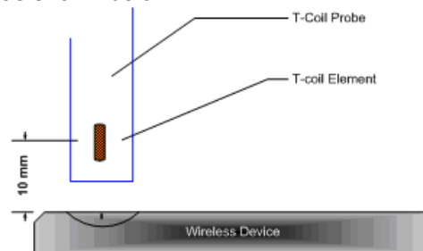
Figure 5-11 Measurement Distance
