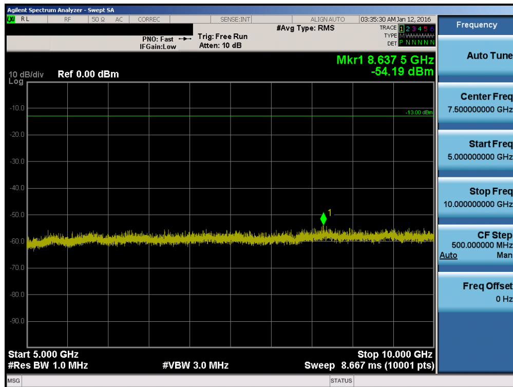
Plot 7-16. Conducted Spurious Plot LTE Band 26 (10MHz QPSK – RB Size 1, RB Offset 0)
