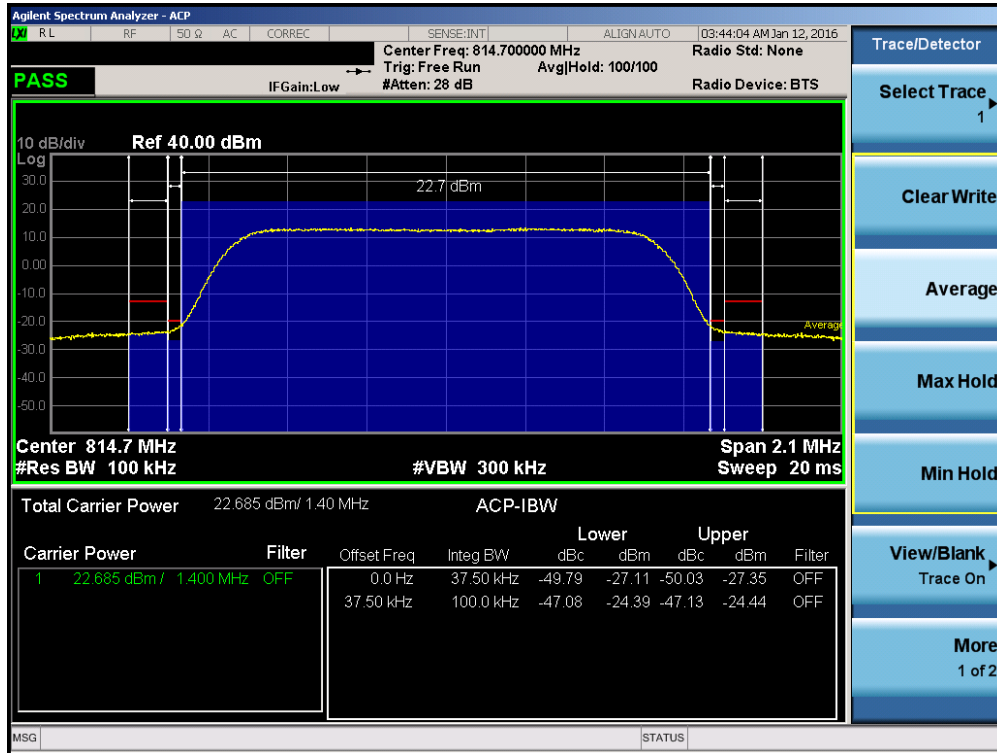
Plot 7-19. Channel Edge Plot LTE Band 26 (1.4MHz - RB Size 6- Low Channel)
