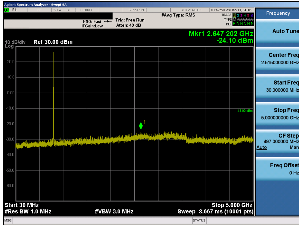
Plot 7-13. Conducted Spurious Plot CDMA BC10 (Ch. 684)
