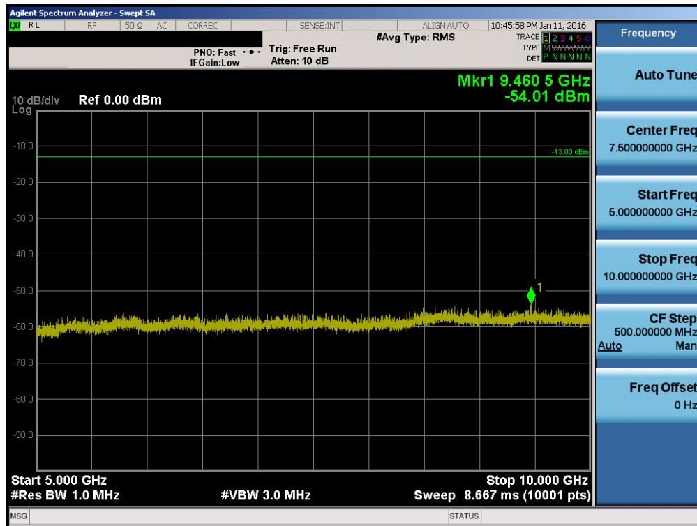
Plot 7-12. Conducted Spurious Plot CDMA BC10 (Ch. 476)
