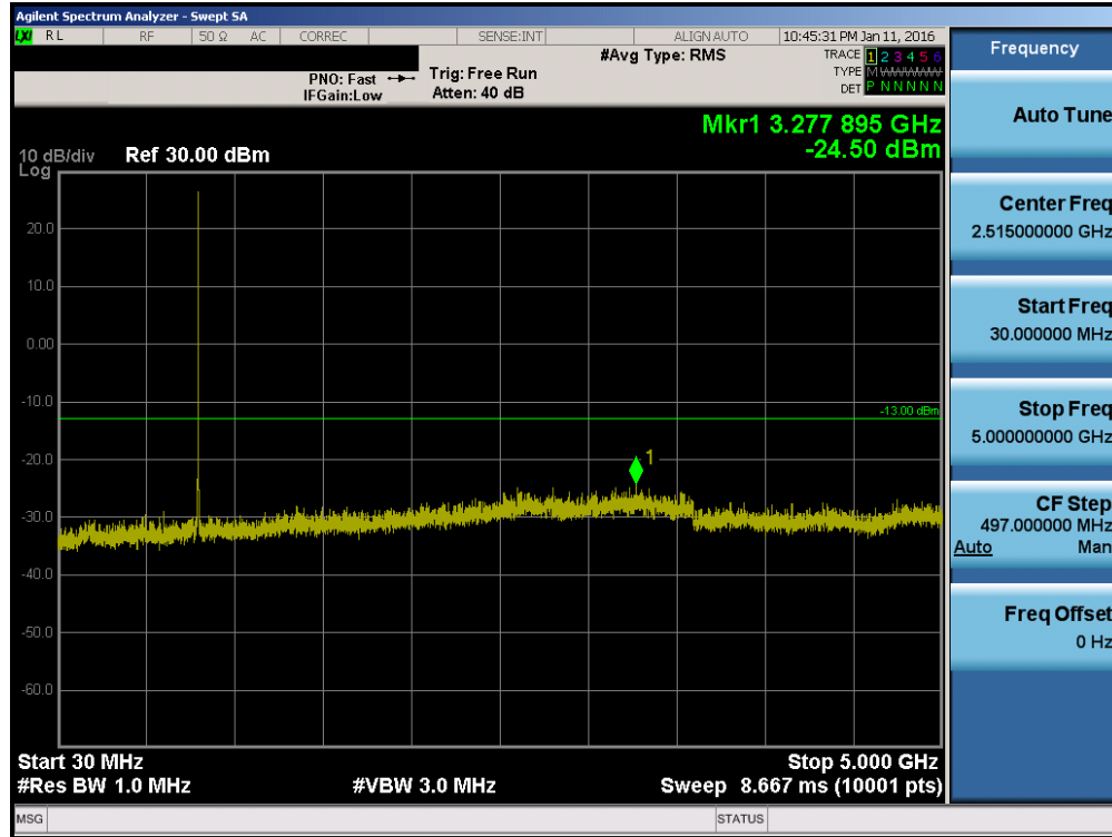
Plot 7-11. Conducted Spurious Plot CDMA BC10 (Ch. 476)
