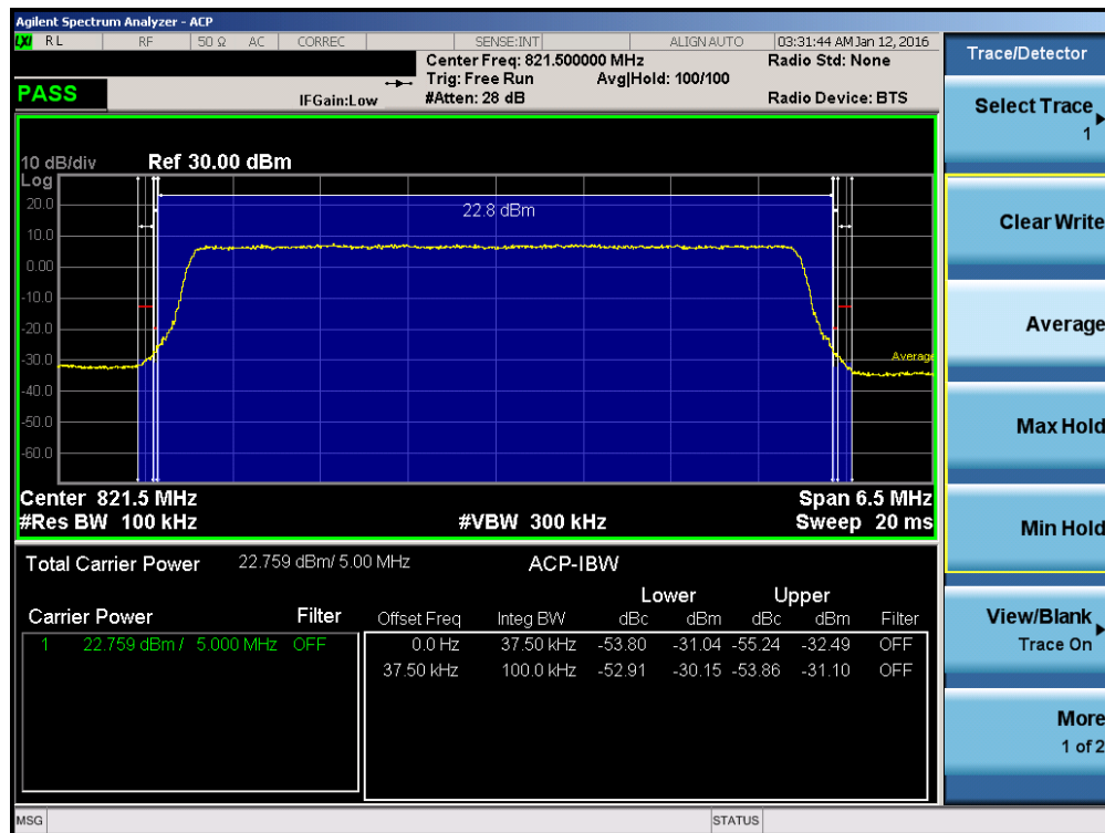
Plot 7-24. Channel Edge Plot LTE Band 26 (5MHz – RB Size 25 – High Channel)
