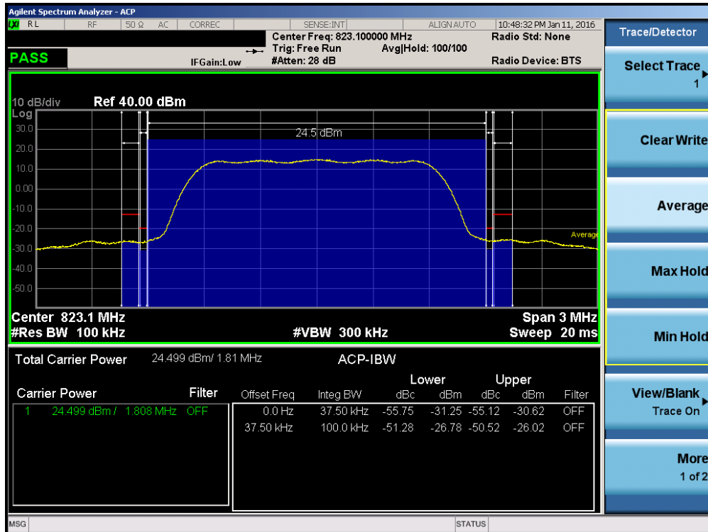
Plot 7-18. Channel Edge Plot CDMA BC10 (Ch. 684)
