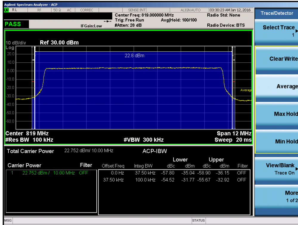
Plot 7-25. Channel Edge Plot LTE Band 26 (10MHz – RB Size 50)
