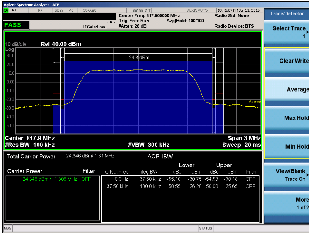
Plot 7-17. Channel Edge Plot CDMA BC10 (Ch. 476)
