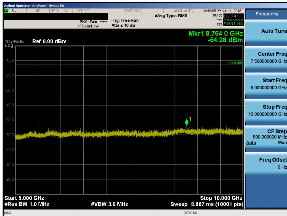
Plot 7-14. Conducted Spurious Plot CDMA BC10 (Ch. 684)
