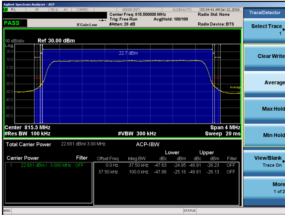
Plot 7-21. Channel Edge Plot LTE Band 26 (3MHz - RB Size 15- Low Channel)
