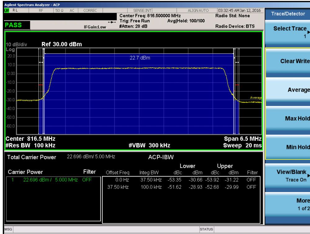
Plot 7-23. Channel Edge Plot LTE Band 26 (5MHz – RB Size 25– Low Channel)
