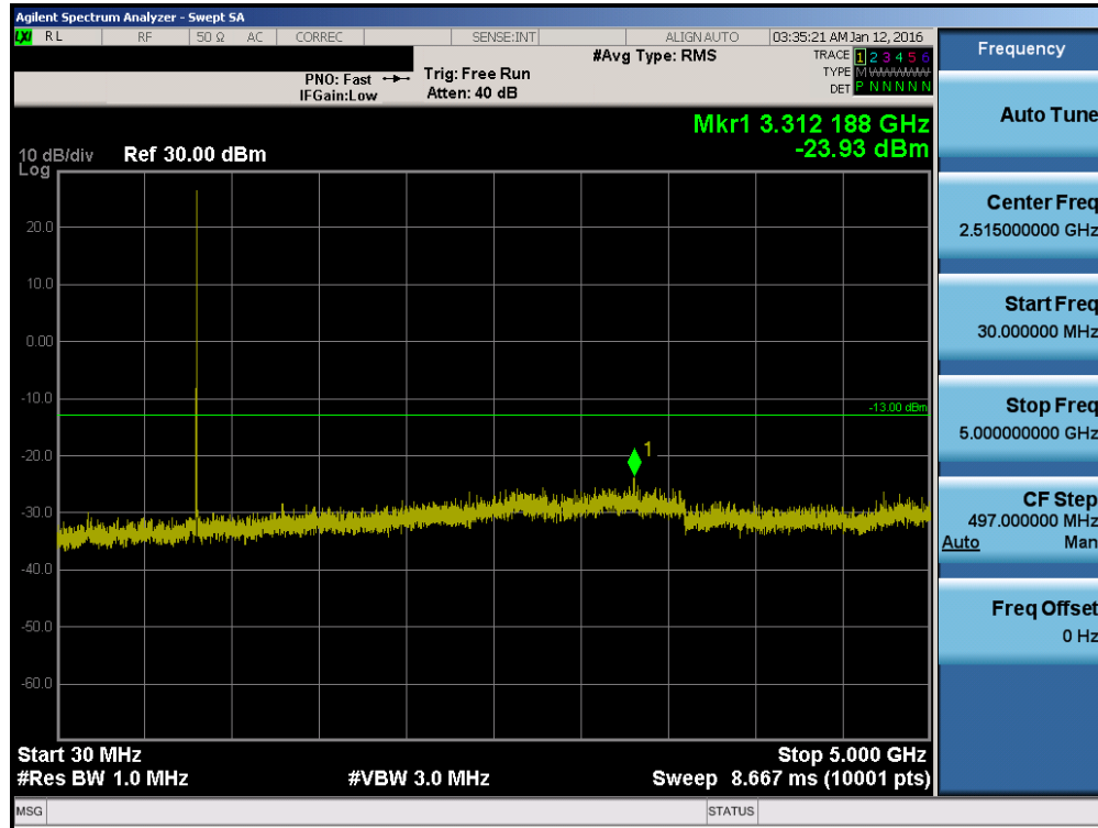
Plot 7-15. Conducted Spurious Plot LTE Band 26 (10MHz QPSK – RB Size 1, RB Offset 0)
