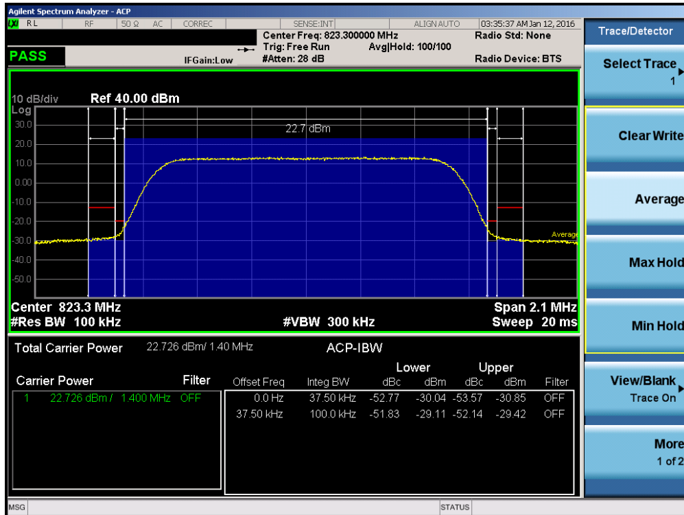
Plot 7-20. Channel Edge Plot LTE Band 26 (1.4MHz - RB Size 6 - High Channel)
