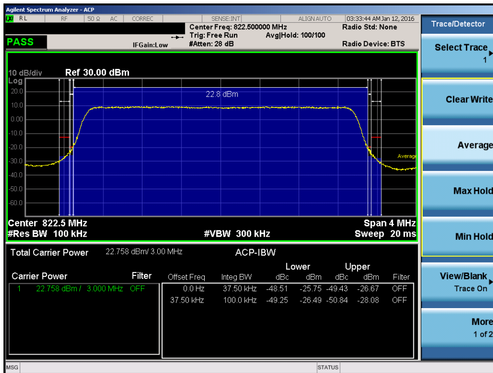
Plot 7-22. Channel Edge Plot LTE Band 26 (3MHz - RB Size 15 - High Channel)
