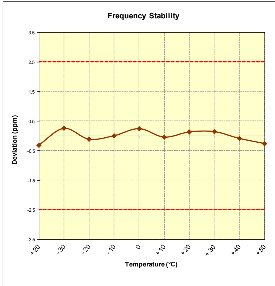
Figure 7-5. CDMA BC10 Frequency Stability Graph (Ch. 670)
