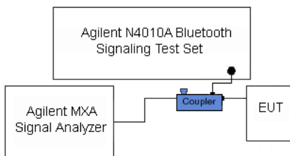
Figure 7-2. Test Instrument & Measurement Setup
