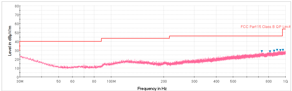
Plot 7-105. Radiated Spurious Plot below 1GHz (802.11a – U3 Ch. 157, Ant. Pol. V)
