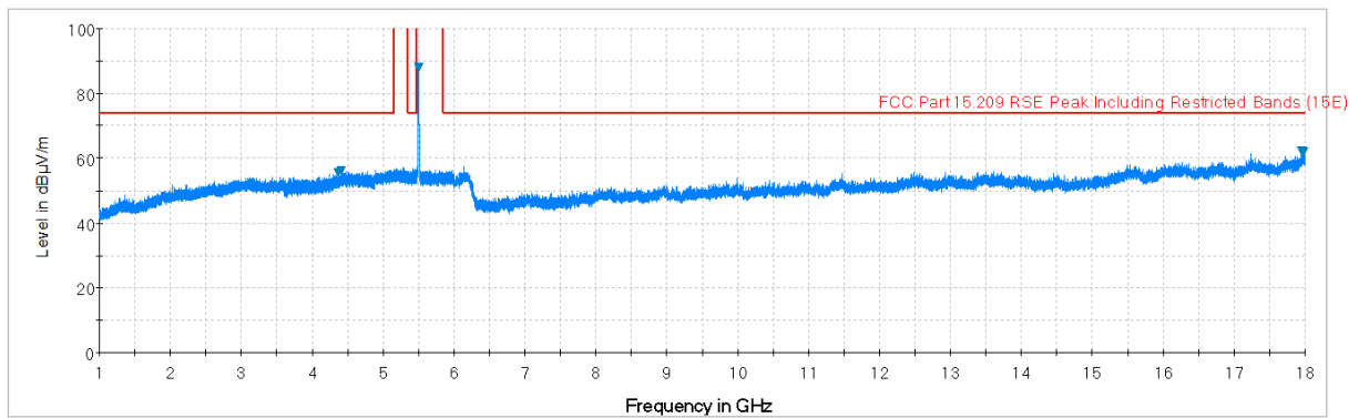
Plot 7-81. Radiated Spurious Plot above 1GHz (802.11a – U2C Ch. 116, Ant. Pol. H)
