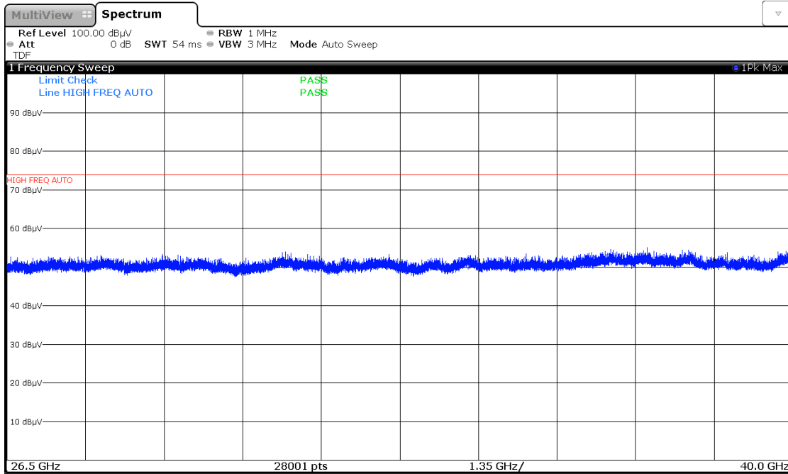
Plot 7-87. Radiated Spurious Plot above 26.5GHz (802.11a – Ant. Pol. H)
