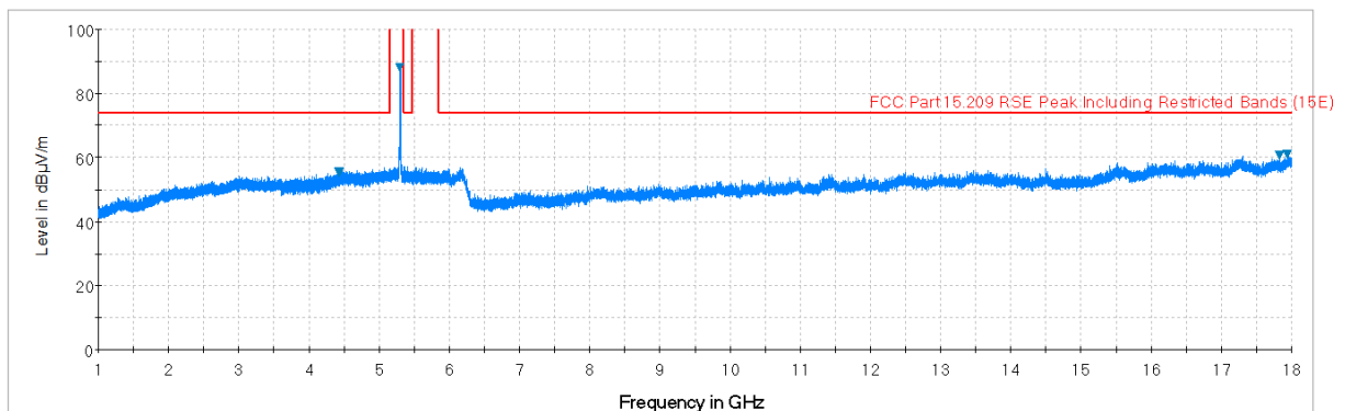
Plot 7-79. Radiated Spurious Plot above 1GHz (802.11a – U2A Ch. 56, Ant. Pol. H)
