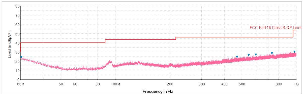
Plot 7-104. Radiated Spurious Plot below 1GHz (802.11a – U3 Ch. 157, Ant. Pol. H)
