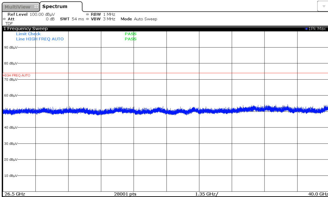
Plot 7-88. Radiated Spurious Plot above 26.5GHz (802.11a – Ant. Pol. V)
