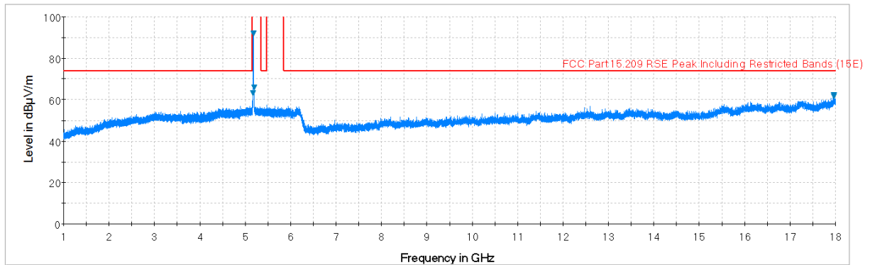
Plot 7-77. Radiated Spurious Plot above 1GHz (802.11a – U1 Ch. 40, Ant. Pol. H)
