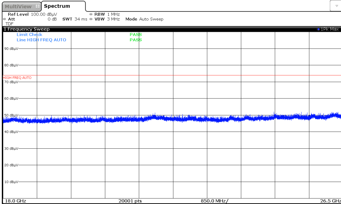
Plot 7-85. Radiated Spurious Plot between 18-26.5GHz (802.11a – Ant. Pol. H)
