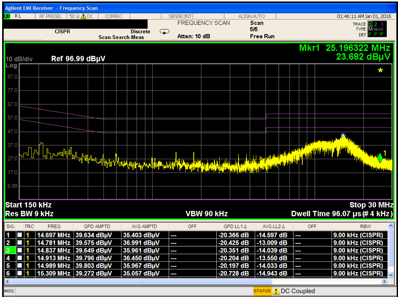
Plot 7-52. Line Conducted Plot with 802.11b (L1)
