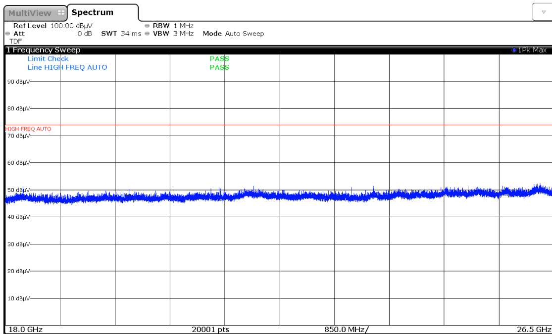
Plot 7-44. Radiated Spurious Plot above 18GHz (Pol. V)
