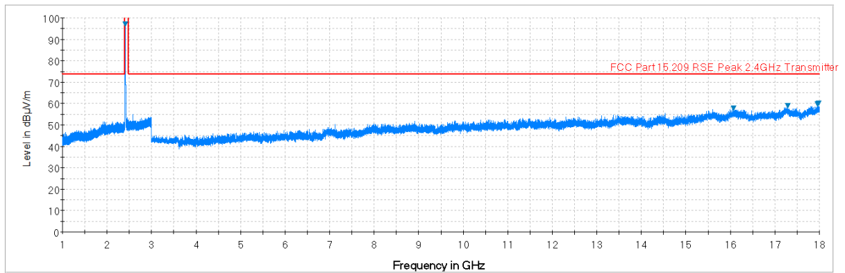
Plot 7-38. Radiated Spurious Plot above 1GHz (802.11b – Ch. 1, Ant. Pol. V)
