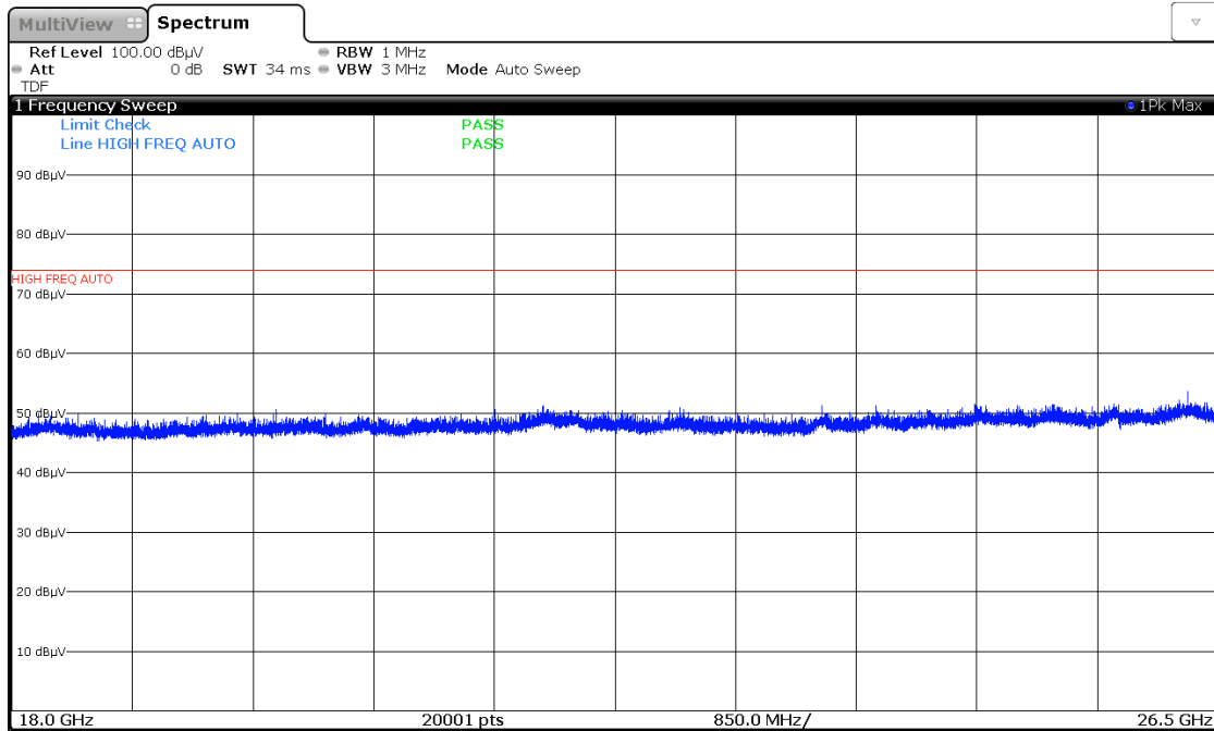
Plot 7-43. Radiated Spurious Plot above 18GHz (Pol. H)
