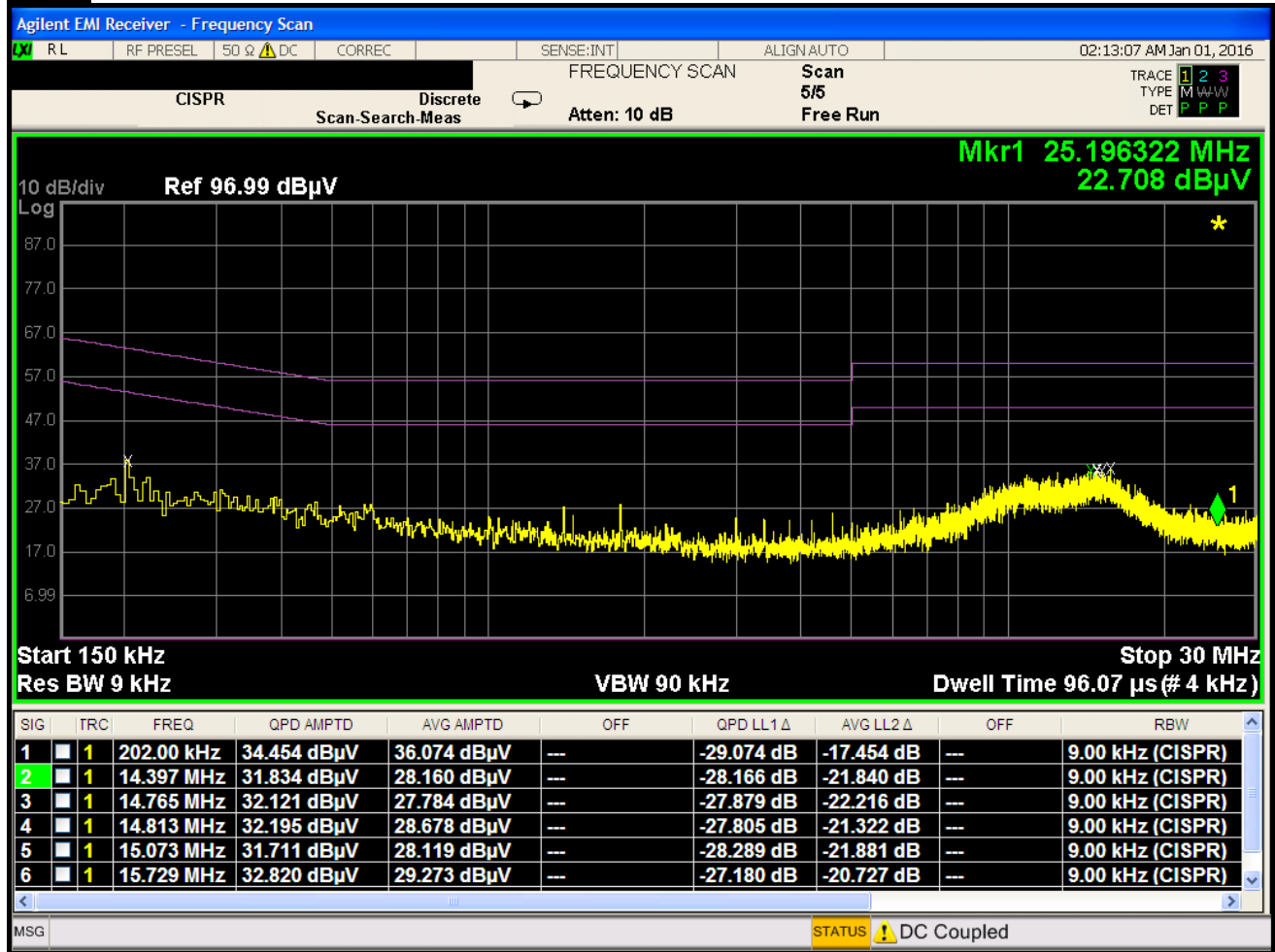
Plot 7-53. Line Conducted Plot with 802.11b (N)
