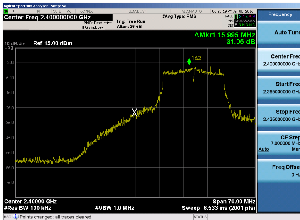
Plot 7-28. Band Edge Plot (802.11n (2.4GHz) – Ch. 2)
