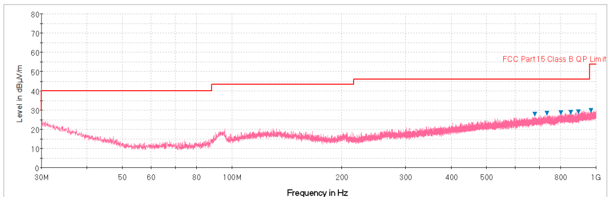
Plot 7-50. Radiated Spurious Plot below 1GHz (Pol. H)
