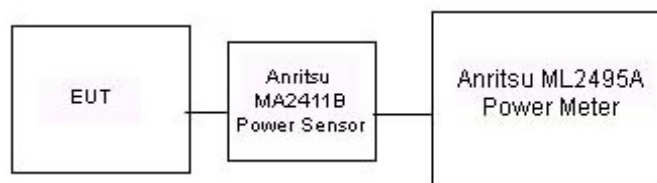
Figure 7-2. Test Instrument & Measurement Setup for Power Meter Measurements
