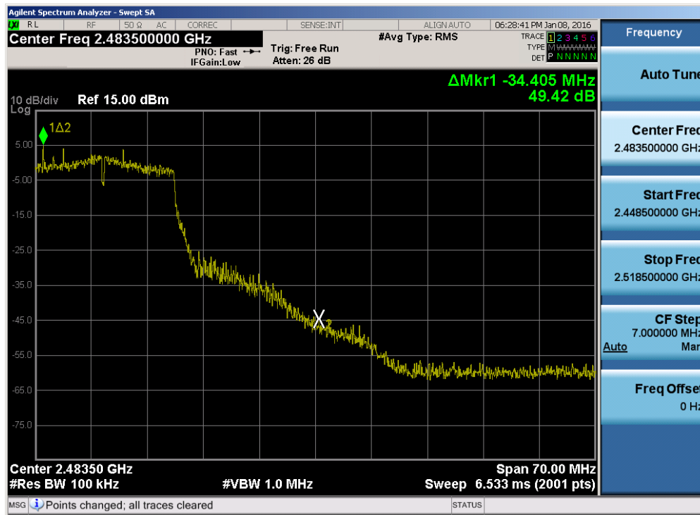
Plot 7-29. Band Edge Plot (802.11n (2.4GHz) – Ch. 10)
