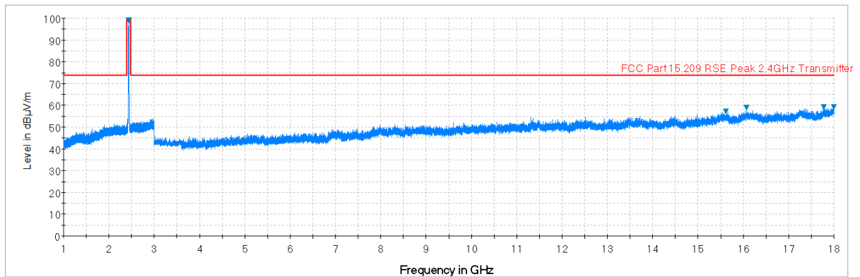
Plot 7-39. Radiated Spurious Plot above 1GHz (802.11b – Ch. 6, Ant. Pol. H)
