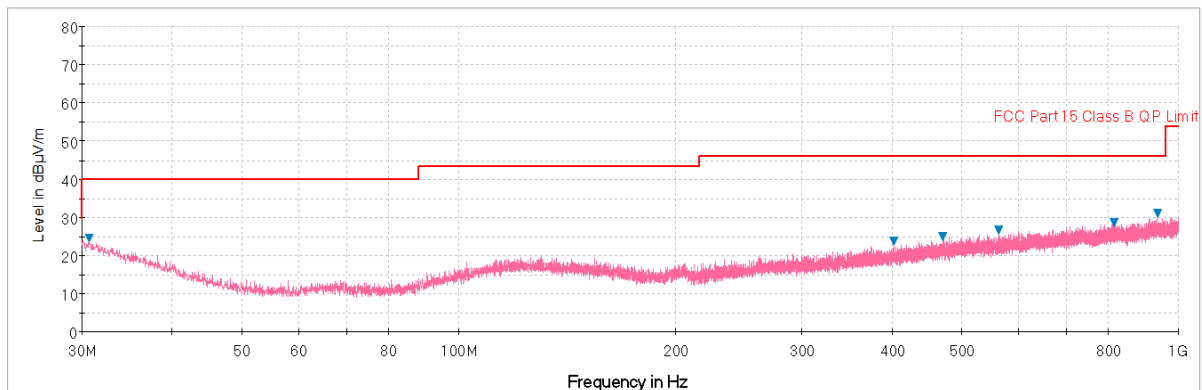
Plot 7-51. Radiated Spurious Plot below 1GHz (Pol. V)
