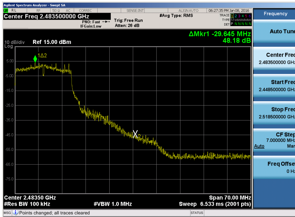
Plot 7-25. Band Edge Plot (802.11g– Ch. 10)
