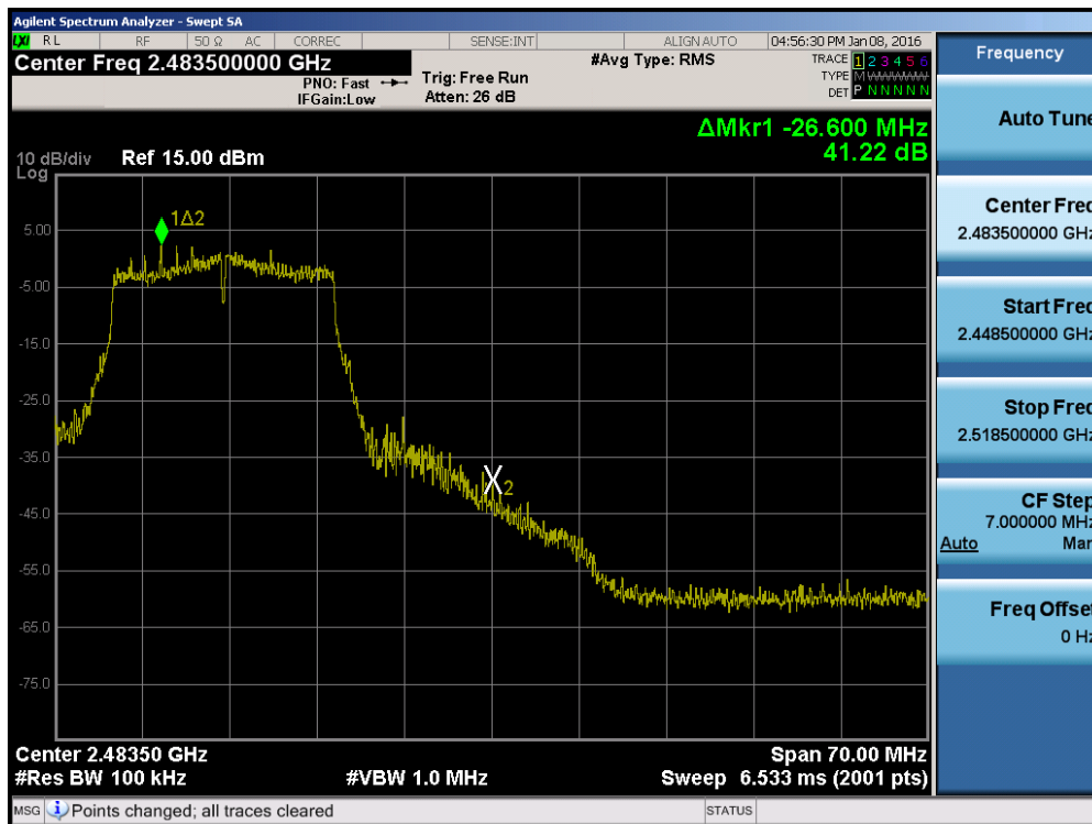
Plot 7-30. Band Edge Plot (802.11n (2.4GHz) – Ch. 11)
