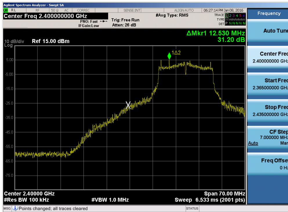
Plot 7-24. Band Edge Plot (802.11g– Ch. 2)
