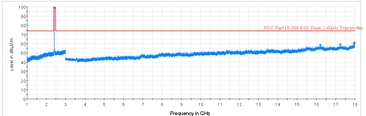
Plot 7-37. Radiated Spurious Plot above 1GHz (802.11b – Ch. 1, Ant. Pol. H)
