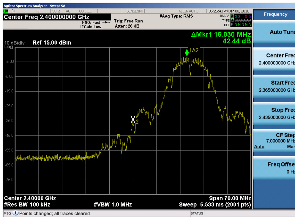
Plot 7-20. Band Edge Plot (802.11b – Ch. 2)
