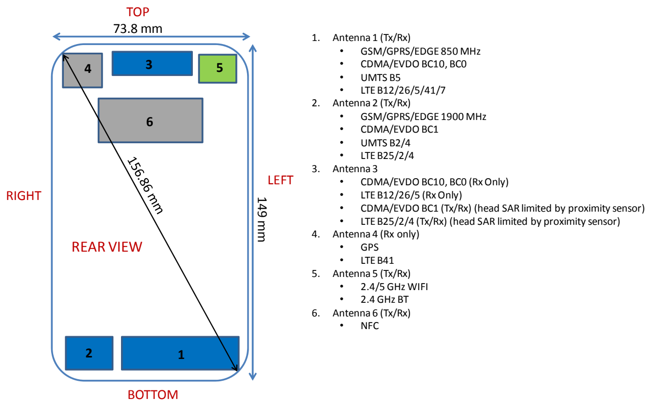
Figure F-1 DUT Antenna Locations
