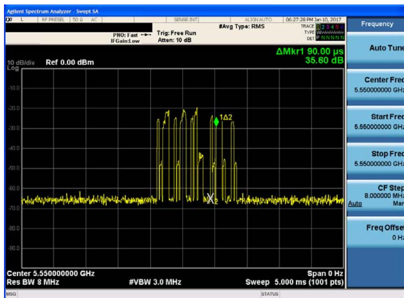
Figure 5-4. Band 2C Period
