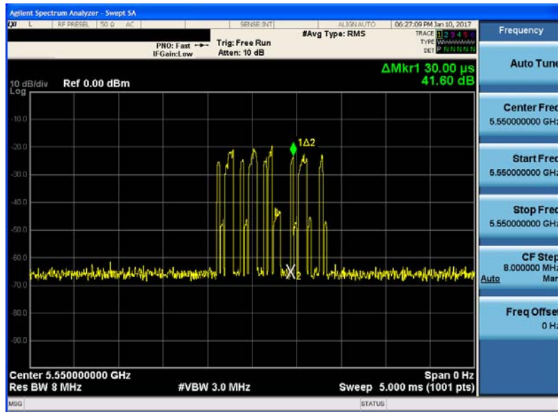
Figure 5-3. Band 2C Pulse Width
