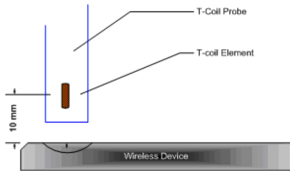
Figure 4-11 Measurement Distance
