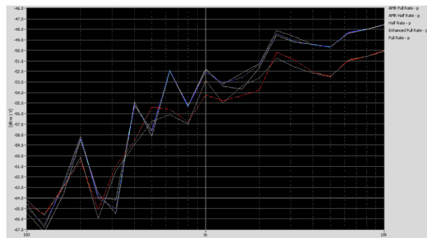
Figure 4-13 Vocoder Analysis for ABM Noise for GSM
