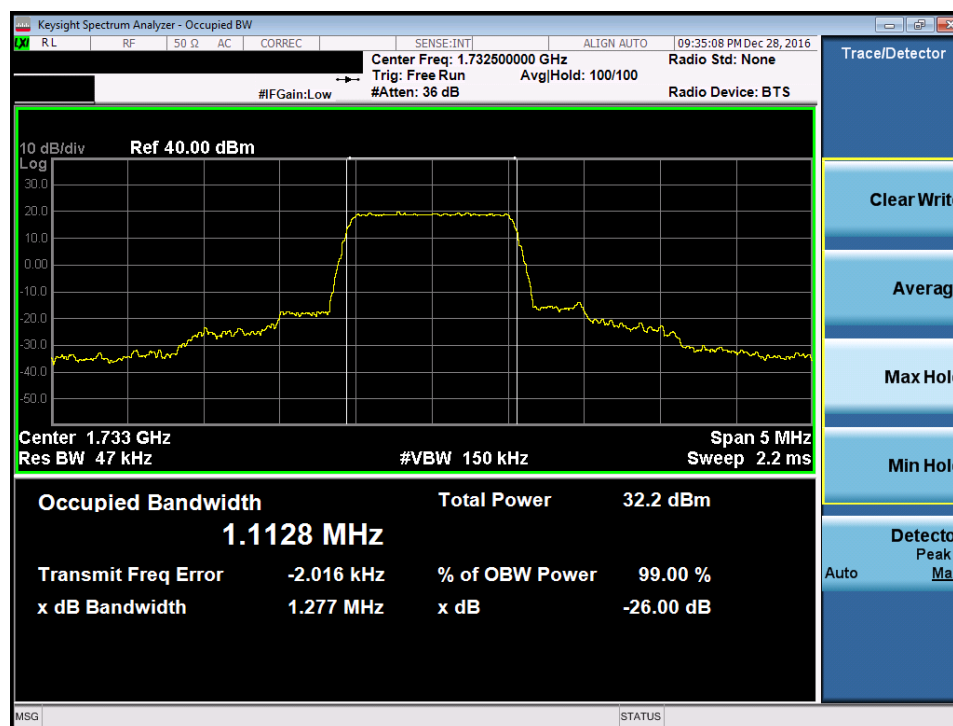
Plot 7-28. Occupied Bandwidth Plot (Band 4 – 1.4MHz QPSK – RB Size 6)
