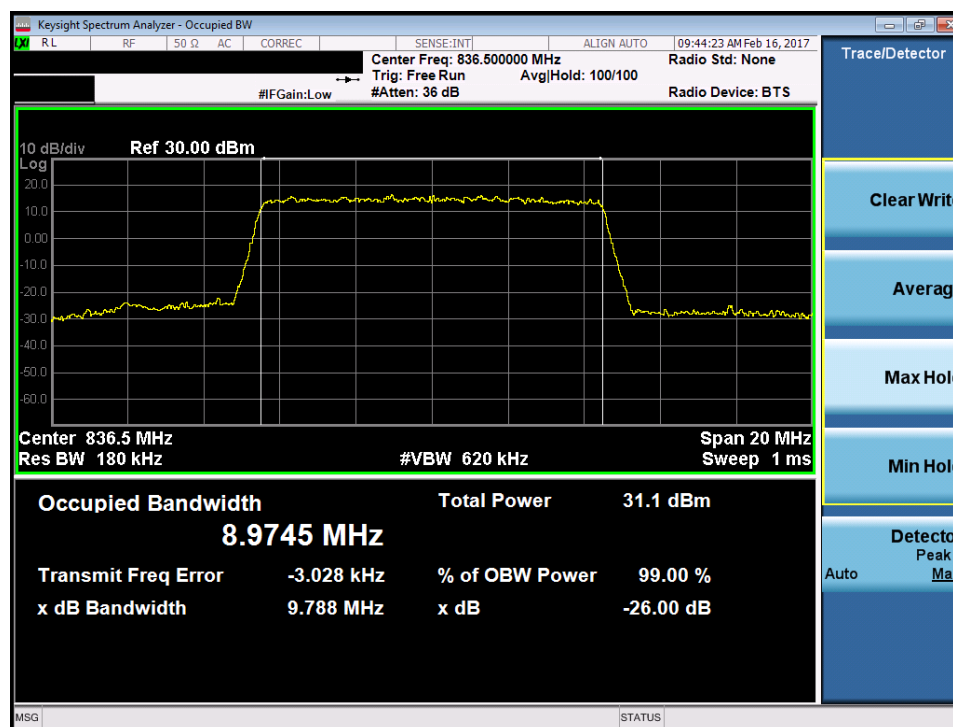
Plot 7-24. Occupied Bandwidth Plot (Band 26/5 – 10.0MHz 64-QAM – RB Size 50)
