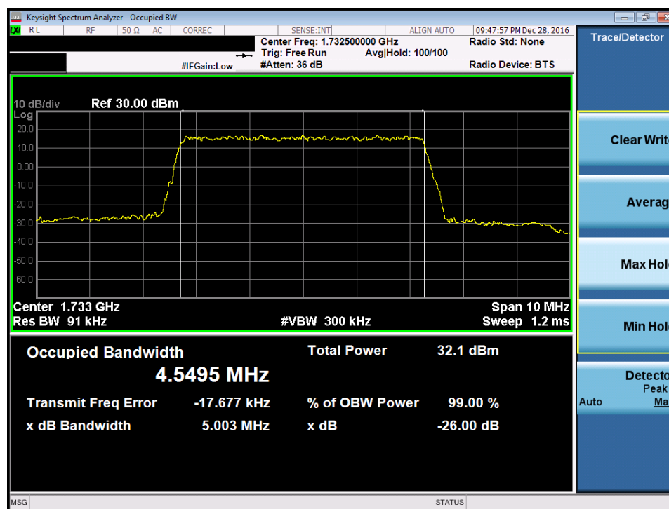
Plot 7-34. Occupied Bandwidth Plot (Band 4 – 5.0MHz QPSK – RB Size 25)
