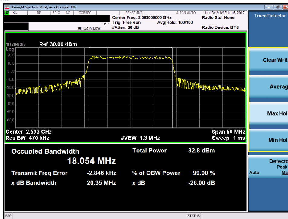
Plot 7-75. Occupied Bandwidth Plot (Band 41 – 20.0MHz 64-QAM – RB Size 100)
