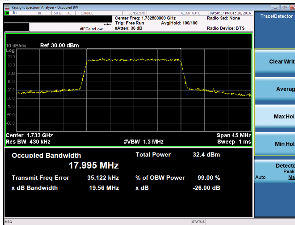
Plot 7-43. Occupied Bandwidth Plot (Band 4 – 20.0MHz QPSK – RB Size 100)
