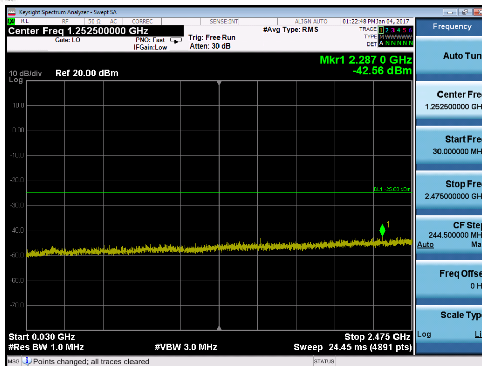
Plot 7-112. Conducted Spurious Plot (Band 41 – 5.0MHz QPSK – RB Size 1, RB Offset 0 – Low Channel)
