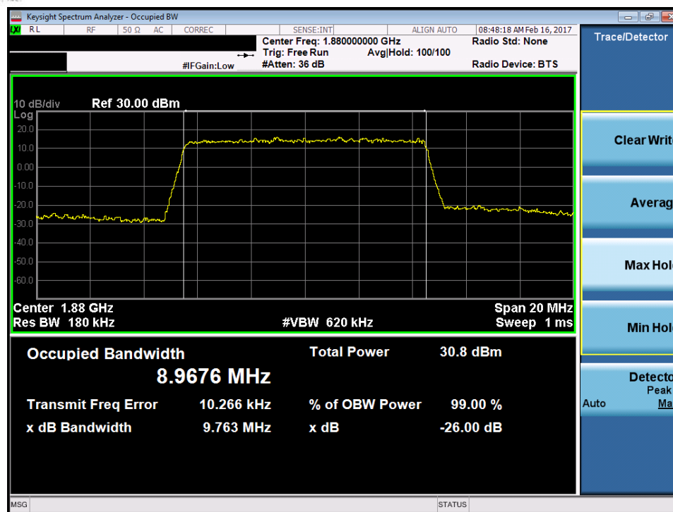
Plot 7-57. Occupied Bandwidth Plot (Band 25/2 – 10.0MHz 64-QAM – RB Size 50)
