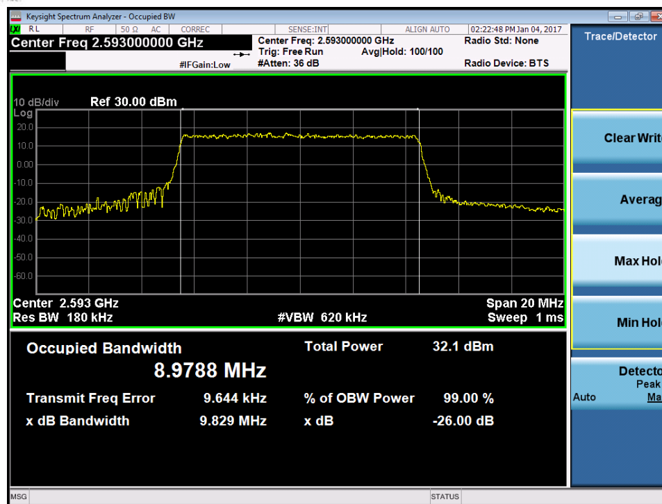
Plot 7-67. Occupied Bandwidth Plot (Band 41 – 10.0MHz QPSK – RB Size 50)
