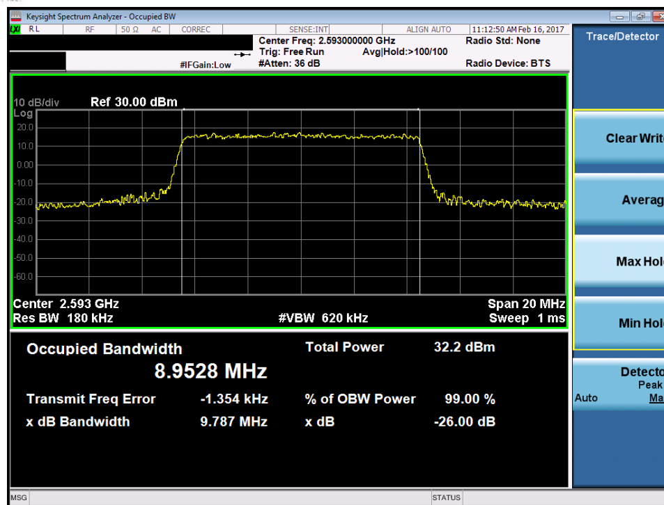
Plot 7-69. Occupied Bandwidth Plot (Band 41 – 10.0MHz 64-QAM – RB Size 50)
