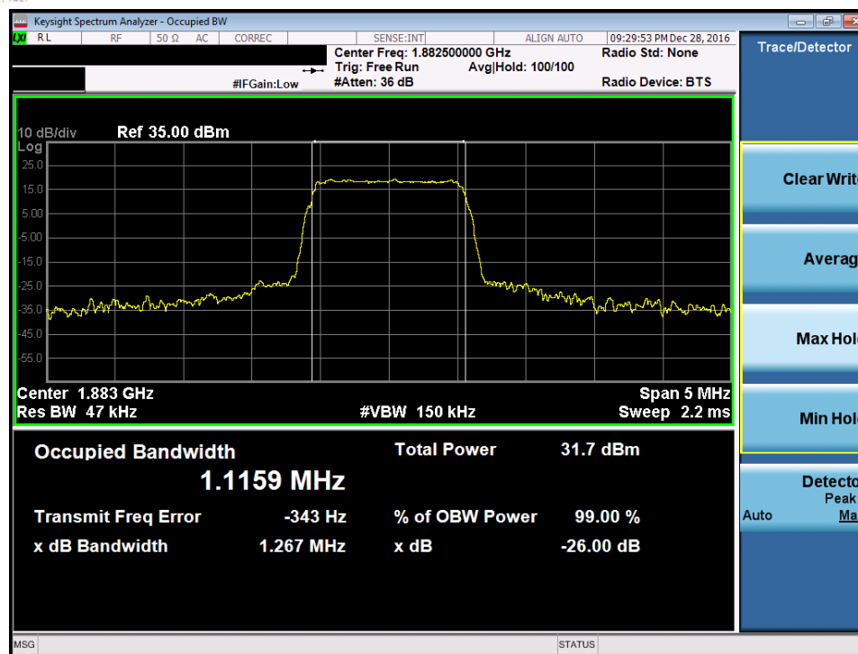
Plot 7-47. Occupied Bandwidth Plot (Band 25/2 – 1.4MHz 16-QAM – RB Size 6)
