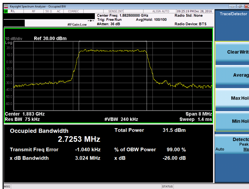
Plot 7-50. Occupied Bandwidth Plot (Band 25/2 – 3.0MHz 16-QAM – RB Size 15)
