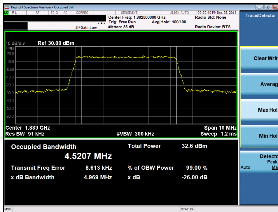
Plot 7-52. Occupied Bandwidth Plot (Band 25/2 – 5.0MHz QPSK – RB Size 25)
