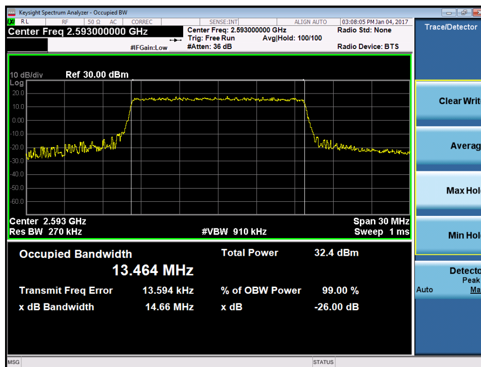
Plot 7-70. Occupied Bandwidth Plot (Band 41 – 15.0MHz QPSK – RB Size 75)
