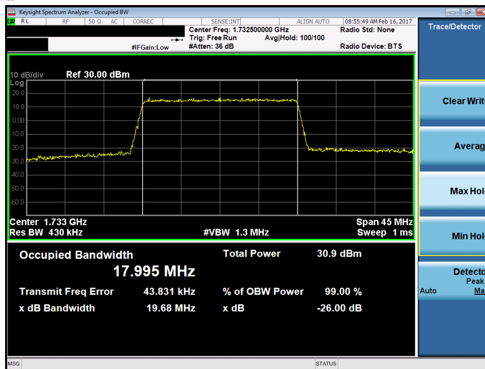
Plot 7-45. Occupied Bandwidth Plot (Band 4 – 20.0MHz 64-QAM – RB Size 100)
