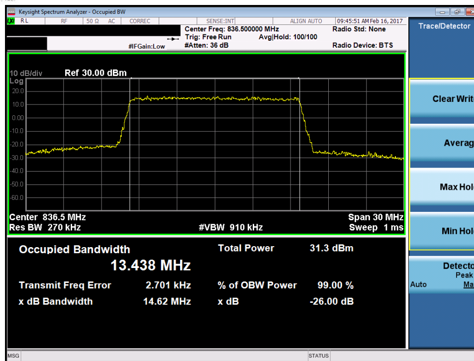
Plot 7-27. Occupied Bandwidth Plot (Band 26 – 15.0MHz 64-QAM – RB Size 50)
