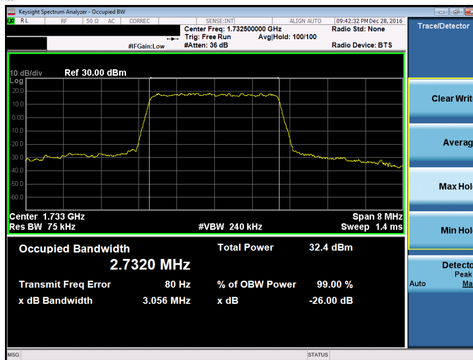
Plot 7-31. Occupied Bandwidth Plot (Band 4 – 3.0MHz QPSK – RB Size 15)
