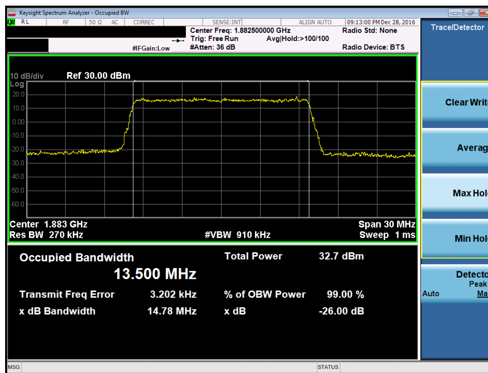
Plot 7-58. Occupied Bandwidth Plot (Band 25/2 – 15.0MHz QPSK – RB Size 75)
