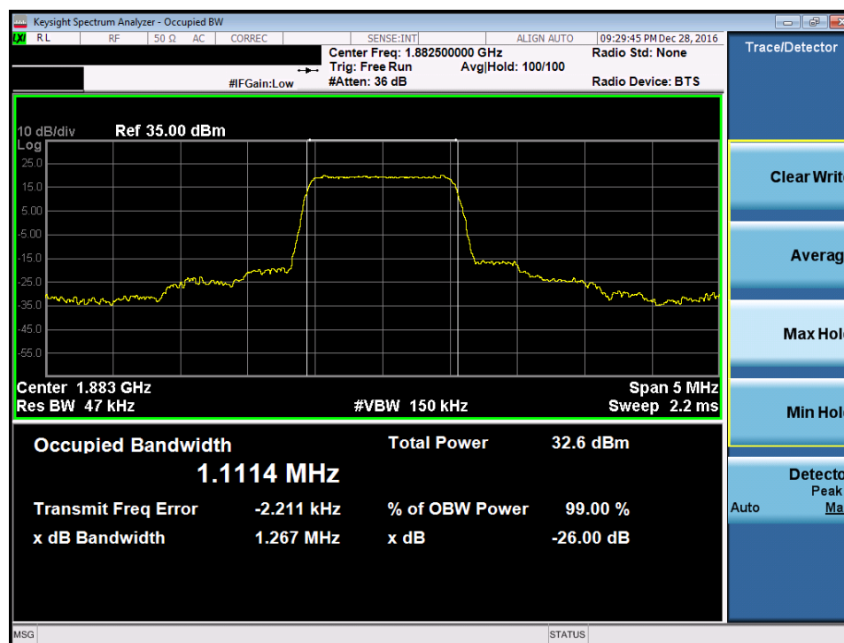
Plot 7-46. Occupied Bandwidth Plot (Band 25/2 – 1.4MHz QPSK – RB Size 6)
