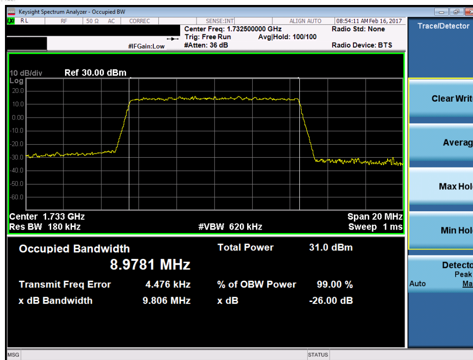
Plot 7-39. Occupied Bandwidth Plot (Band 4 – 10.0MHz 64-QAM – RB Size 50)
