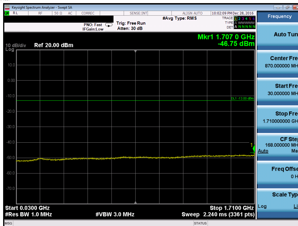
Plot 7-100. Conducted Spurious Plot (Band 4 – 20.0MHz QPSK – RB Size 1, RB Offset 0 – High Channel)
