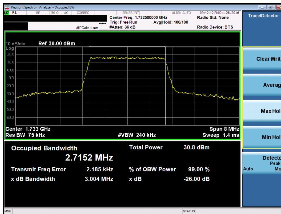
Plot 7-32. Occupied Bandwidth Plot (Band 4 – 3.0MHz 16-QAM – RB Size 15)
