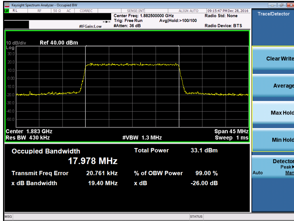
Plot 7-61. Occupied Bandwidth Plot (Band 25/2 – 20.0MHz QPSK – RB Size 100)
