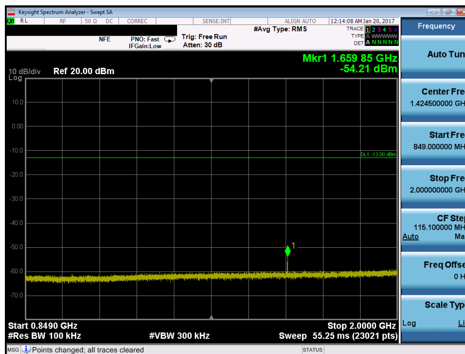
Plot 7-89. Conducted Spurious Plot (Band 26 – 15.0MHz QPSK – RB Size 1, RB Offset 0 – Mid Channel)
