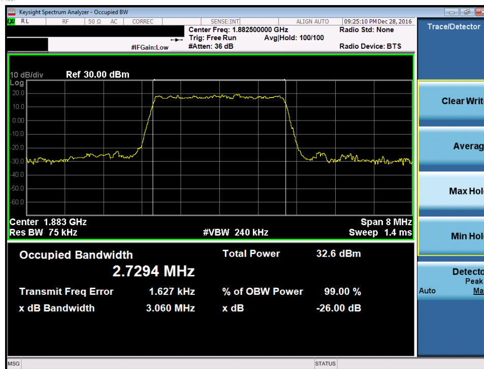
Plot 7-49. Occupied Bandwidth Plot (Band 25/2 – 3.0MHz QPSK – RB Size 15)
