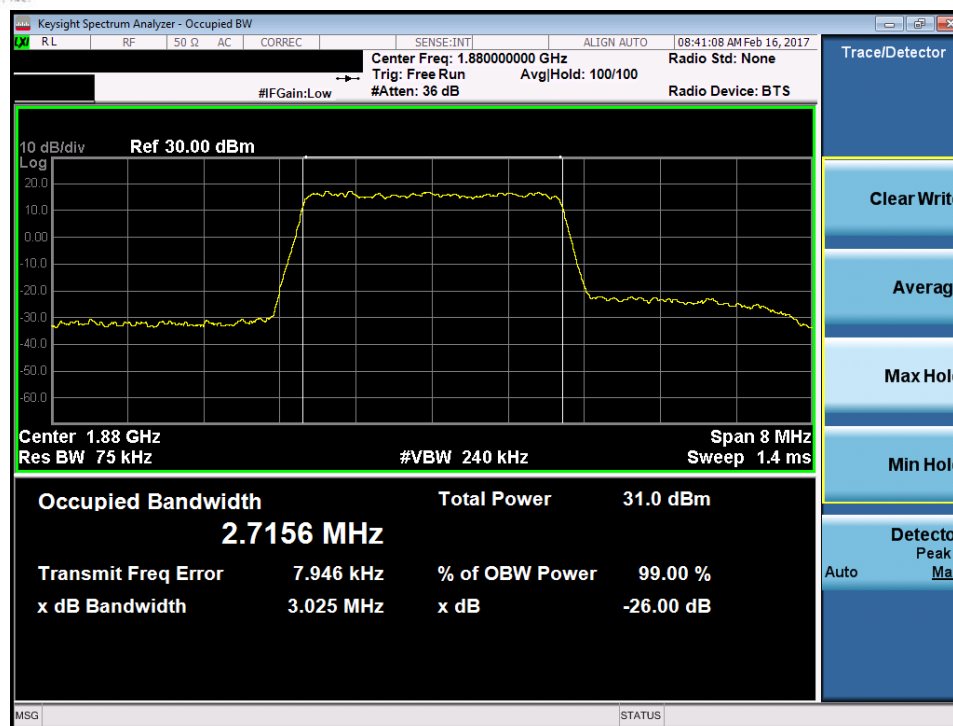
Plot 7-51. Occupied Bandwidth Plot (Band 25/2 – 3.0MHz 64-QAM – RB Size 15)
