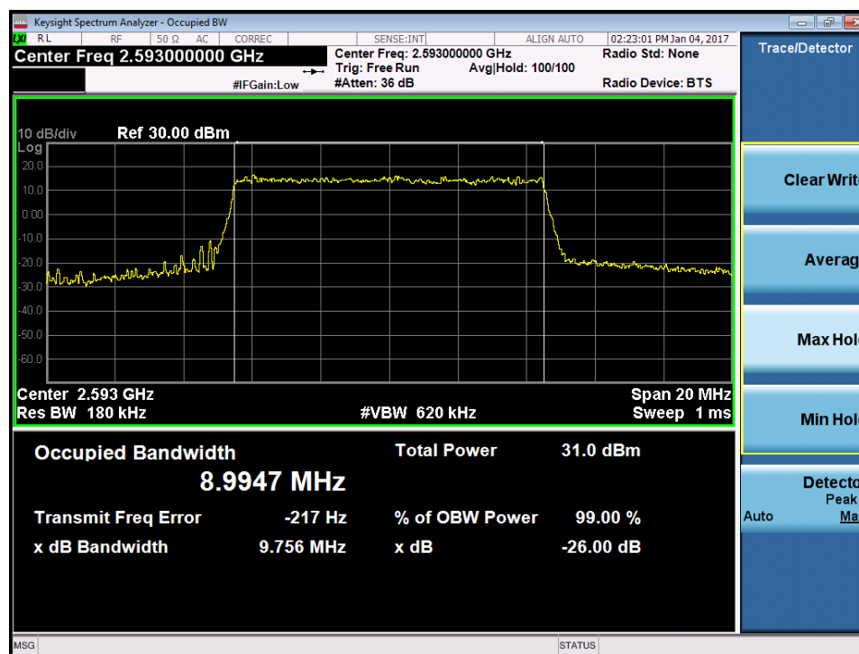
Plot 7-68. Occupied Bandwidth Plot (Band 41 – 10.0MHz 16-QAM – RB Size 50)
