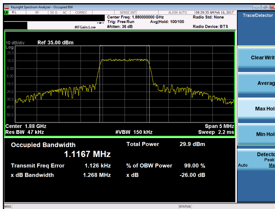
Plot 7-48. Occupied Bandwidth Plot (Band 25/2 – 1.4MHz 64-QAM – RB Size 6)
