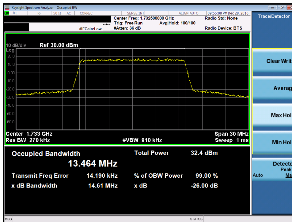
Plot 7-40. Occupied Bandwidth Plot (Band 4 – 15.0MHz QPSK – RB Size 75)
