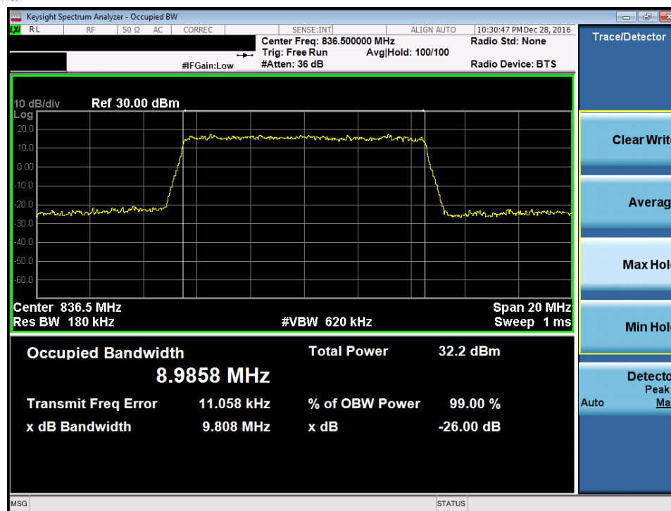
Plot 7-23. Occupied Bandwidth Plot (Band 26/5 – 10.0MHz 16-QAM – RB Size 50)
