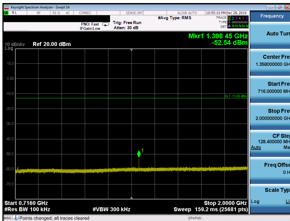
Plot 7-77. Conducted Spurious Plot (Band 12 – 3.0MHz QPSK – RB Size 1, RB Offset 0 – Low Channel)
