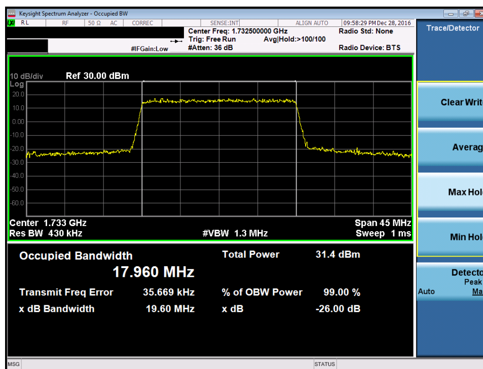
Plot 7-44. Occupied Bandwidth Plot (Band 4 – 20.0MHz 16-QAM – RB Size 100)
