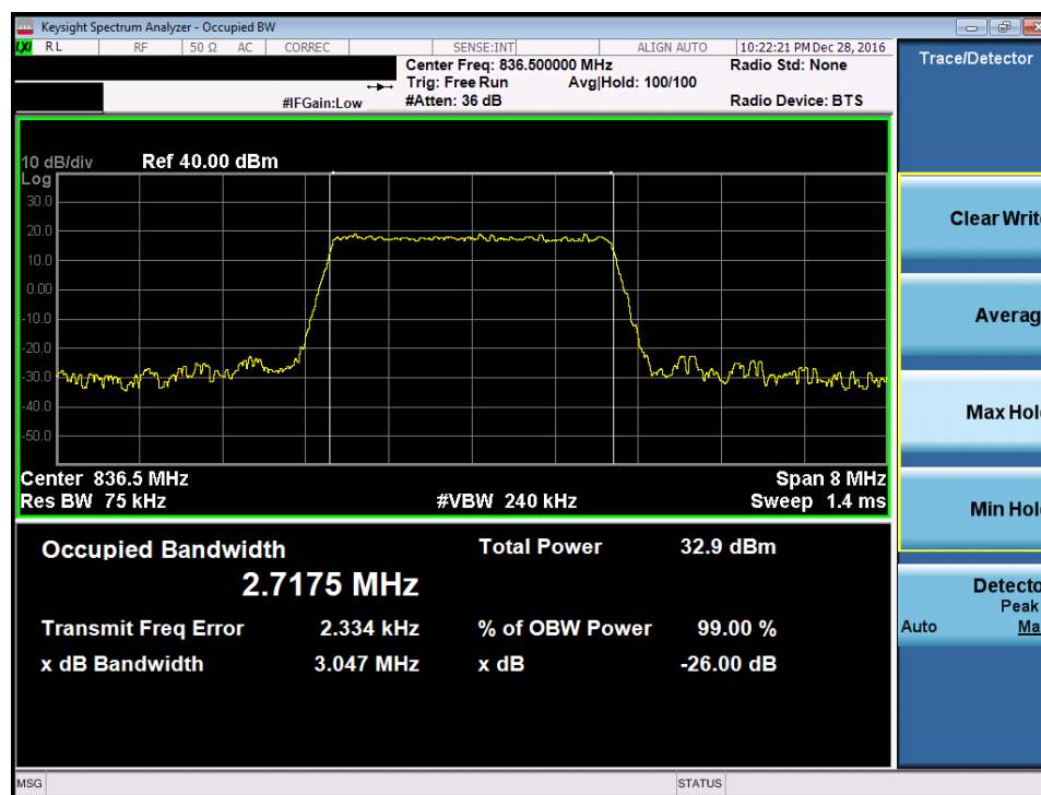
Plot 7-16. Occupied Bandwidth Plot (Band 26/5 – 3.0MHz QPSK – RB Size 15)
