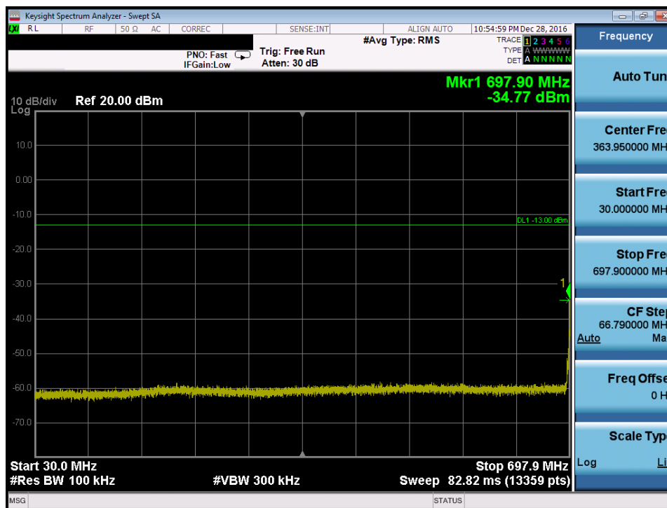
Plot 7-76. Conducted Spurious Plot (Band 12 – 3.0MHz QPSK – RB Size 1, RB Offset 0 – Low Channel)
