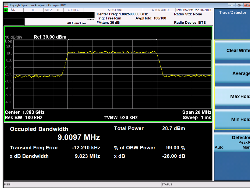
Plot 7-56. Occupied Bandwidth Plot (Band 25/2 – 10.0MHz 16-QAM – RB Size 50)
