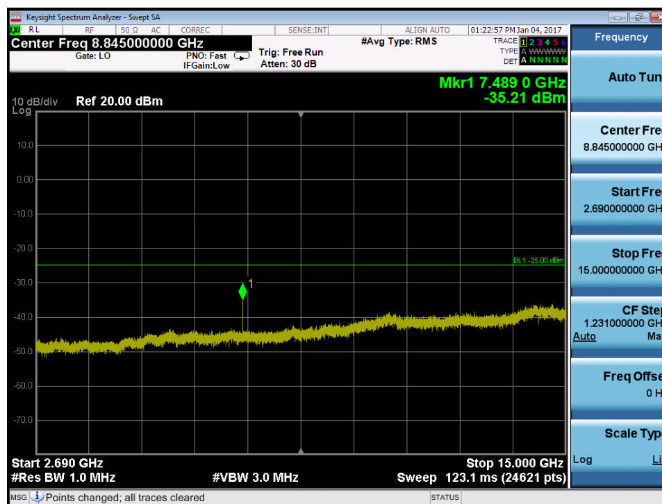
Plot 7-113. Conducted Spurious Plot (Band 41 – 5.0MHz QPSK – RB Size 1, RB Offset 0 – Low Channel)
