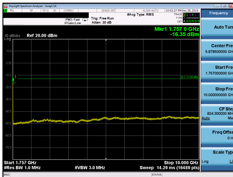
Plot 7-101. Conducted Spurious Plot (Band 4 – 20.0MHz QPSK – RB Size 1, RB Offset 0 – High Channel)
