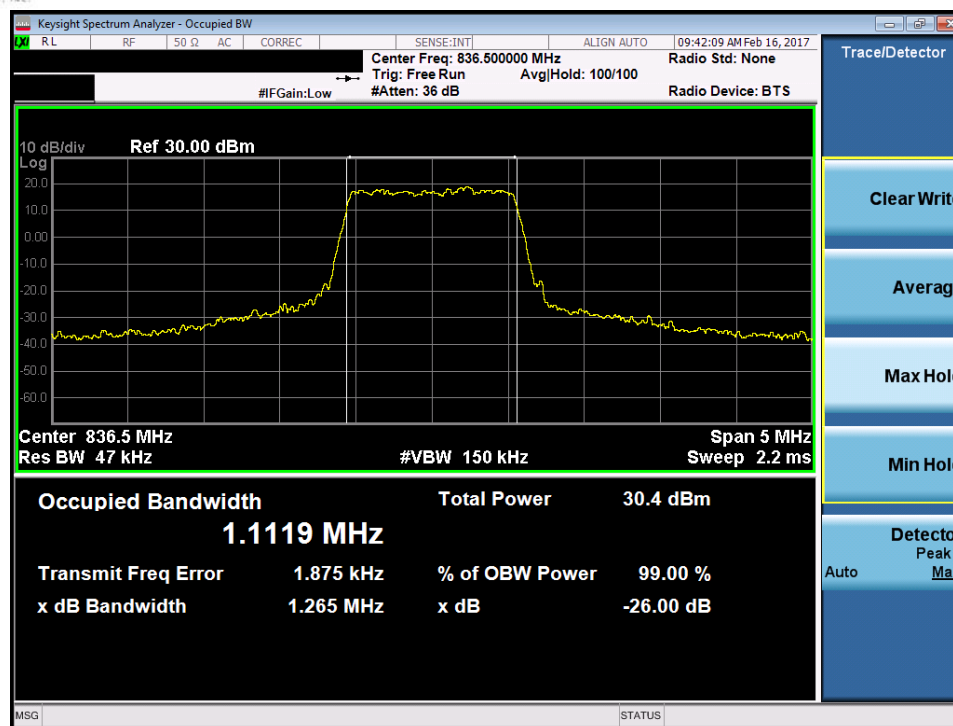
Plot 7-15. Occupied Bandwidth Plot (Band 26/5 – 1.4MHz 64-QAM – RB Size 6)
