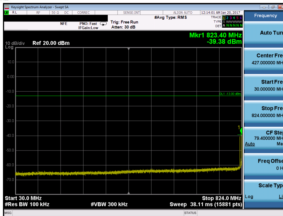
Plot 7-88. Conducted Spurious Plot (Band 26 – 15.0MHz QPSK – RB Size 1, RB Offset 0 – Mid Channel)
