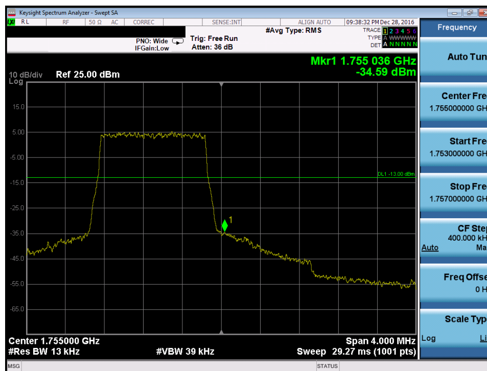
Plot 7-141. Upper Band Edge Plot (Band 4 – 1.4MHz QPSK – RB Size 6)
