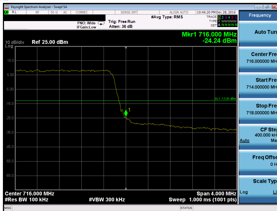
Plot 7-126. Upper Band Edge Plot (Band 12 – 5.0MHz QPSK – RB Size 25)
