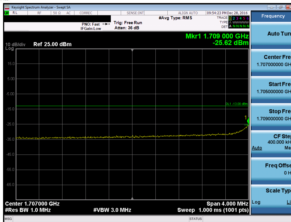
Plot 7-152. Lower Extended Band Edge Plot (Band 4 – 10.0MHz QPSK – RB Size 50)
