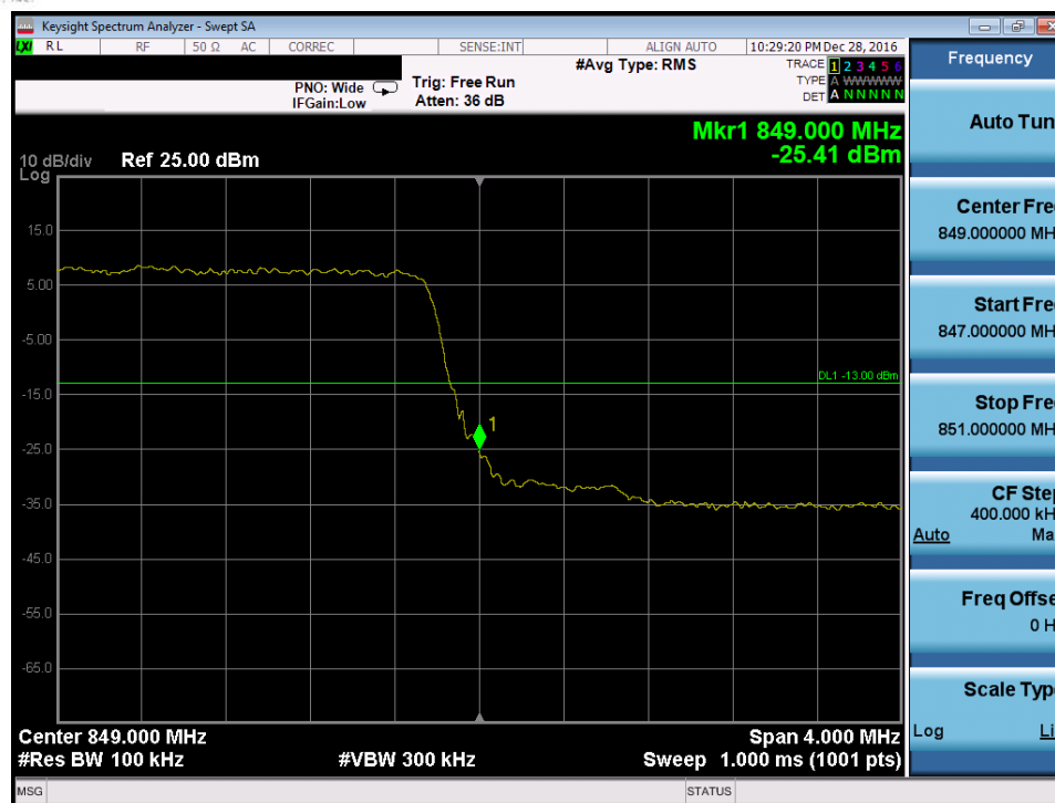
Plot 7-134. Upper Band Edge Plot (Band 26/5 – 5.0MHz QPSK – RB Size 25)
