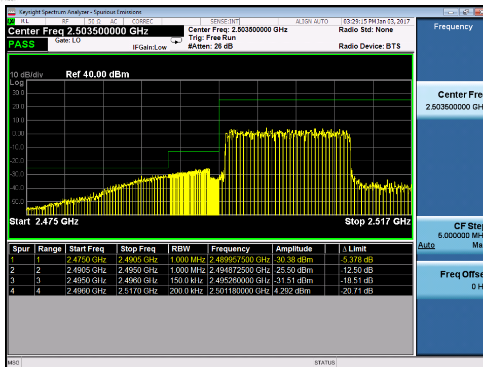
Plot 7-206. Lower ACP Plot with AMPR Reduction (Band 41 – 15.0MHz QPSK – RB Size 75)
