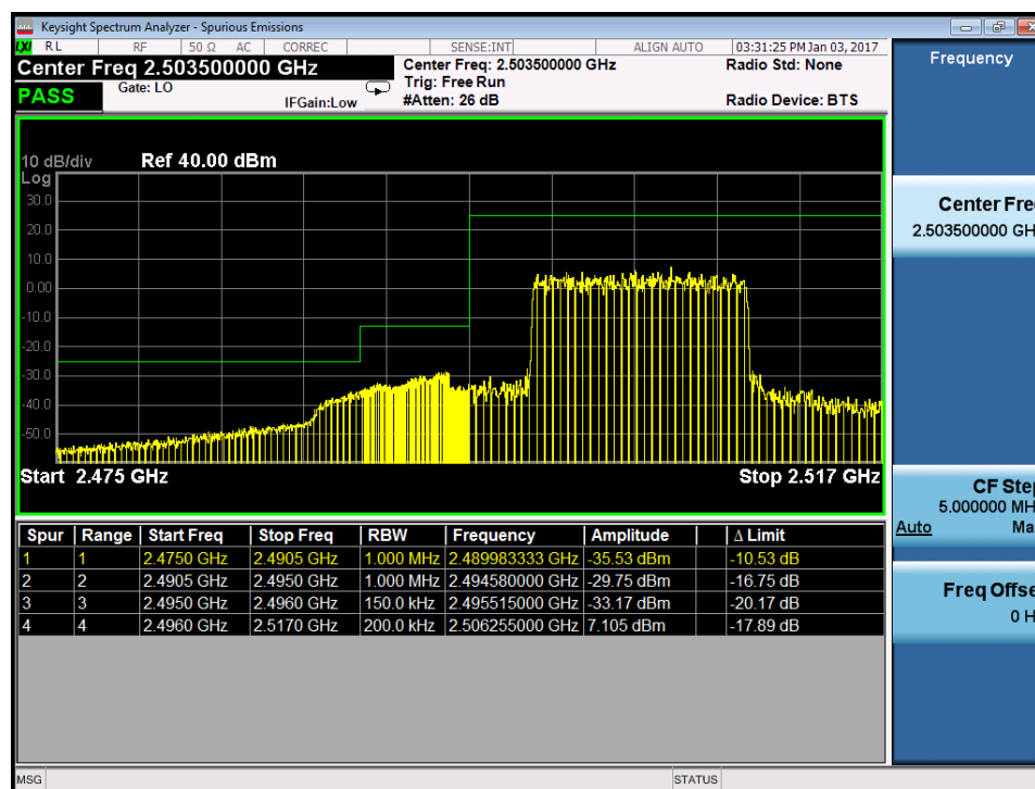
Plot 7-205. Lower ACP Plot with AMPR Reduction (Band 41 – 15.0MHz QPSK – RB Size 60)
