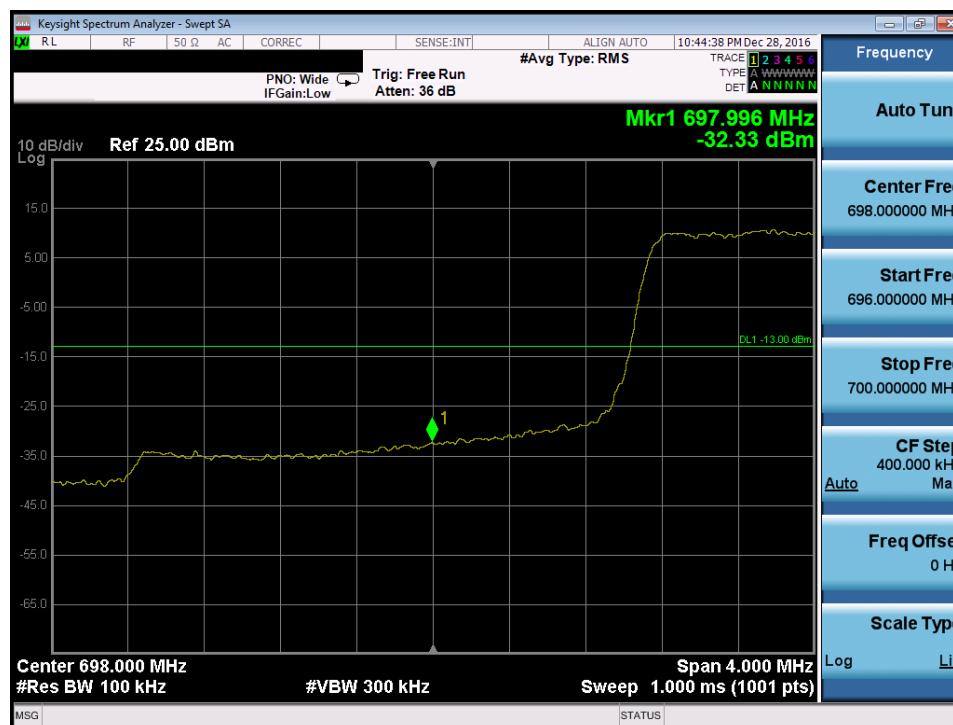
Plot 7-123. Lower Band Edge Plot (Band 12 – 3.0MHz QPSK – RB Size 15)
