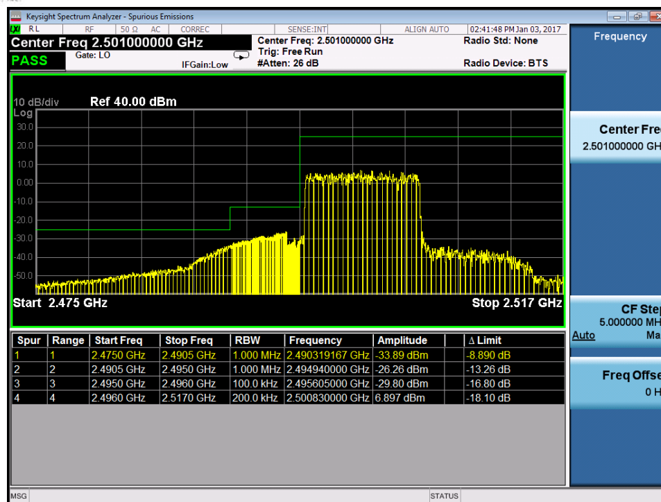
Plot 7-198. Lower ACP Plot with AMPR Reduction (Band 41 – 10.0MHz QPSK – RB Size 50)
