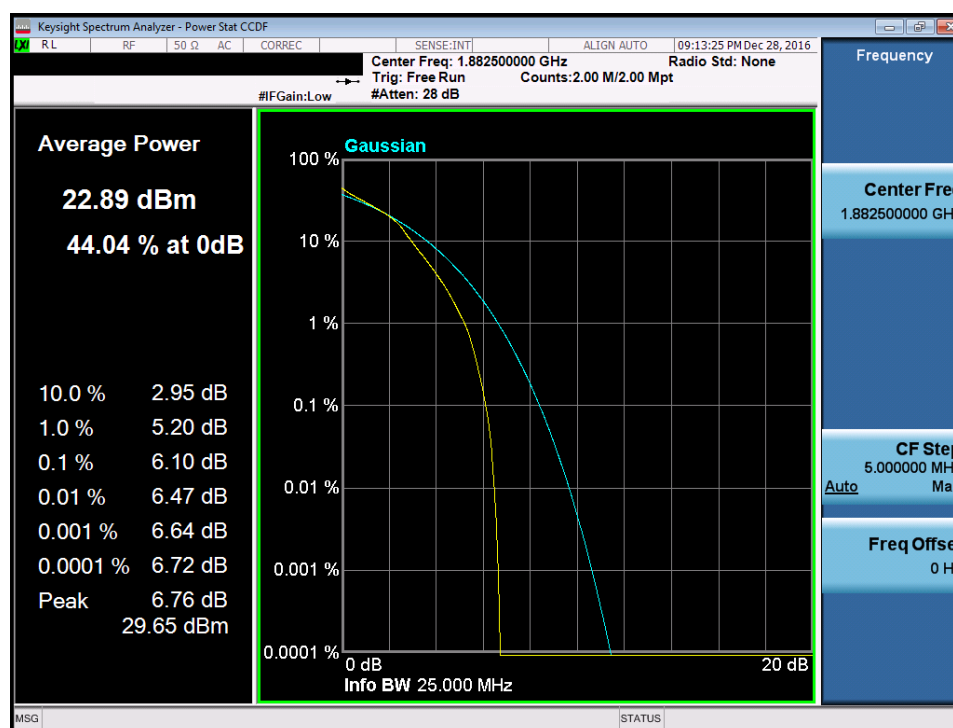
Plot 7-230. PAR Plot (Band 25/2 – 15.0MHz 16-QAM – RB Size 75)
