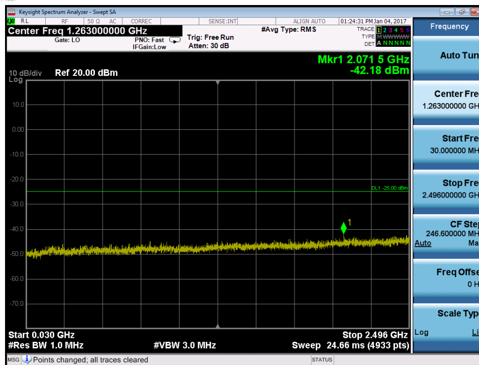
Plot 7-118. Conducted Spurious Plot (Band 41 – 5.0MHz QPSK – RB Size 1, RB Offset 0 – High Channel)
