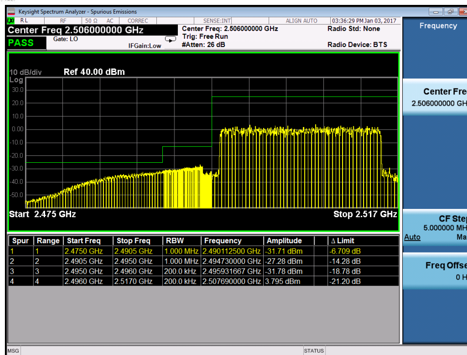
Plot 7-214. Lower ACP Plot with AMPR Reduction (Band 41 – 20.0MHz QPSK – RB Size 100)
