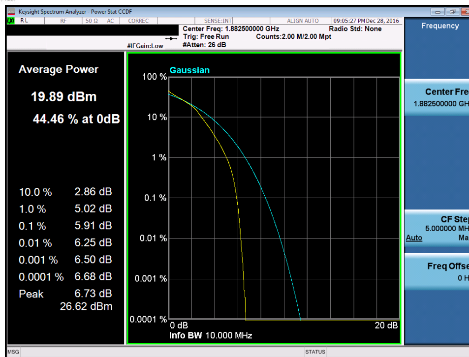
Plot 7-227. PAR Plot (Band 25/2 – 10.0MHz 16-QAM – RB Size 50)
