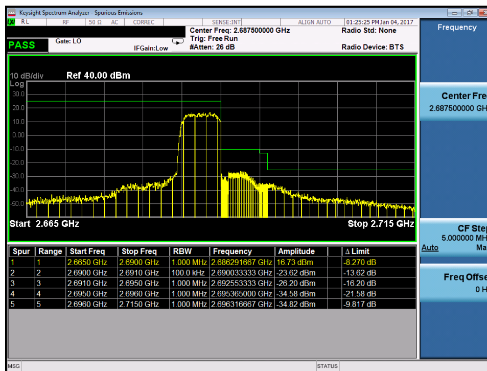
Plot 7-191. Upper ACP Plot (Band 41 – 5.0MHz QPSK – RB Size 25)
