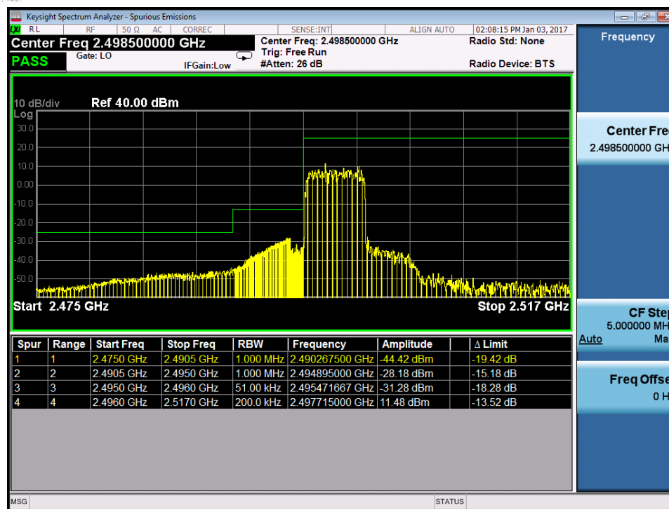
Plot 7-190. Lower ACP Plot with AMPR Reduction (Band 41 – 5.0MHz QPSK – RB Size 25)
