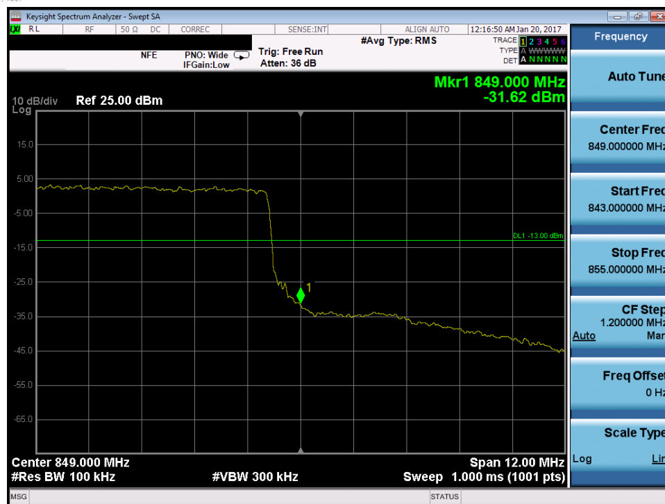
Plot 7-138. Upper Band Edge Plot (Band 26/5 – 15.0MHz QPSK – RB Size 75)
