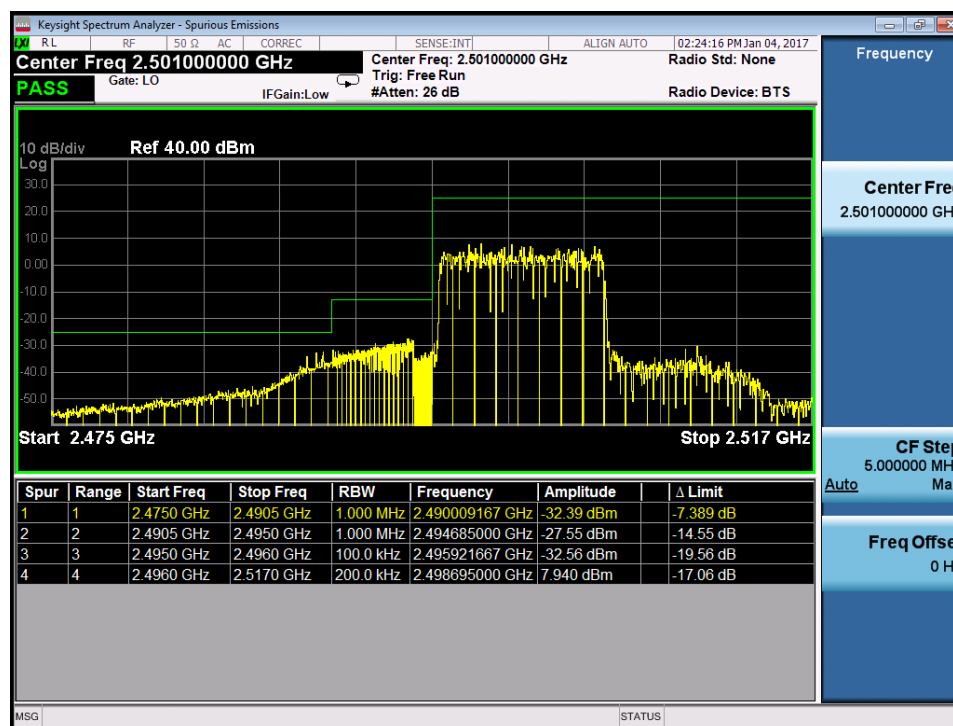
Plot 7-193. Lower ACP Plot (Band 41 – 10.0MHz QPSK – RB Size 50)
