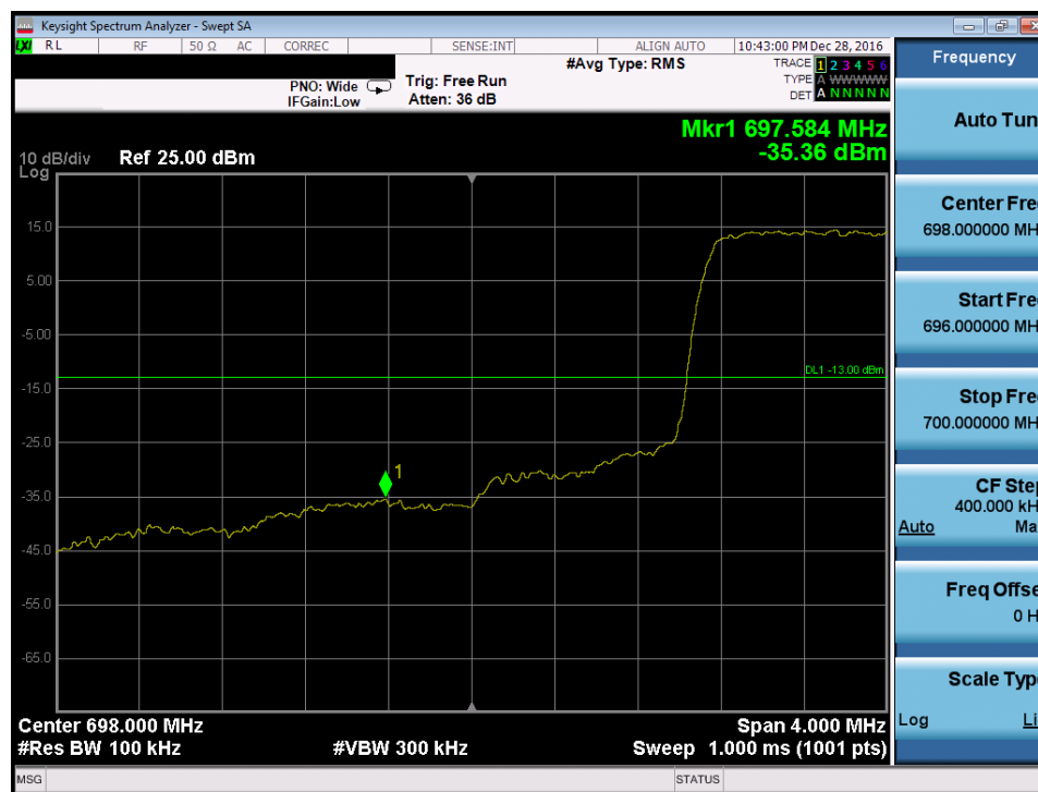
Plot 7-121. Lower Band Edge Plot (Band 12 – 1.4MHz QPSK – RB Size 6)
