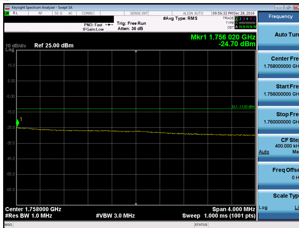
Plot 7-158. Upper Extended Band Edge Plot (Band 4 – 15.0MHz QPSK – RB Size 75)
