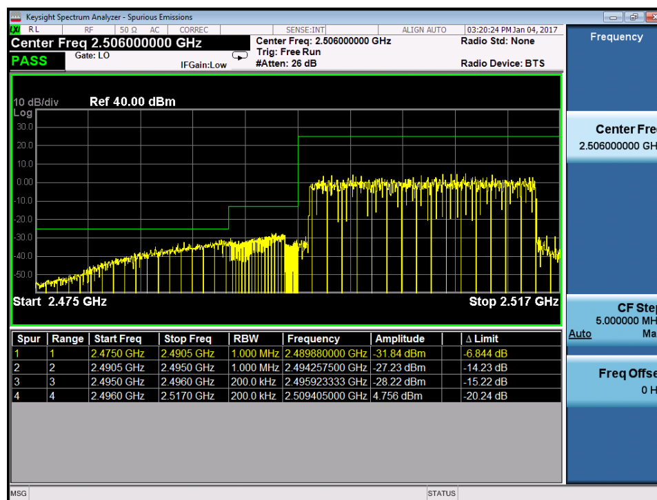
Plot 7-209. Lower ACP Plot (Band 41 – 20.0MHz QPSK – RB Size 100)
