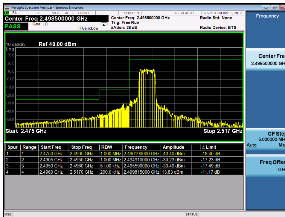
Plot 7-189. Lower ACP Plot with AMPR Reduction (Band 41 – 5.0MHz QPSK – RB Size 16)
