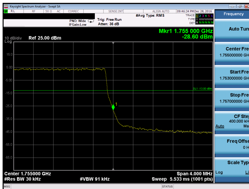
Plot 7-145. Upper Band Edge Plot (Band 4 – 3.0MHz QPSK – RB Size 15)
