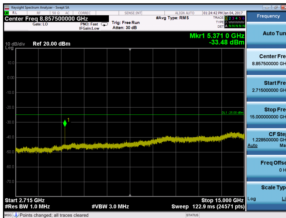
Plot 7-119. Conducted Spurious Plot (Band 41 – 5.0MHz QPSK – RB Size 1, RB Offset 0 – High Channel)
