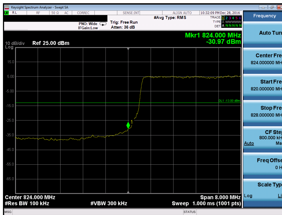
Plot 7-135. Lower Band Edge Plot (Band 26/5 – 10.0MHz QPSK – RB Size 50)
