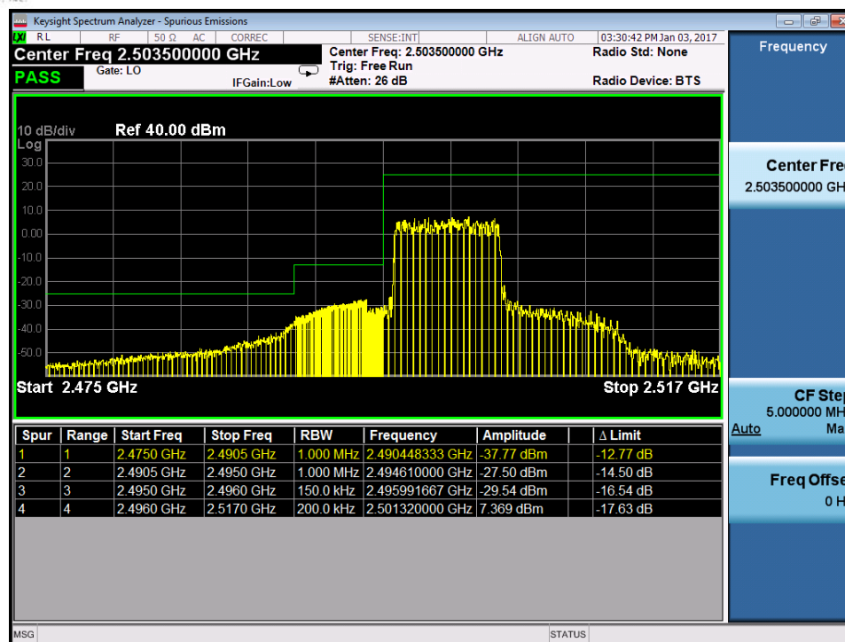
Plot 7-204. Lower ACP Plot with AMPR Reduction (Band 41 – 15.0MHz QPSK – RB Size 36)
