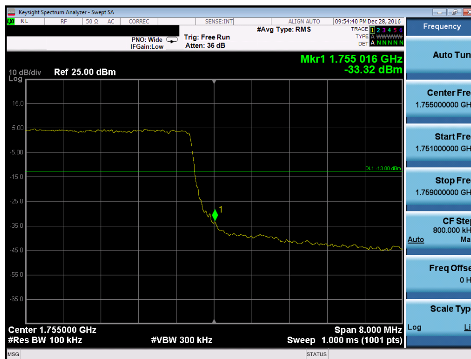
Plot 7-153. Upper Band Edge Plot (Band 4 – 10.0MHz QPSK – RB Size 50)
