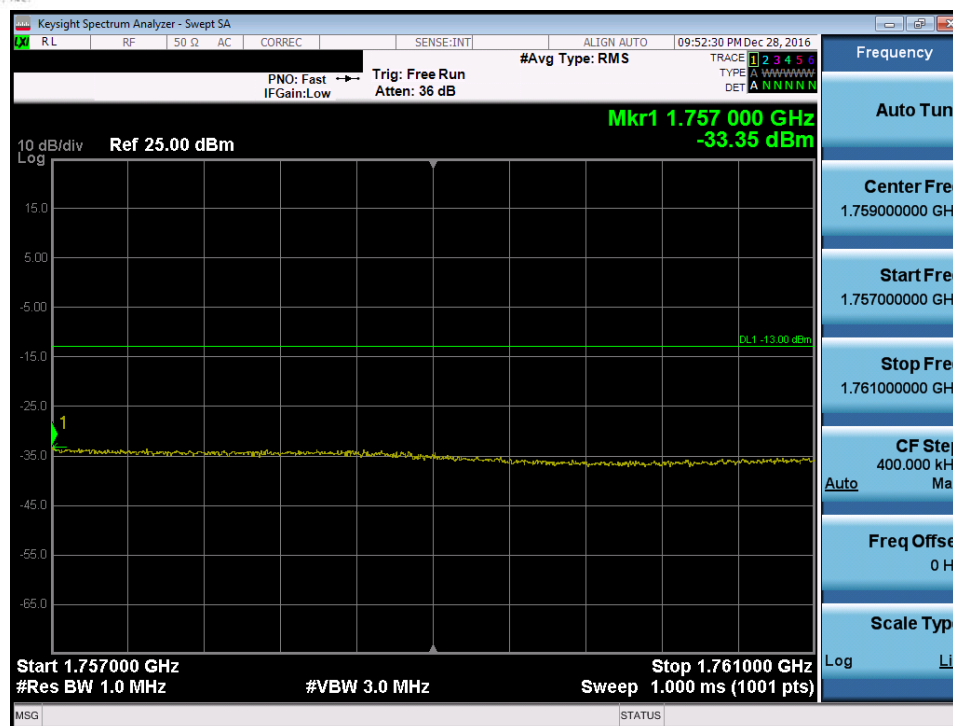
Plot 7-150. Upper Extended Band Edge Plot (Band 4 – 5.0MHz QPSK – RB Size 25)
