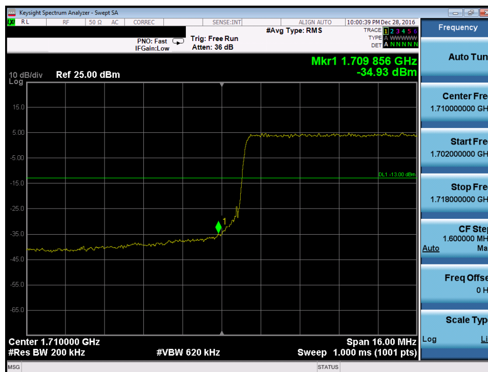
Plot 7-159. Lower Band Edge Plot (Band 4 – 20.0MHz QPSK – RB Size 100)
