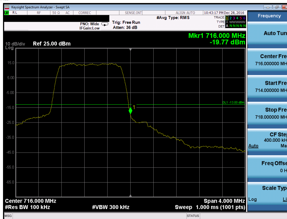
Plot 7-122. Upper Band Edge Plot (Band 12 – 1.4MHz QPSK – RB Size 6)
