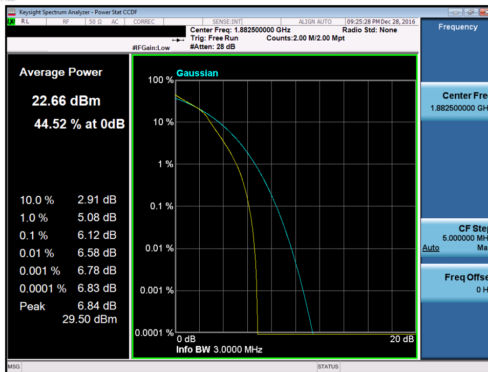
Plot 7-221. PAR Plot (Band 25/2 – 3.0MHz 16-QAM – RB Size 15)
