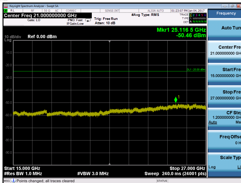
Plot 7-114. Conducted Spurious Plot (Band 41 – 5.0MHz QPSK – RB Size 1, RB Offset 0 – Low Channel)
