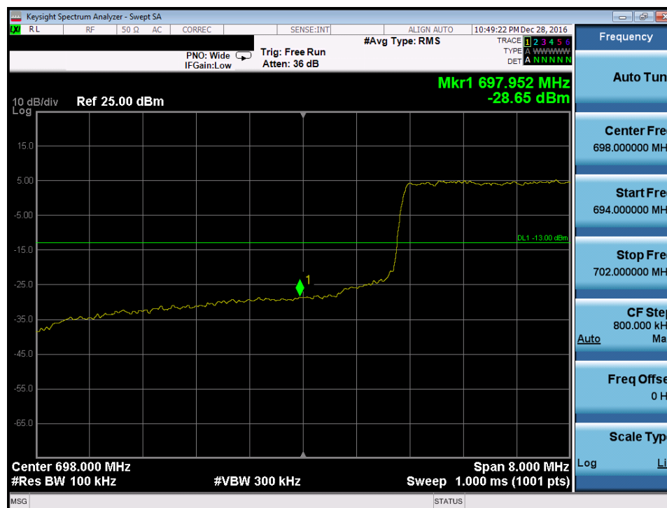
Plot 7-127. Lower Band Edge Plot (Band 12 – 10.0MHz QPSK – RB Size 50)
