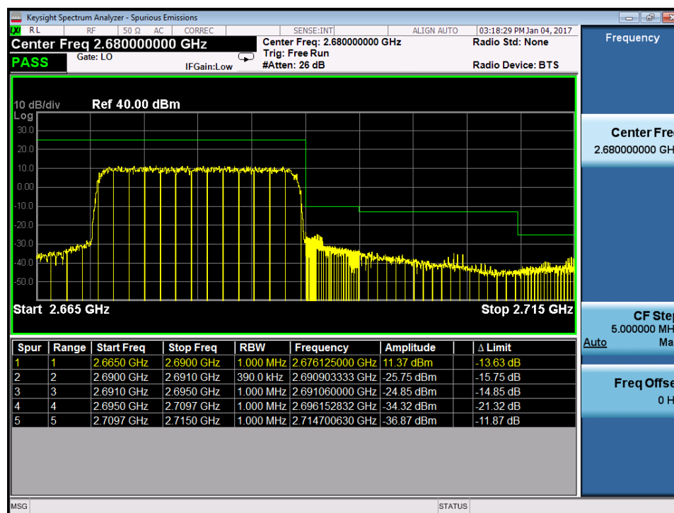
Plot 7-215. Upper ACP Plot (Band 41 – 20.0MHz QPSK – RB Size 100)
