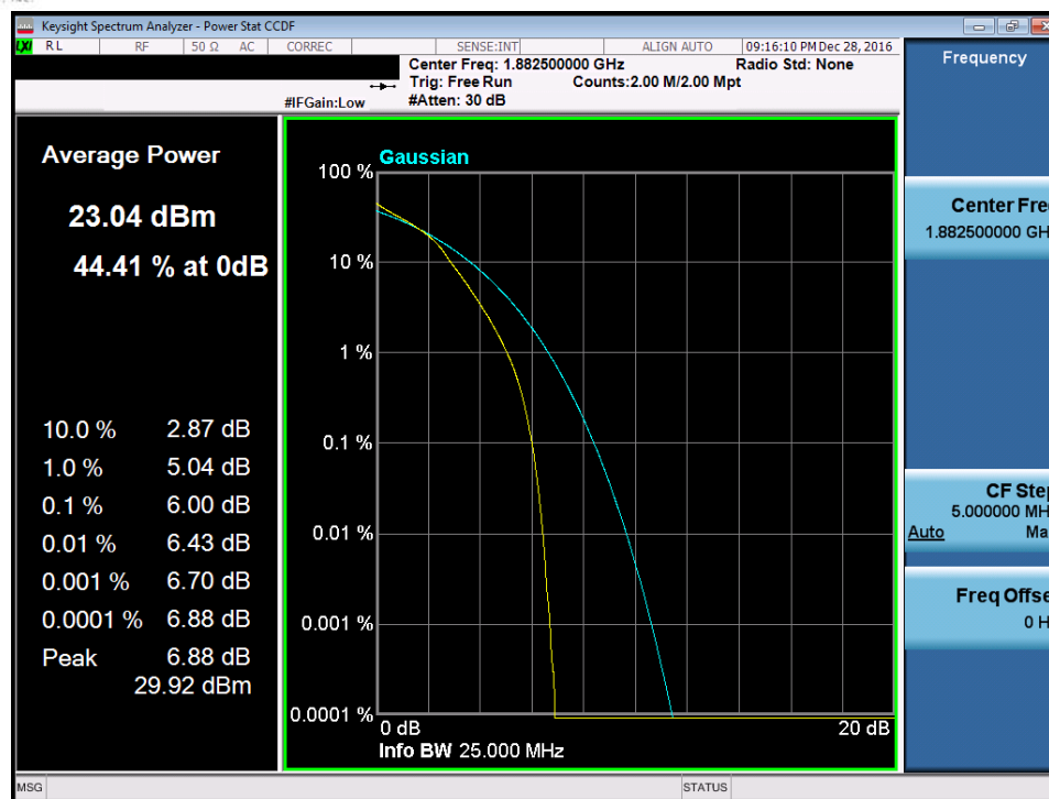
Plot 7-233. PAR Plot (Band 25/2 – 20.0MHz 16-QAM – RB Size 100)
