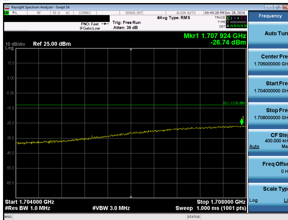
Plot 7-148. Lower Extended Band Edge Plot (Band 4 – 5.0MHz QPSK – RB Size 25)
