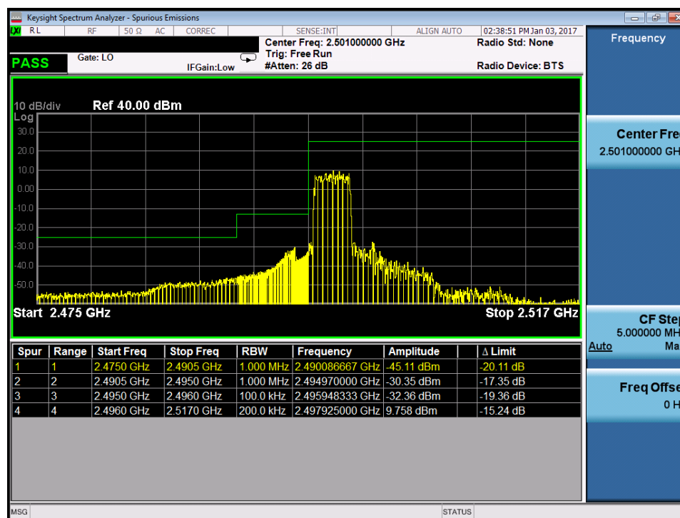
Plot 7-195. Lower ACP Plot with AMPR Reduction (Band 41 – 10.0MHz QPSK – RB Size 15)
