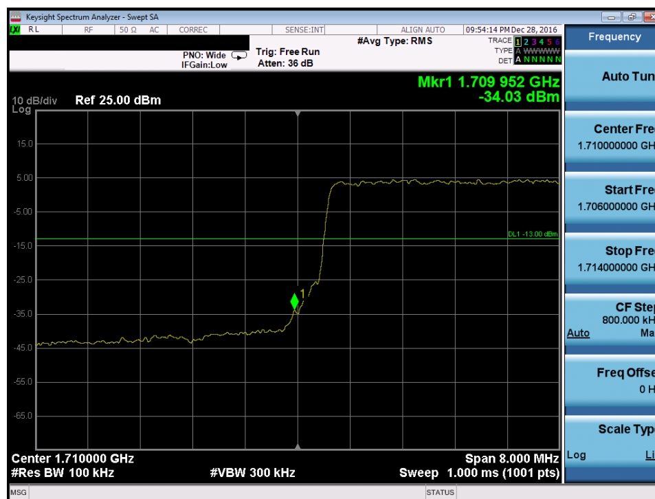
Plot 7-151. Lower Band Edge Plot (Band 4 – 10.0MHz QPSK – RB Size 50)
