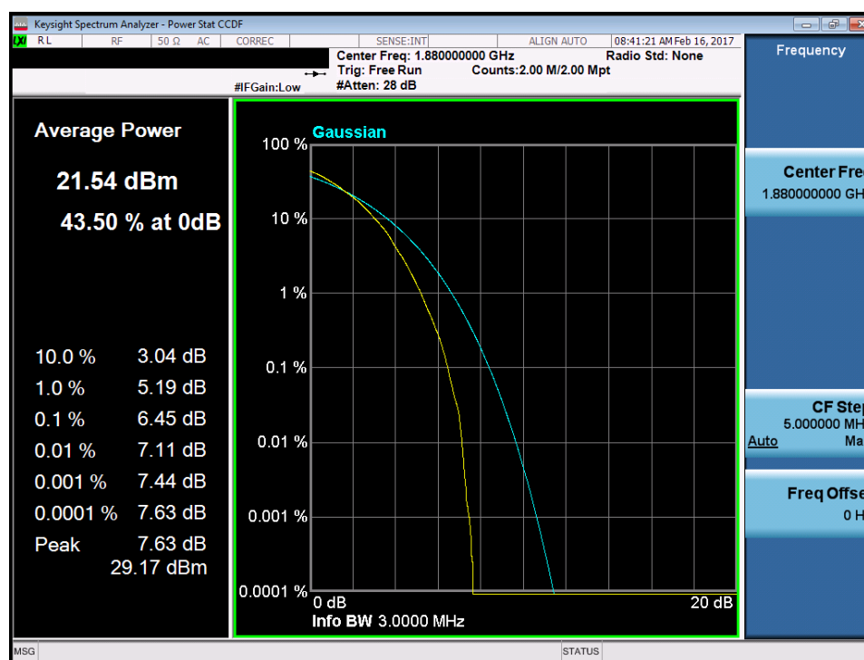
Plot 7-222. PAR Plot (Band 25/2 – 3.0MHz 64-QAM – RB Size 15)
