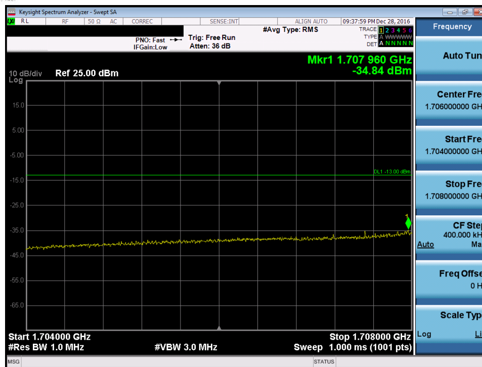
Plot 7-140. Lower Extended Band Edge Plot (Band 4 – 1.4MHz QPSK – RB Size 6)
