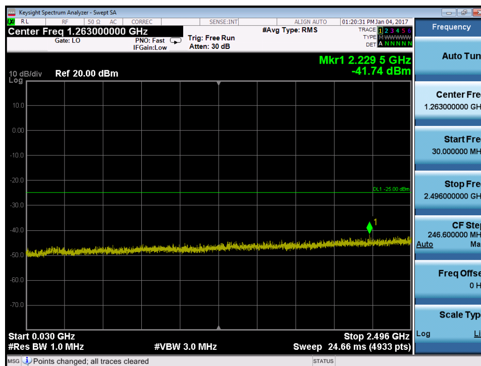
Plot 7-115. Conducted Spurious Plot (Band 41 – 5.0MHz QPSK – RB Size 1, RB Offset 0 – Mid Channel)
