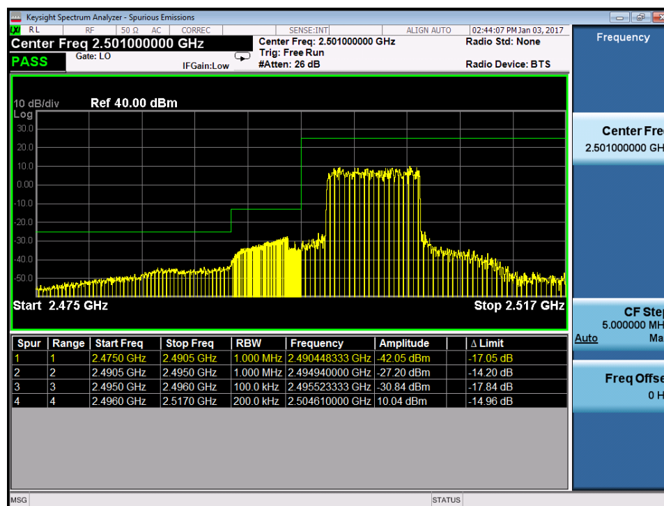
Plot 7-197. Lower ACP Plot with AMPR Reduction (Band 41 – 10.0MHz QPSK – RB Size 41)
