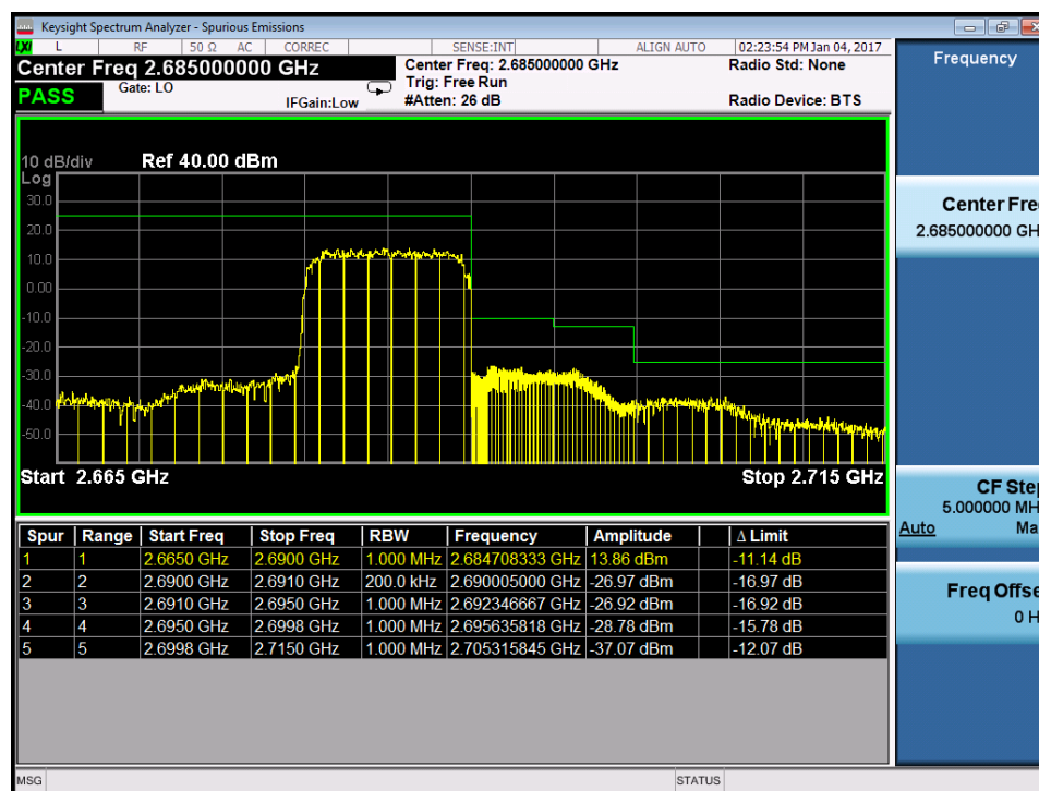
Plot 7-199. Upper ACP Plot (Band 41 – 10.0MHz QPSK – RB Size 50)
