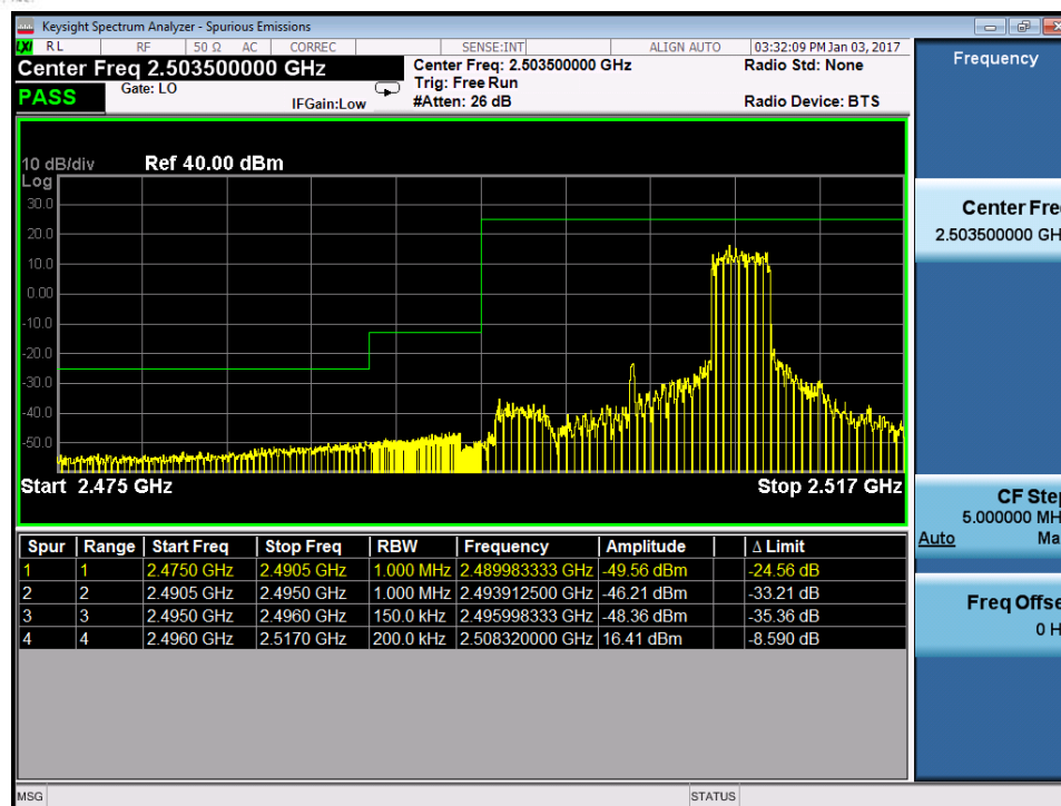
Plot 7-202. Lower ACP Plot with AMPR Reduction (Band 41 – 15.0MHz QPSK – RB Size 15)
