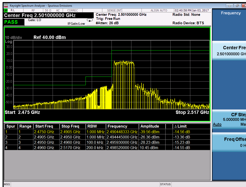
Plot 7-196. Lower ACP Plot (Band 41 – 10.0MHz QPSK – RB Size 24)
