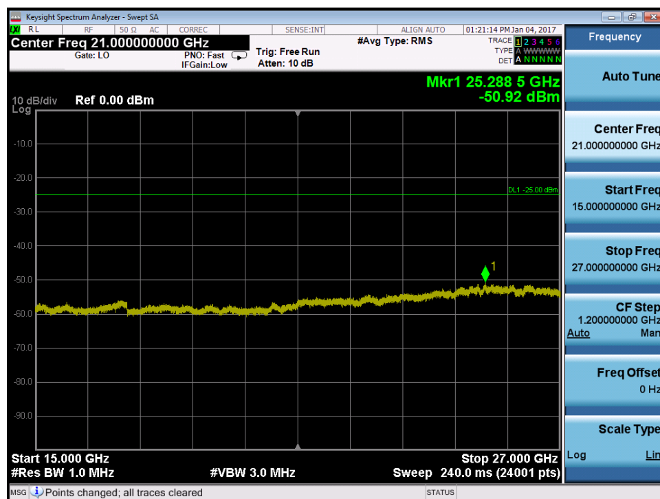
Plot 7-117. Conducted Spurious Plot (Band 41 – 5.0MHz QPSK – RB Size 1, RB Offset 0 – Mid Channel)
