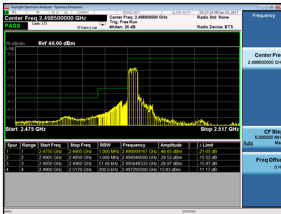
Plot 7-188. Lower ACP Plot with AMPR Reduction (Band 41 – 5.0MHz QPSK – RB Size 9)
