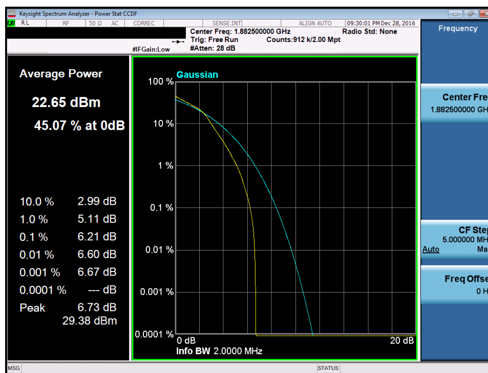
Plot 7-218. PAR Plot (Band 25/2 – 1.4MHz 16-QAM – RB Size 6)
