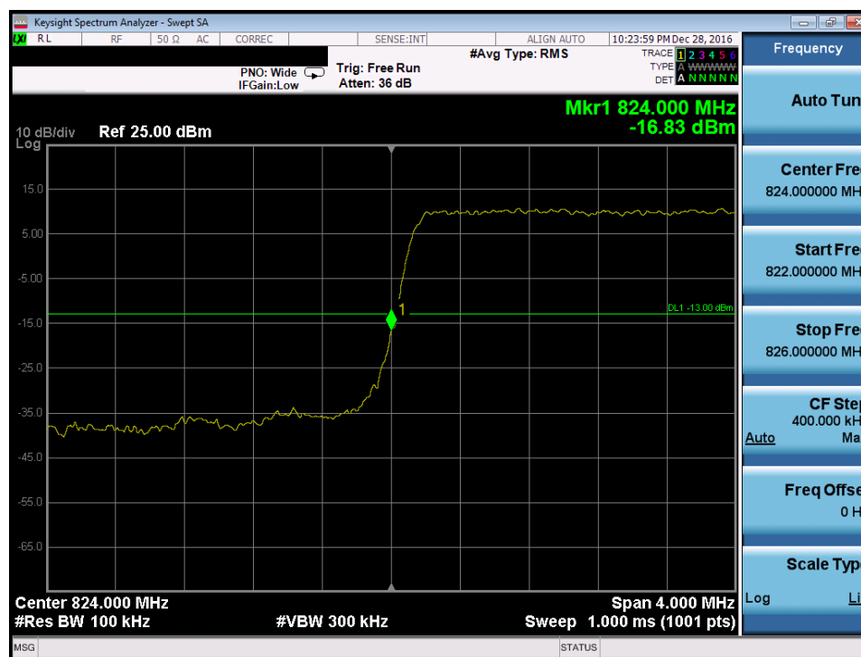
Plot 7-131. Lower Band Edge Plot (Band 26/5 - 3.0MHz QPSK - RB Size 15)
