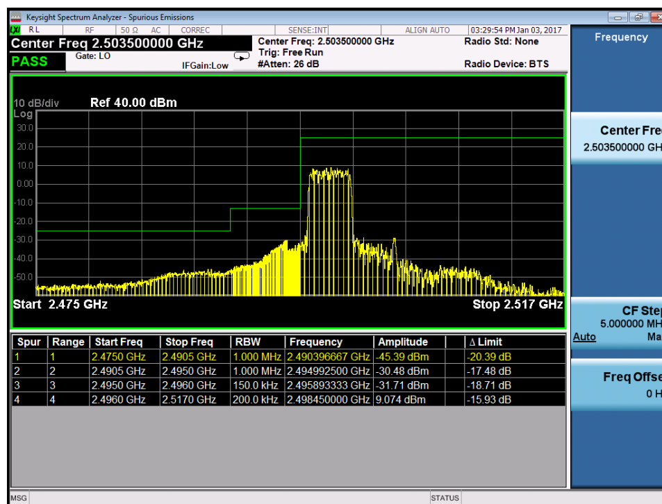
Plot 7-203. Lower ACP Plot with AMPR Reduction (Band 41 – 15.0MHz QPSK – RB Size 18)
