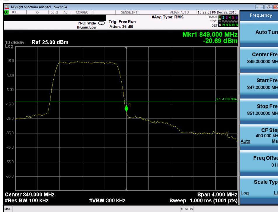
Plot 7-130. Upper Band Edge Plot (Band 26/5 - 1.4MHz QPSK - RB Size 6)
