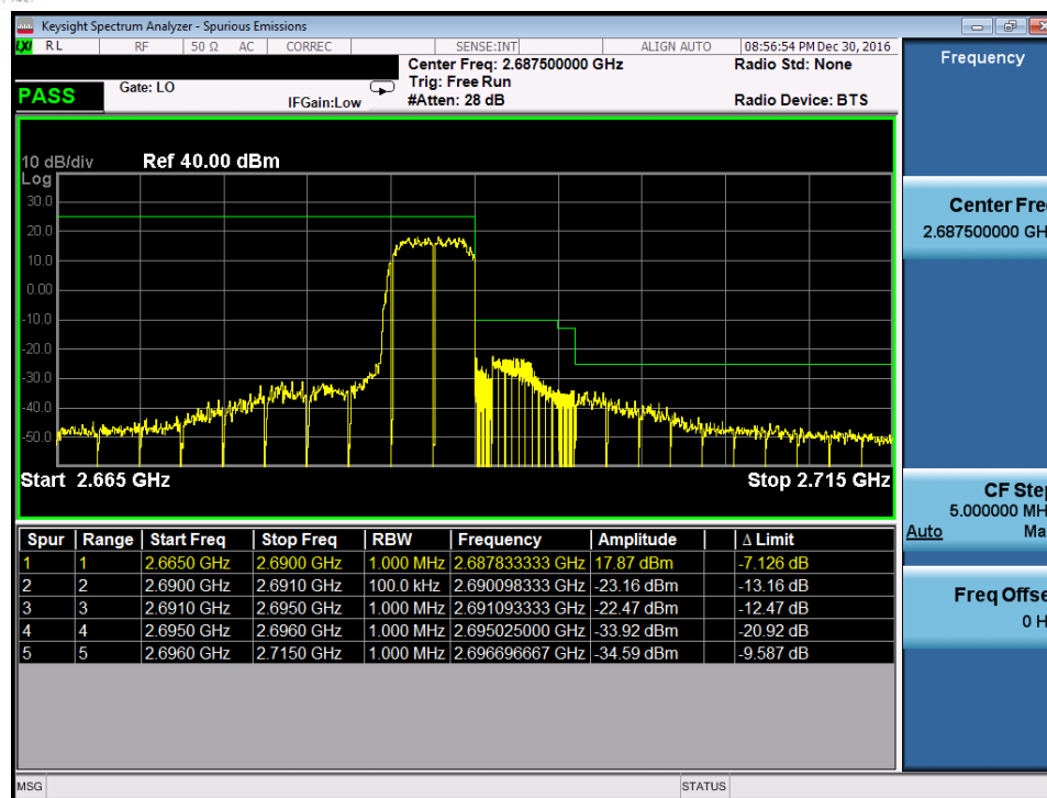
Plot 7-192. Upper ACP Plot with AMPR Reduction (Band 41 – 5.0MHz QPSK – RB Size 25)
