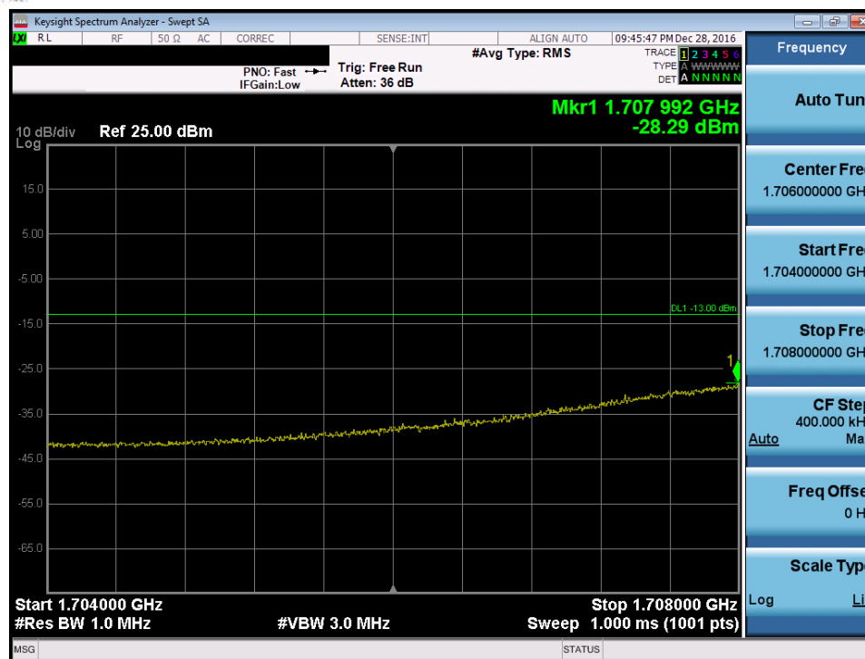
Plot 7-144. Lower Extended Band Edge Plot (Band 4 – 3.0MHz QPSK – RB Size 15)
