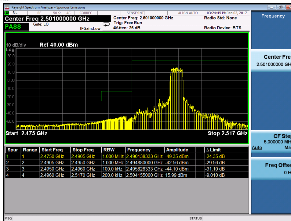
Plot 7-194. Lower ACP Plot with AMPR Reduction (Band 41 – 10.0MHz QPSK – RB Size 12)
