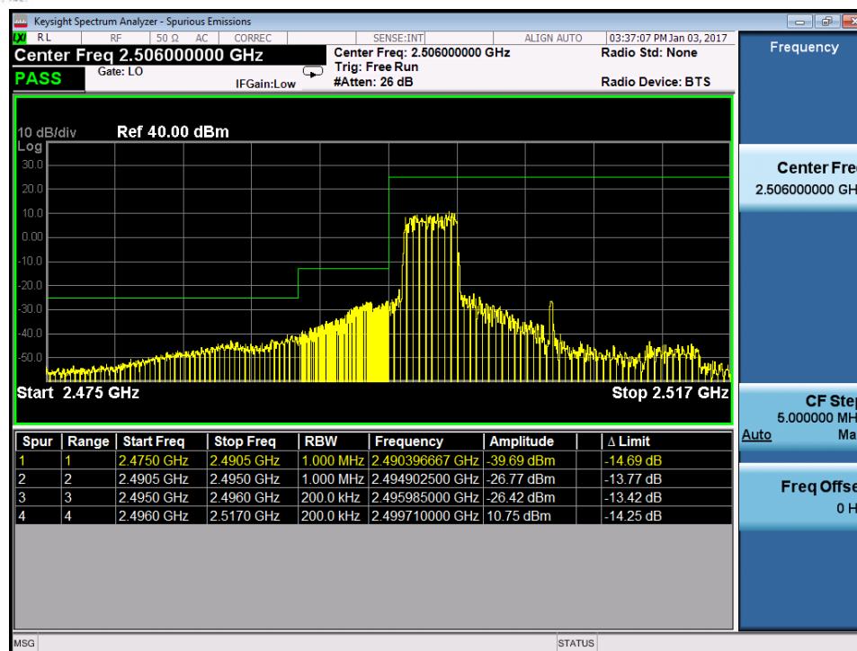
Plot 7-210. Lower ACP Plot with AMPR Reduction (Band 41 – 20.0MHz QPSK – RB Size 18)
