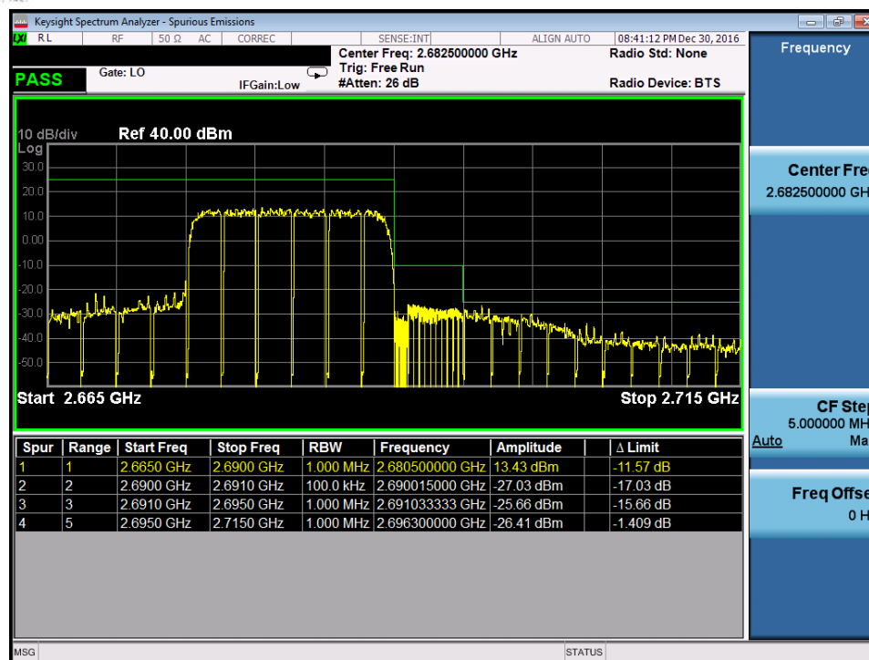
Plot 7-208. Upper ACP Plot with AMPR Reduction (Band 41 – 15.0MHz QPSK – RB Size 75)
