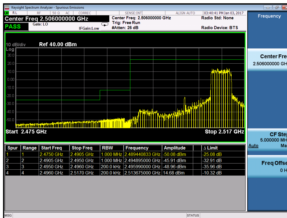
Plot 7-211. Lower ACP Plot with AMPR Reduction (Band 41 – 20.0MHz QPSK – RB Size 20)
