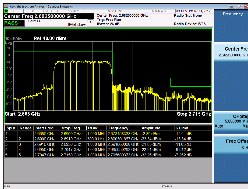
Plot 7-207. Upper ACP Plot (Band 41 – 15.0MHz QPSK – RB Size 75)
