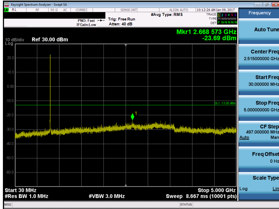
Plot 7-24. Conducted Spurious Plot LTE B26 (5MHz QPSK – RB Size 1, RB Offset 0 – High Channel)
