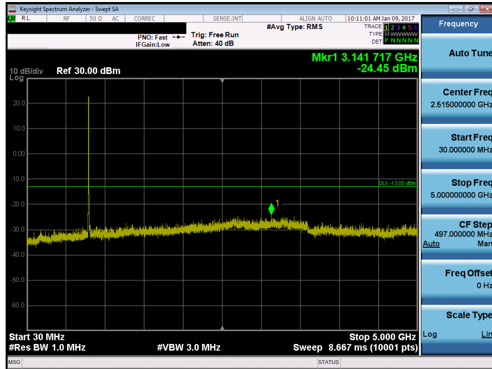
Plot 7-22. Conducted Spurious Plot LTE B26 LTE B26 (5MHz QPSK – RB Size 1, RB Offset 0 – Low Channel)
