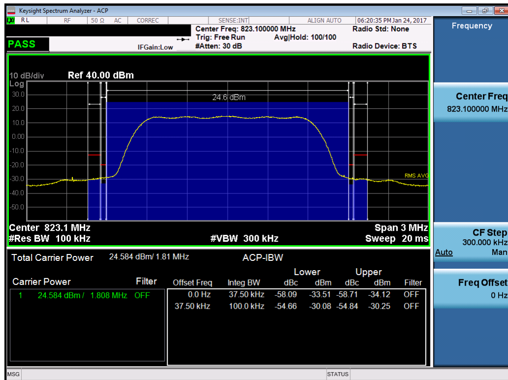
Plot 7-27. Channel Edge Plot CDMA (Ch. 684)
