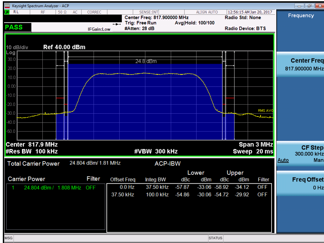
Plot 7-26. Channel Edge Plot CDMA (Ch. 476)
