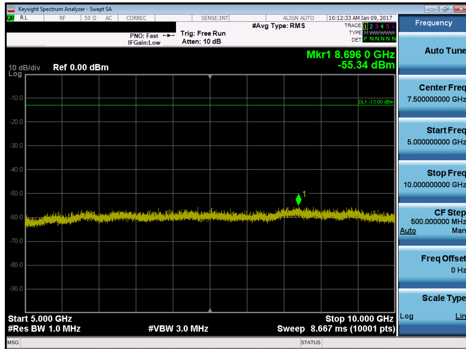
Plot 7-25. Conducted Spurious Plot LTE B26 (5MHz QPSK – RB Size 1, RB Offset 0 – High Channel)
