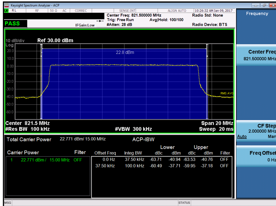
Plot 7-35. Channel Edge Plot LTE B26 (15MHz QPSK – RB Size 75)
