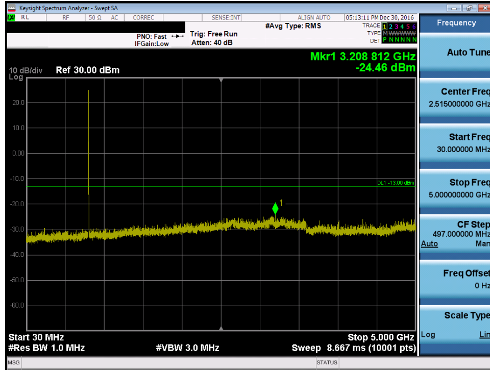
Plot 7-20. Conducted Spurious Plot LTE B26 CDMA (Ch. 684)
