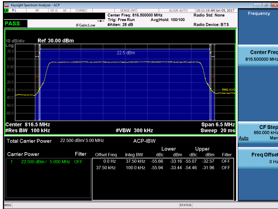
Plot 7-32. Channel Edge Plot LTE B26 (5MHz QPSK – RB Size 25– Low Channel)
