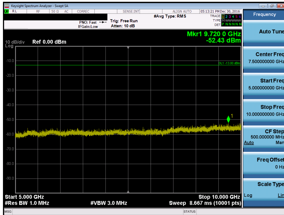
Plot 7-21. Conducted Spurious Plot LTE B26 CDMA (Ch. 684)
