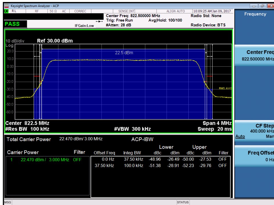
Plot 7-31. Channel Edge Plot LTE B26 (3MHz QPSK - RB Size 15 - High Channel)
