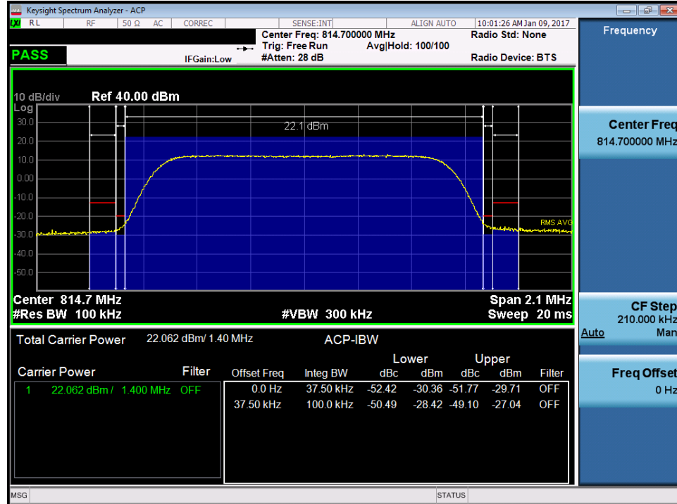
Plot 7-28. Channel Edge Plot LTE B26 (1.4MHz QPSK – RB Size 6– Low Channel)
