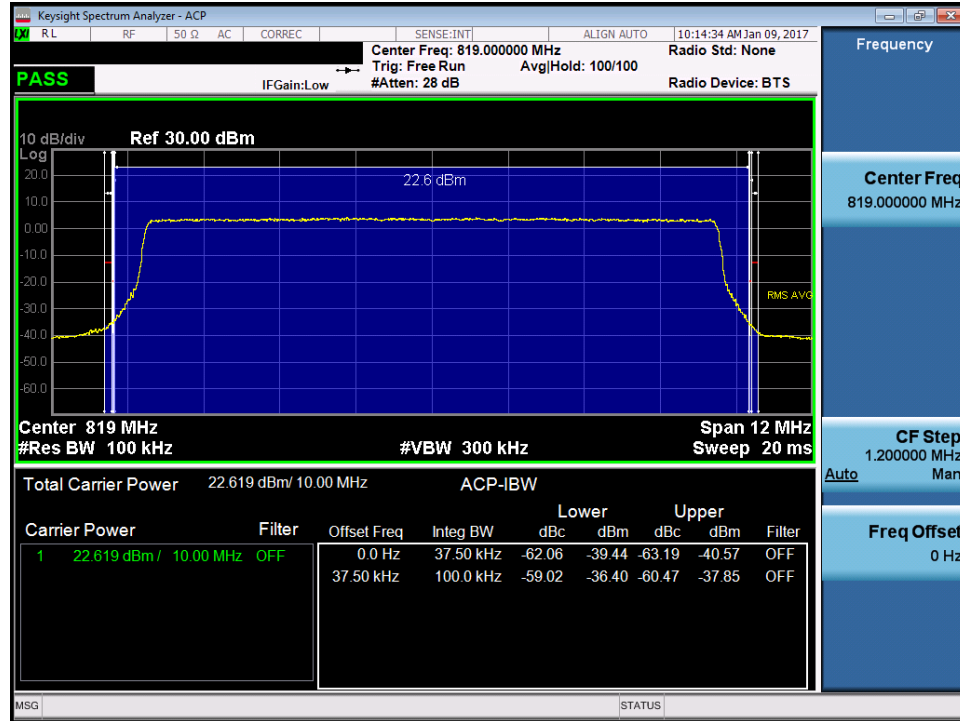
Plot 7-34. Channel Edge Plot LTE B26 (10MHz QPSK – RB Size 50)
