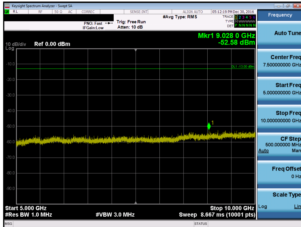
Plot 7-19. Conducted Spurious Plot LTE B26 CDMA (Ch. 476)
