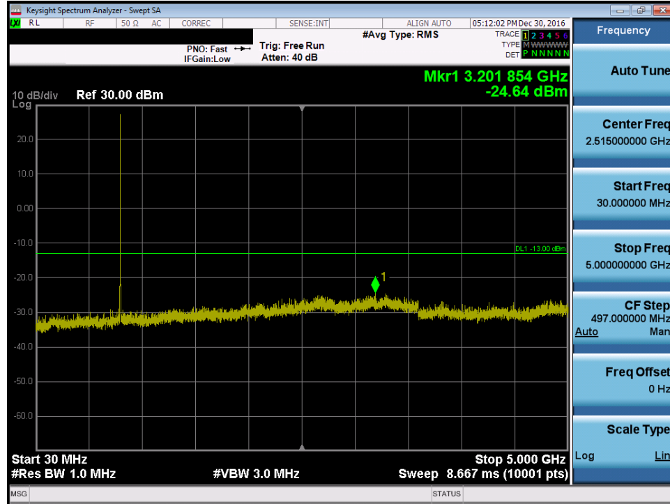
Plot 7-18. Conducted Spurious Plot LTE B26 CDMA (Ch. 476)
