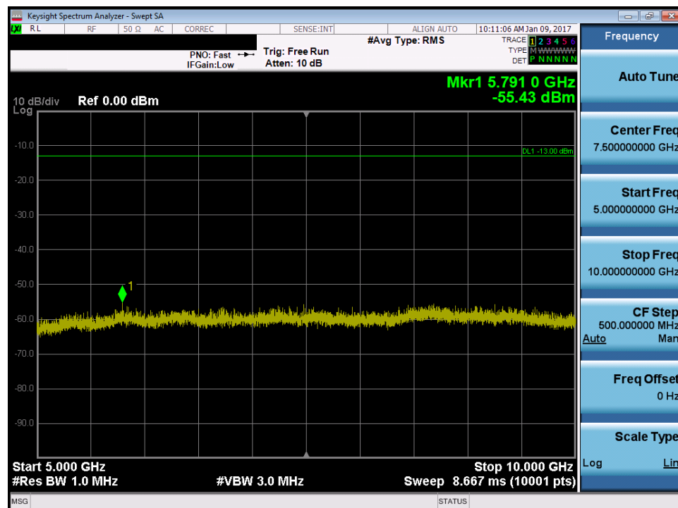
Plot 7-23. Conducted Spurious Plot LTE B26 (5MHz QPSK – RB Size 1, RB Offset 0 – Low Channel)
