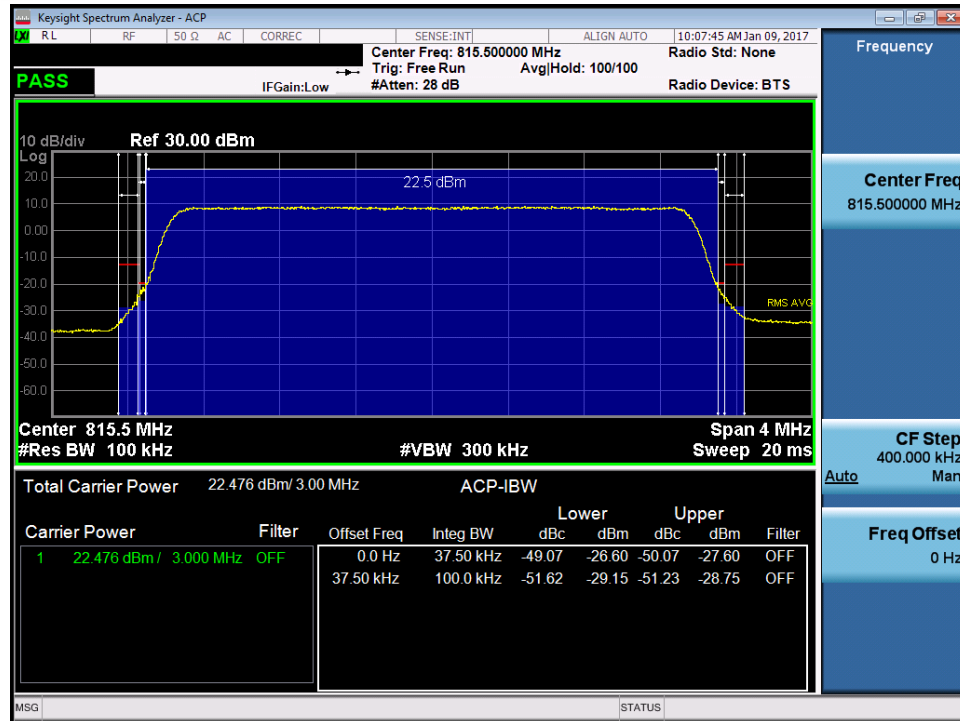
Plot 7-30. Channel Edge Plot LTE B26 (3MHz QPSK - RB Size 15- Low Channel)
