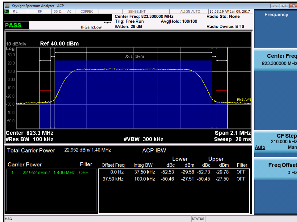
Plot 7-29. Channel Edge Plot LTE B26 (1.4MHz QPSK – RB Size 6 – High Channel)
