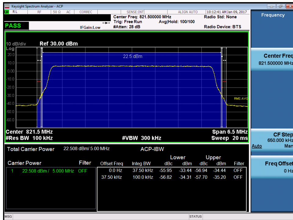
Plot 7-33. Channel Edge Plot LTE B26 (5MHz QPSK – RB Size 25 – High Channel)
