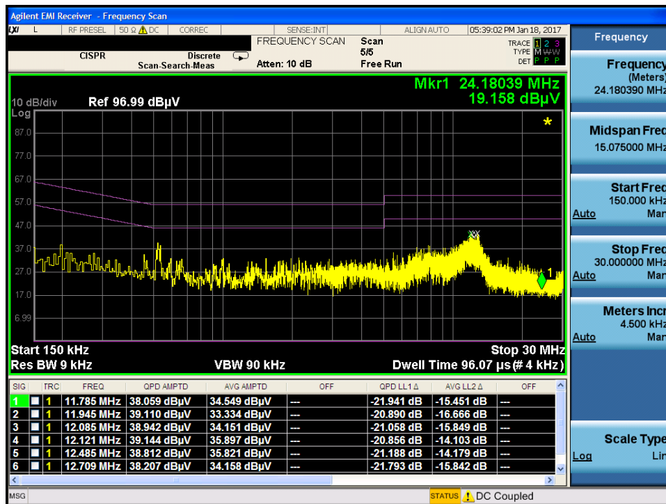
Plot 8-4. Line-Conducted Test Plot with Antenna Terminated in (N)
