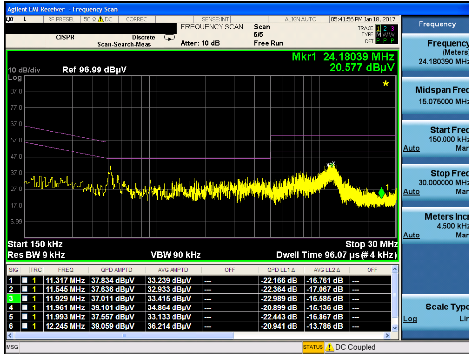
Plot 8-3. Line-Conducted Test Plot with Antenna Terminated in 50Ω (L1)
