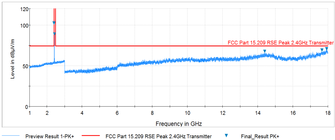
Plot 7-42. Radiated Spurious Plot above 1GHz (BT – Ch. 0, Ant. Pol. H)
