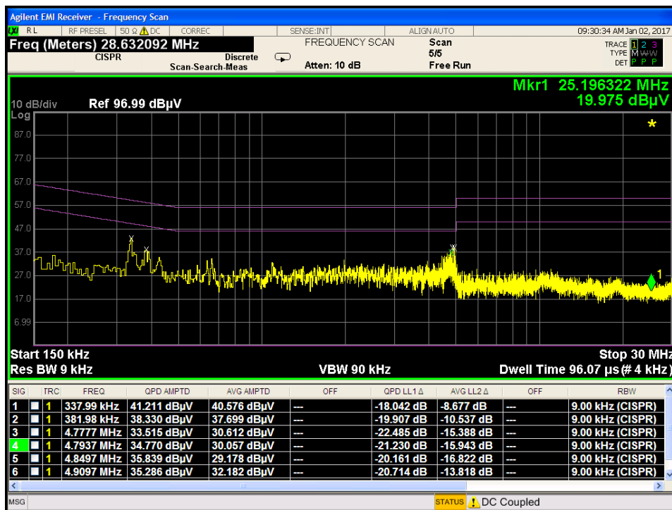
Plot 7-273. Line Conducted Plot with 802.11a UNII Band 3 (N)
