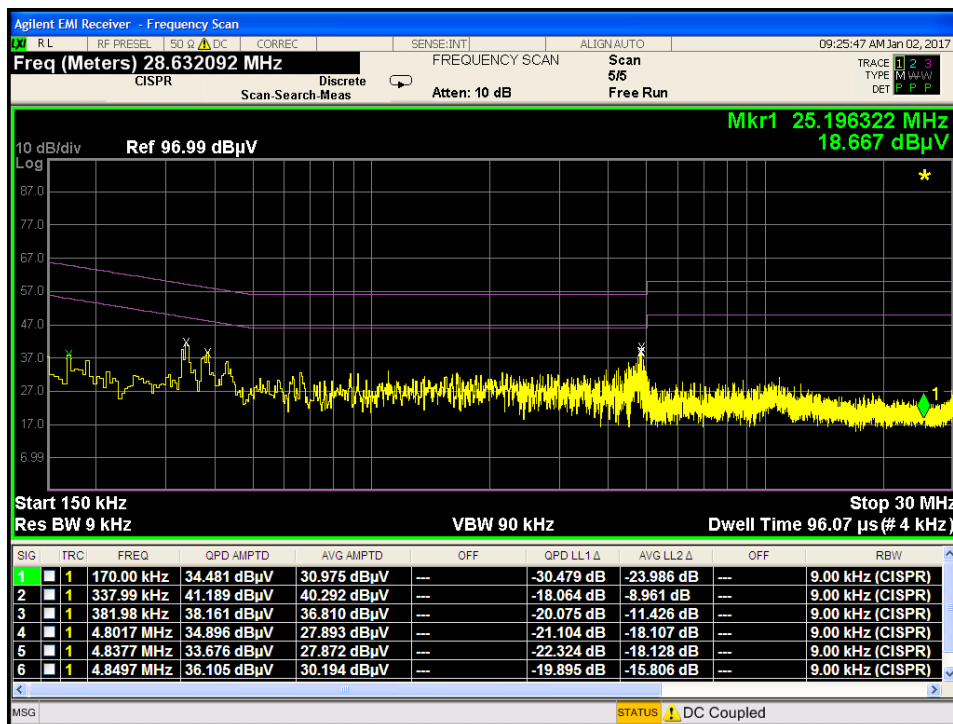
Plot 7-271. Line Conducted Plot with 802.11a UNII Band 2C (N)
