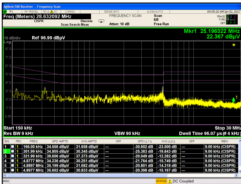
Plot 7-269. Line Conducted Plot with 802.11a UNII Band 2A (N)
