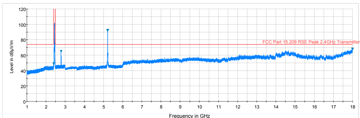
Plot 7-179. Radiated Spurious Plot above 1GHz (5GHz – 2.4 GHz, Ant. Pol. H)
