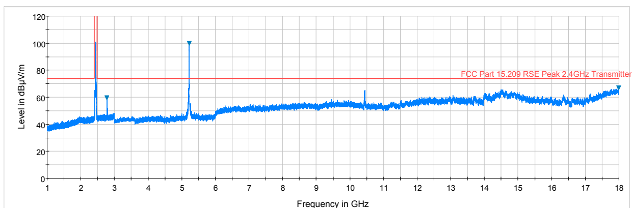
Plot 7-180. Radiated Spurious Plot above 1GHz (5GHz – 2.4 GHz, Ant. Pol. V)
