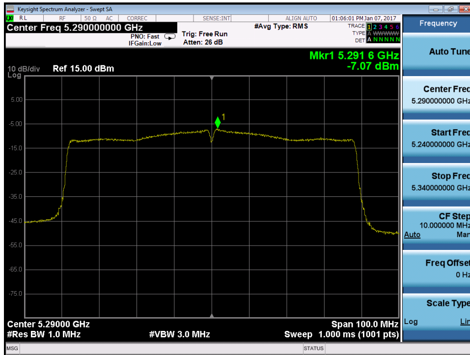
Plot 7-132. Power Spectral Density Plot (80MHz BW 802.11a/n/ac (UNII Band 2A) – Ch. 58)
